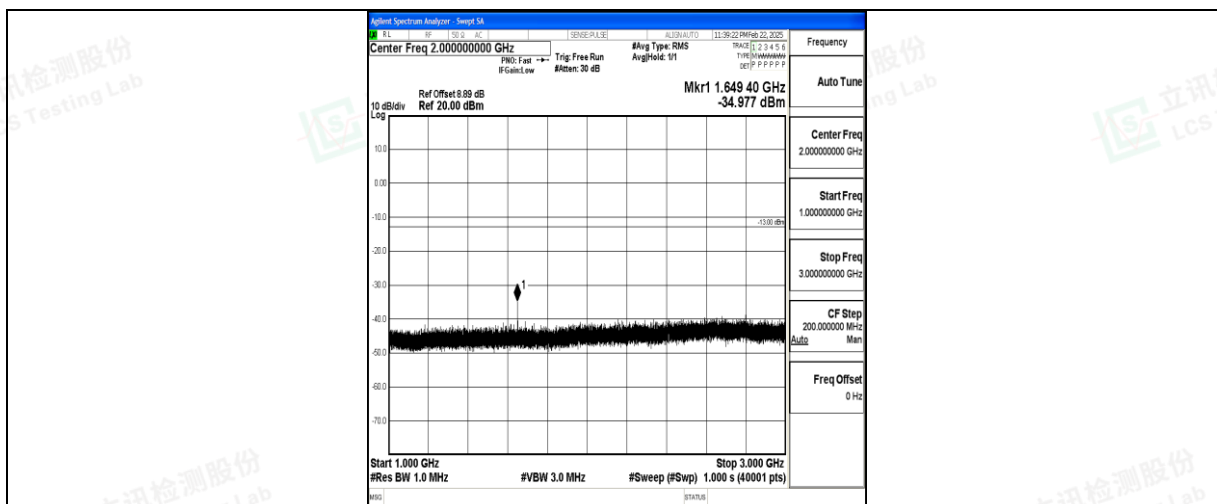
Band5_10MHz_QPSK_20450_1RB#0_1000~3000_1000~3000
