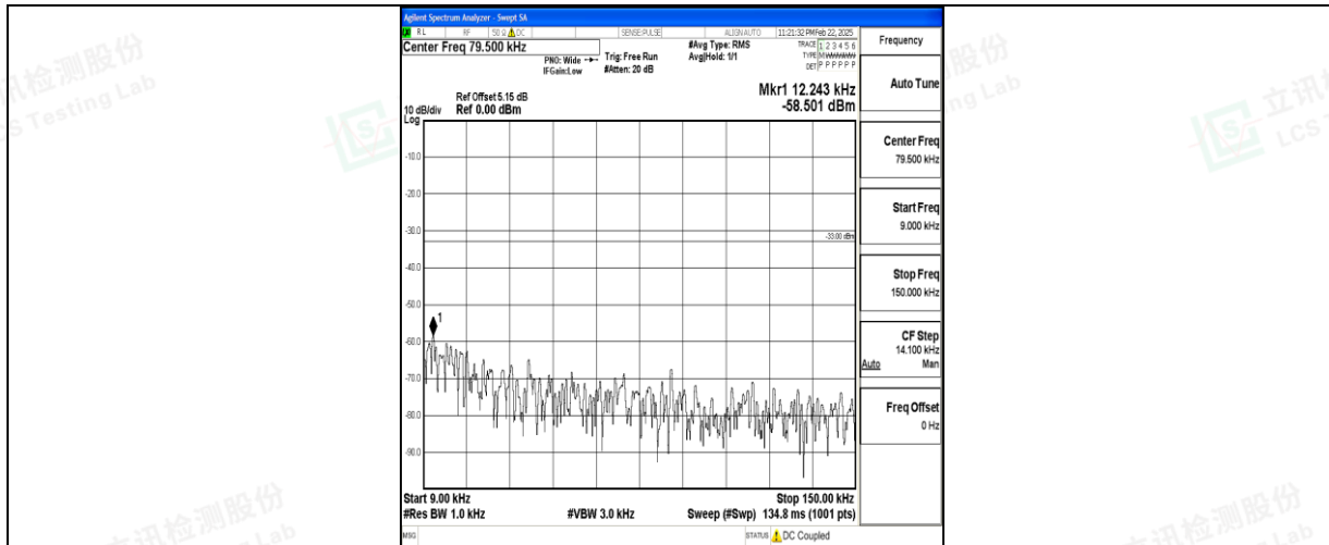
Band5_5MHz_16QAM_20525_1RB#0_0.009~0.15_0.009~0.15
