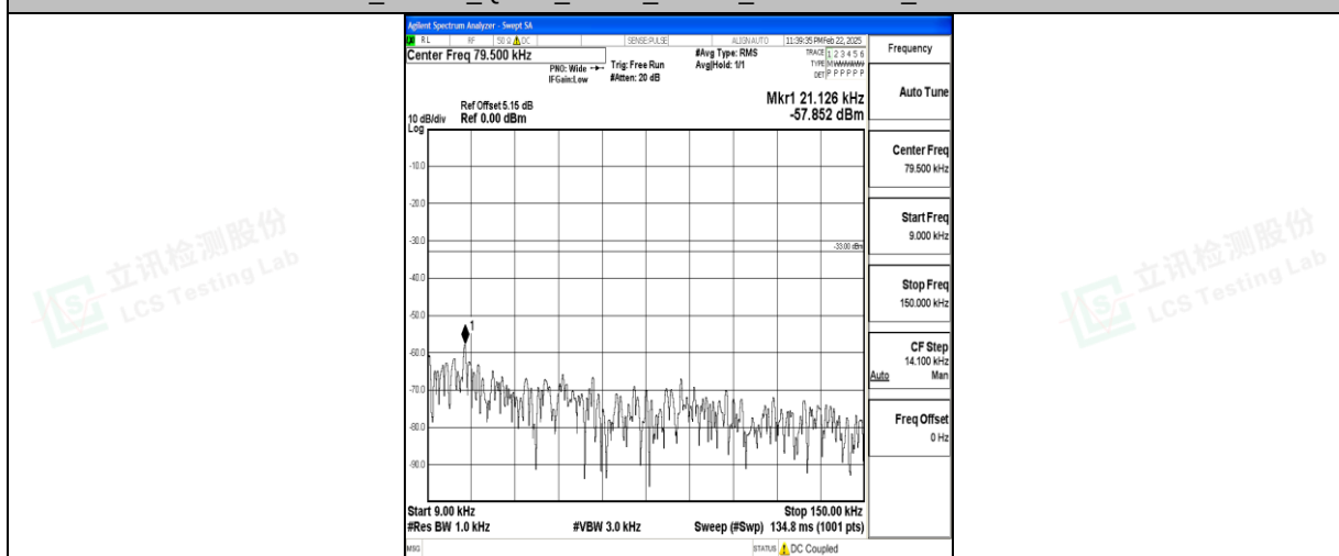
Band5_10MHz_16QAM_20450_1RB#0_0.009~0.15_0.009~0.15
