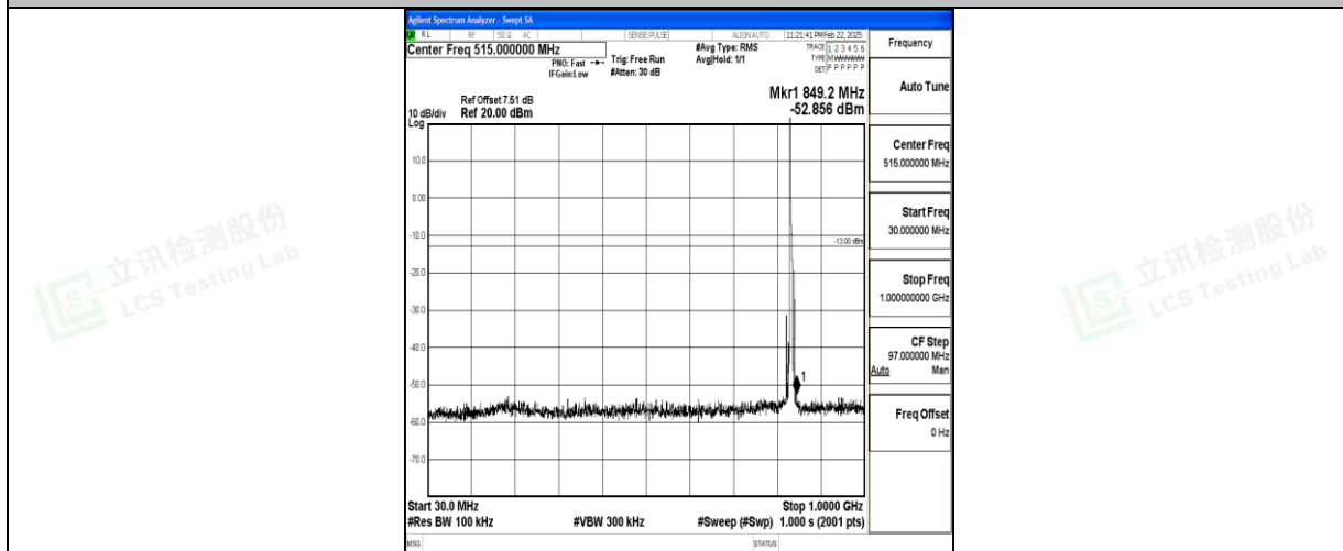
Band5_5MHz_16QAM_20525_1RB#0_30~1000_30~1000
