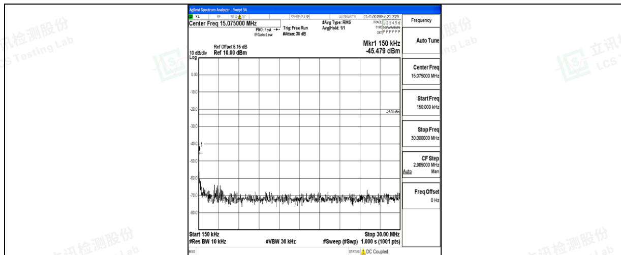
Band5_10MHz_QPSK_20600_1RB#0_0.15~30_0.15~30
