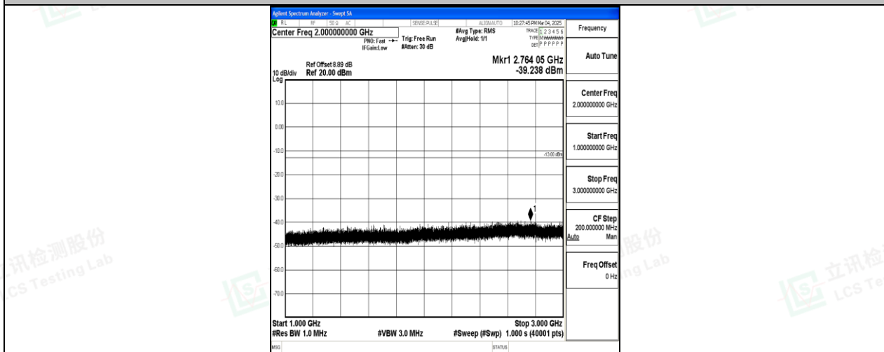
Band12_10MHz_QPSK_23095_1RB#0_1000~3000_1000~3000
