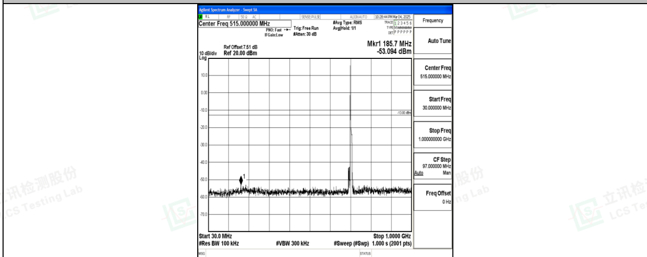
Band12_10MHz_QPSK_23130_1RB#0_30~1000_30~1000
