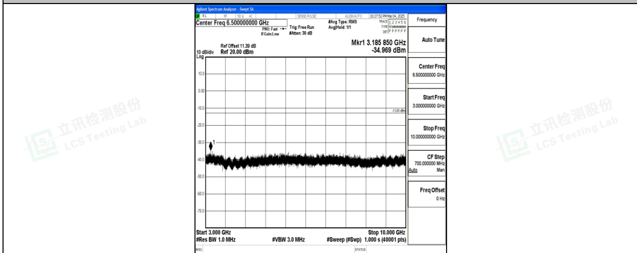
Band12_10MHz_QPSK_23095_1RB#0_3000~10000_3000~10000
