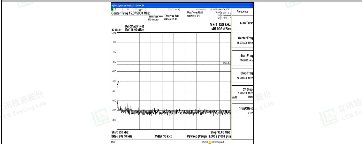
Band17_5MHz_QPSK_23790_1RB#0_0.15~30_0.15~30
