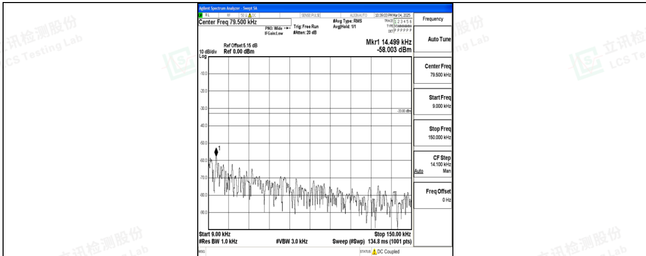
Band17_5MHz_QPSK_23790_1RB#0_0.009~0.15_0.009~0.15
