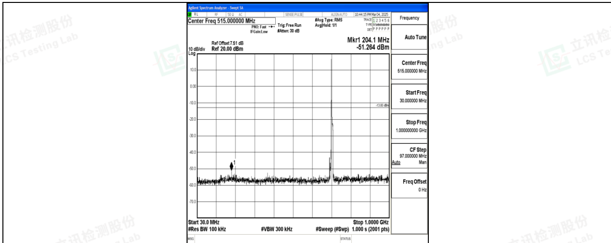
Band17_10MHz_QPSK_23800_1RB#0_30~1000_30~1000
