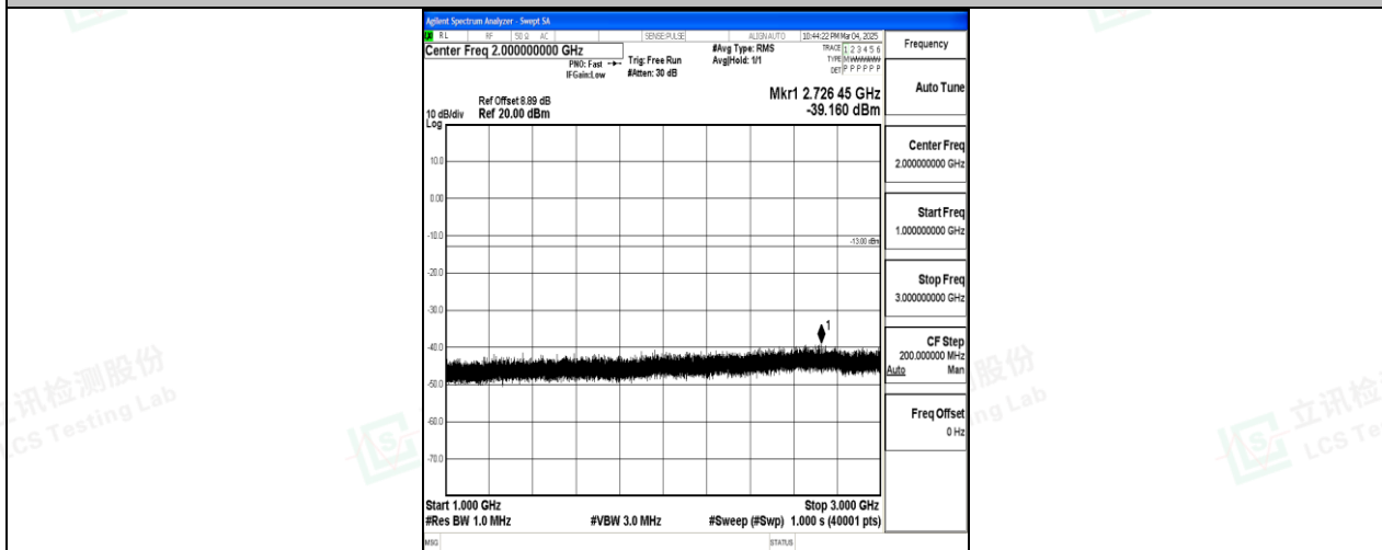
Band17_10MHz_QPSK_23800_1RB#0_1000~3000_1000~3000
