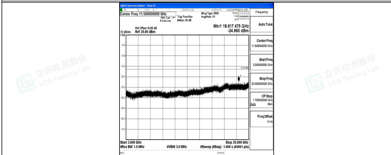
Band25_10MHz_QPSK_26640_1RB#0_3000~20000_3000~20000
