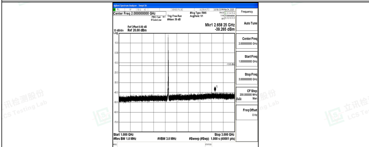
Band25_5MHz_16QAM_26065_1RB#0_1000~3000_1000~3000
