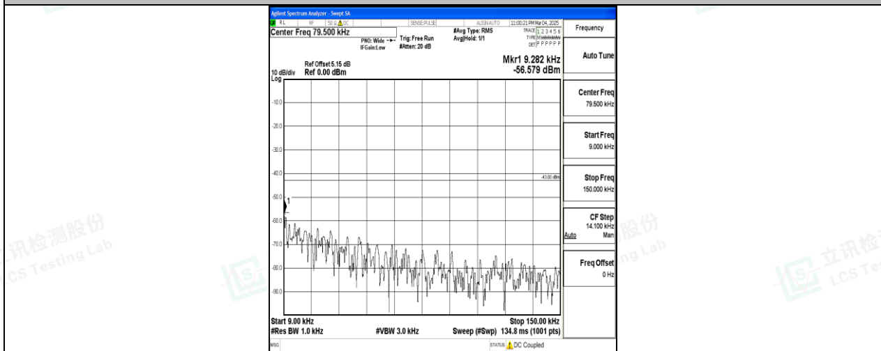
Band25_10MHz_16QAM_26090_1RB#0_0.009~0.15_0.009~0.15
