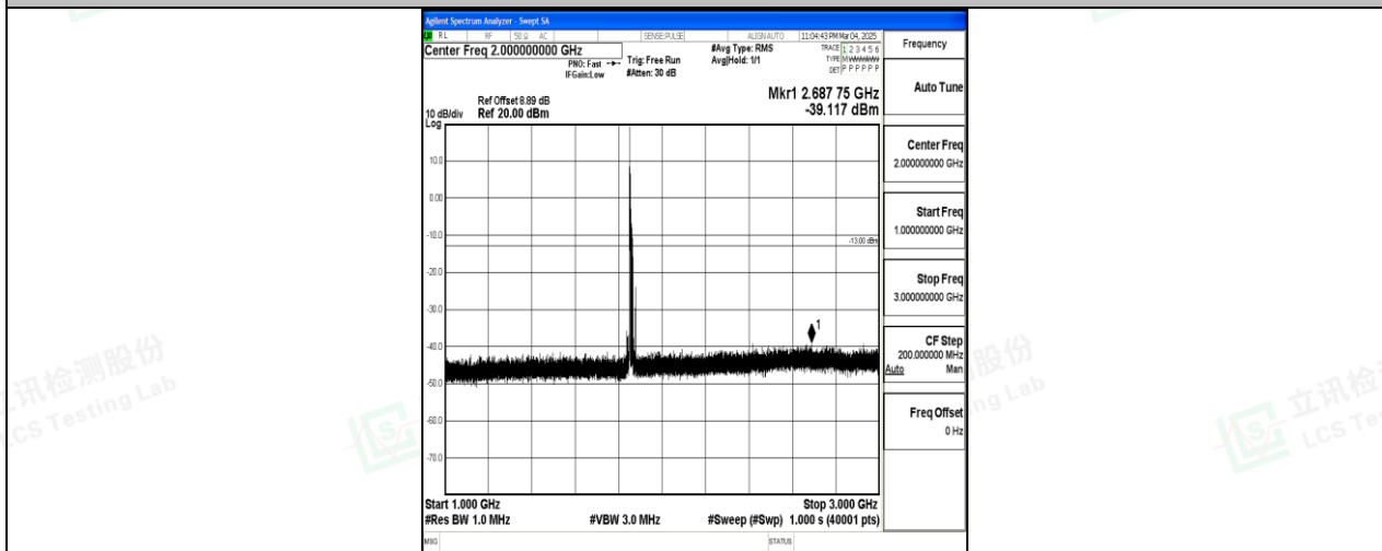
Band25_15MHz_16QAM_26115_1RB#0_1000~3000_1000~3000
