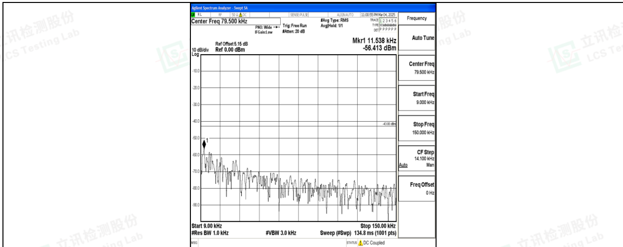
Band25_10MHz_QPSK_26365_1RB#0_0.009~0.15_0.009~0.15
