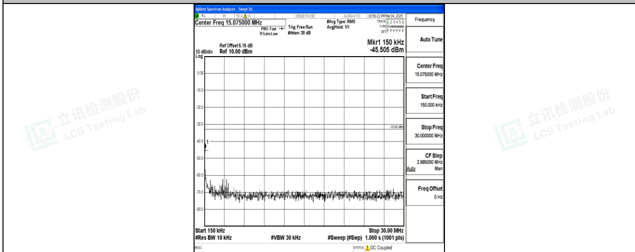
Band25_5MHz_16QAM_26065_1RB#0_0.15~30_0.15~30
