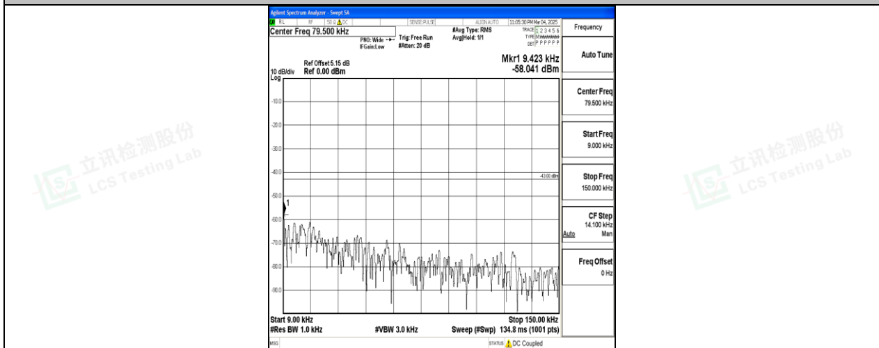
Band25_15MHz_16QAM_26365_1RB#0_0.009~0.15_0.009~0.15
