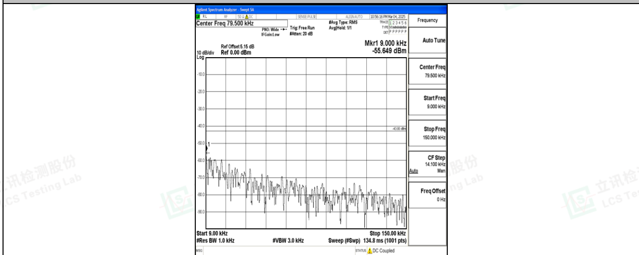
Band25_5MHz_16QAM_26065_1RB#0_0.009~0.15_0.009~0.15
