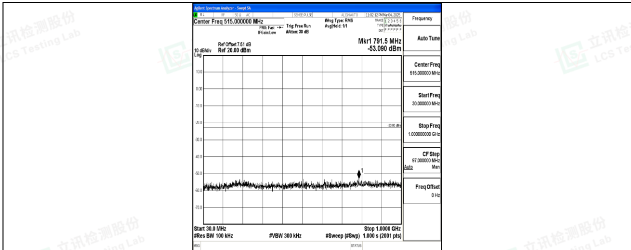
Band25_10MHz_QPSK_26640_1RB#0_30~1000_30~1000
