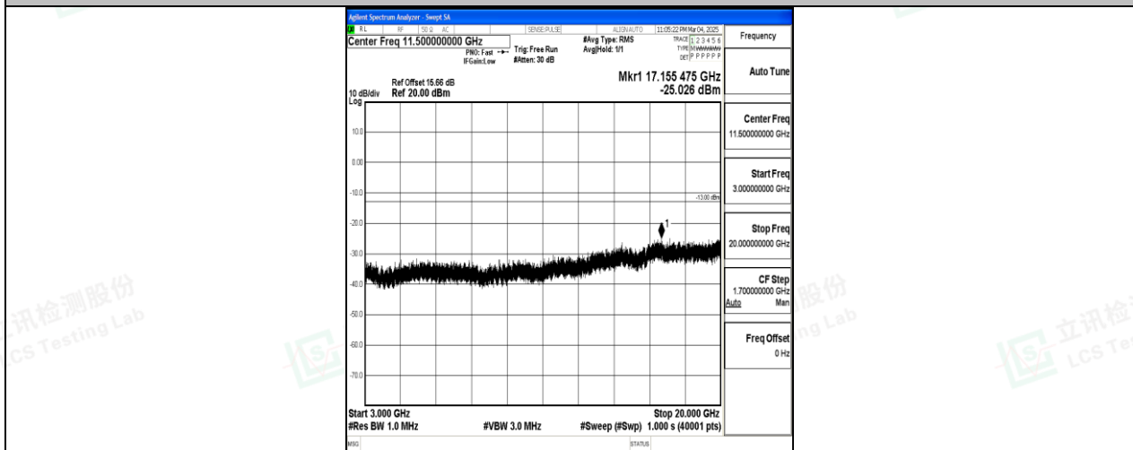
Band25_15MHz_QPSK_26365_1RB#0_3000~20000_3000~20000
