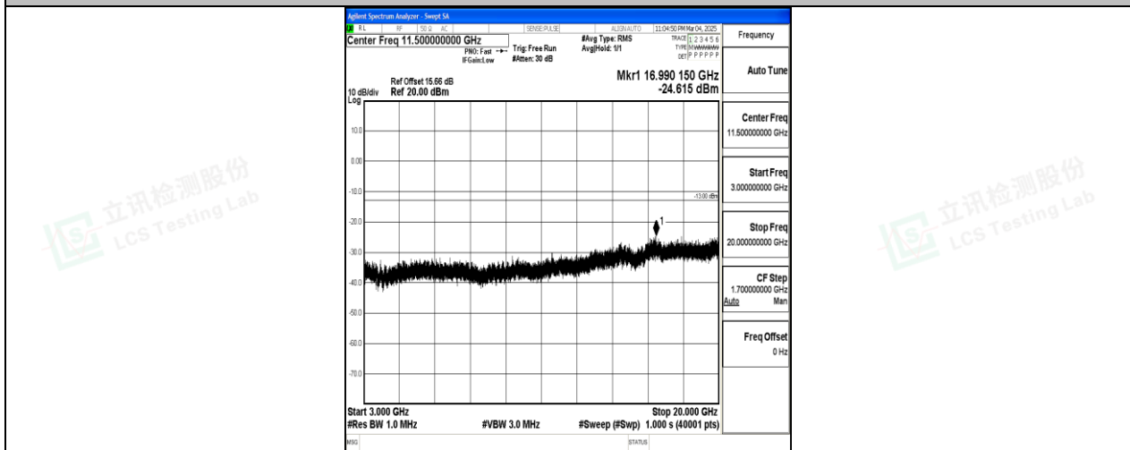
Band25_15MHz_16QAM_26115_1RB#0_3000~20000_3000~20000
