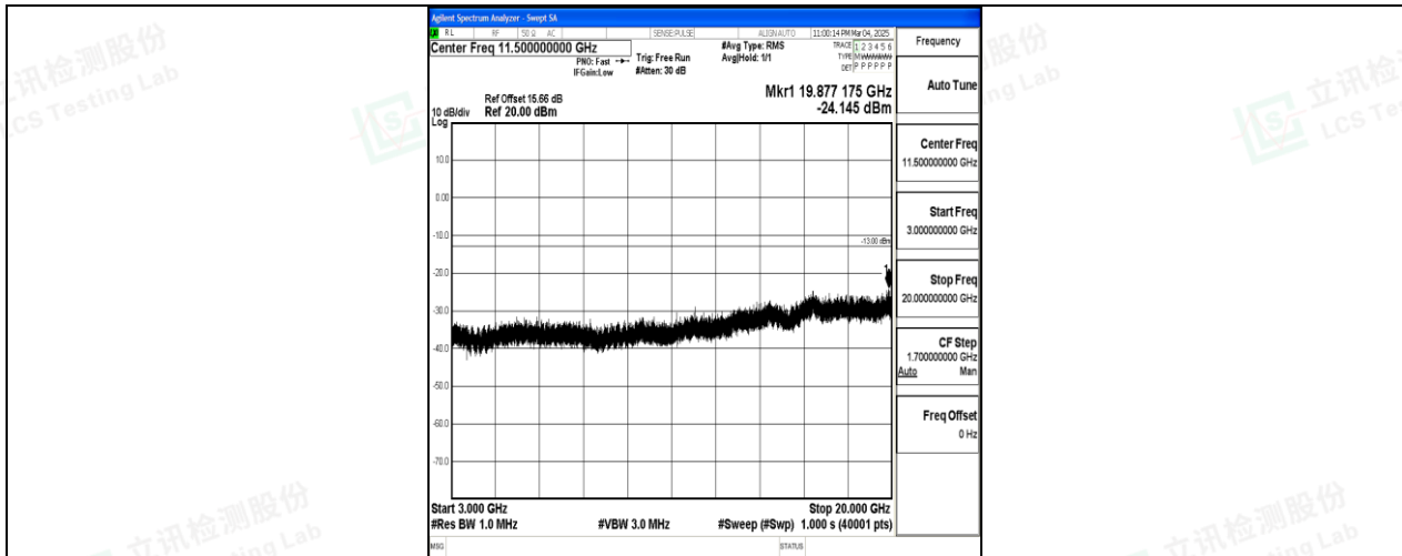
Band25_10MHz_QPSK_26090_1RB#0_3000~20000_3000~20000
