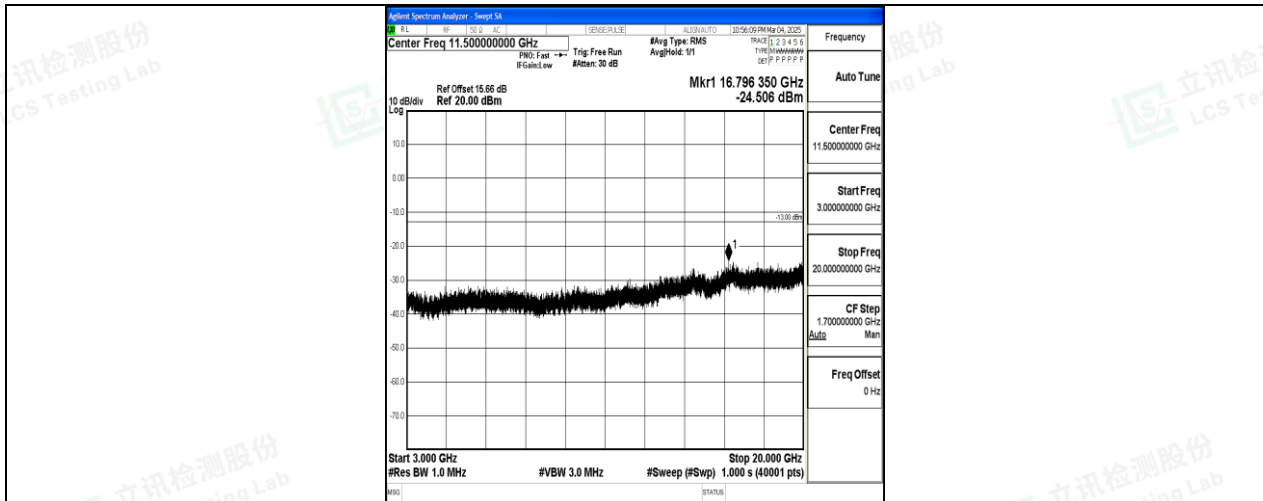
Band25_5MHz_QPSK_26065_1RB#0_3000~20000_3000~20000
