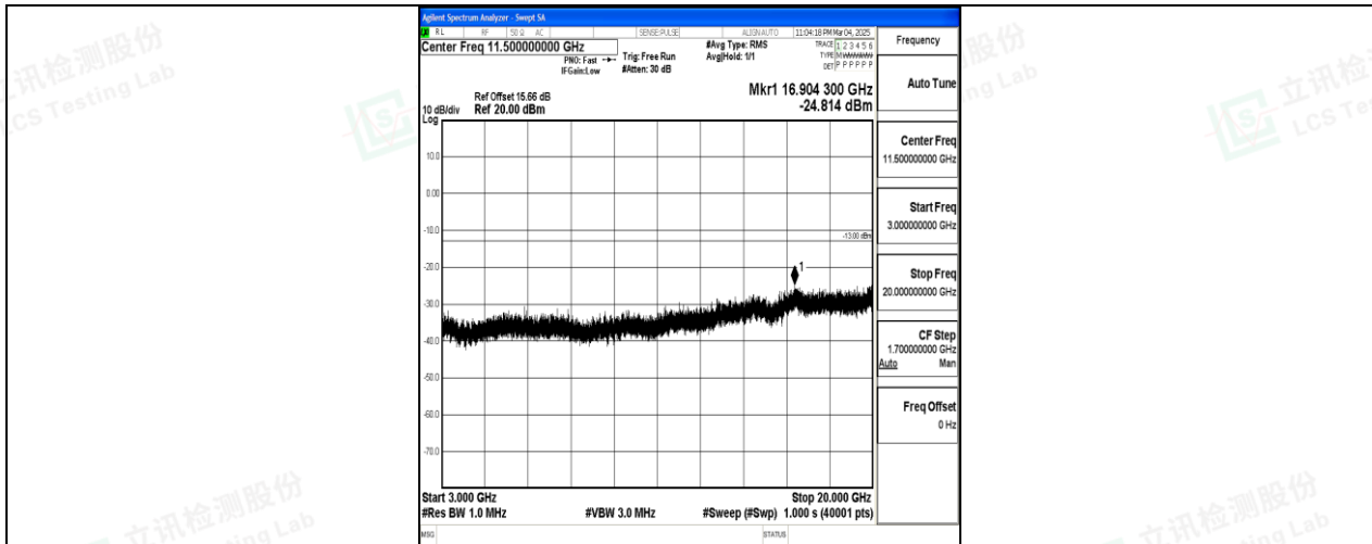
Band25_15MHz_QPSK_26115_1RB#0_3000~20000_3000~20000
