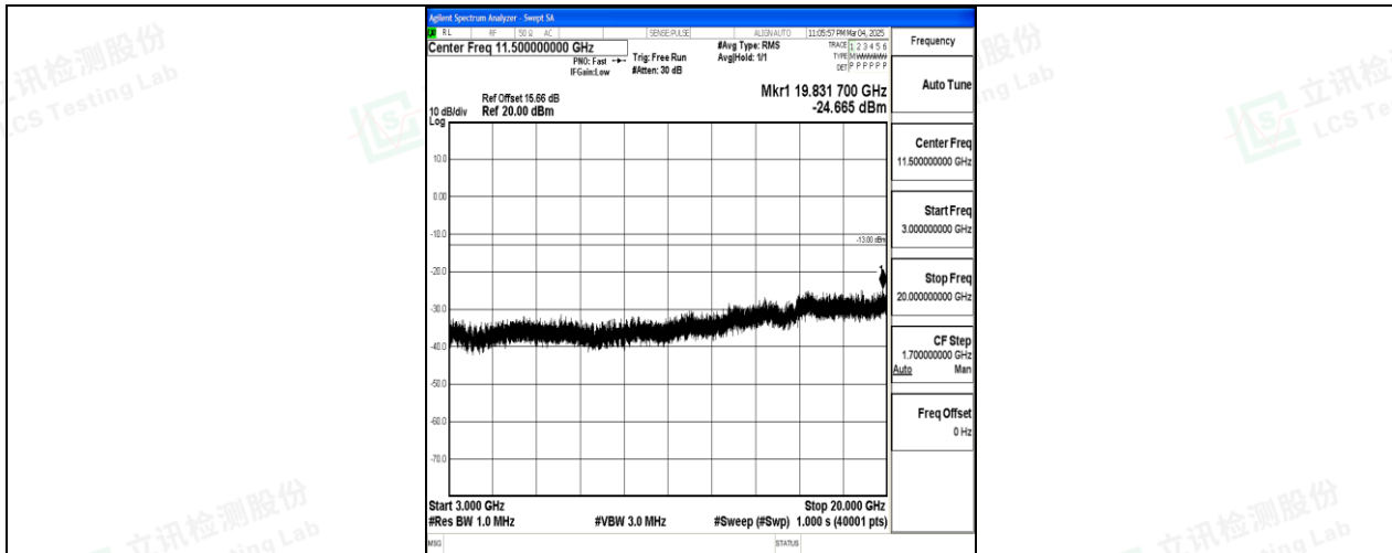
Band25_15MHz_16QAM_26365_1RB#0_3000~20000_3000~20000
