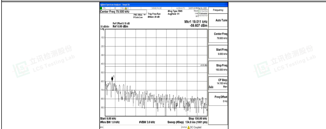
Band25_5MHz_16QAM_26365_1RB#0_0.009~0.15_0.009~0.15
