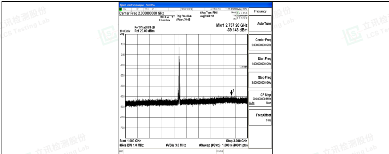
Band25_10MHz_QPSK_26365_1RB#0_1000~3000_1000~3000
