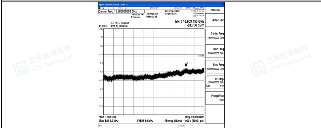
Band25_5MHz_QPSK_26665_1RB#0_3000~20000_3000~20000
