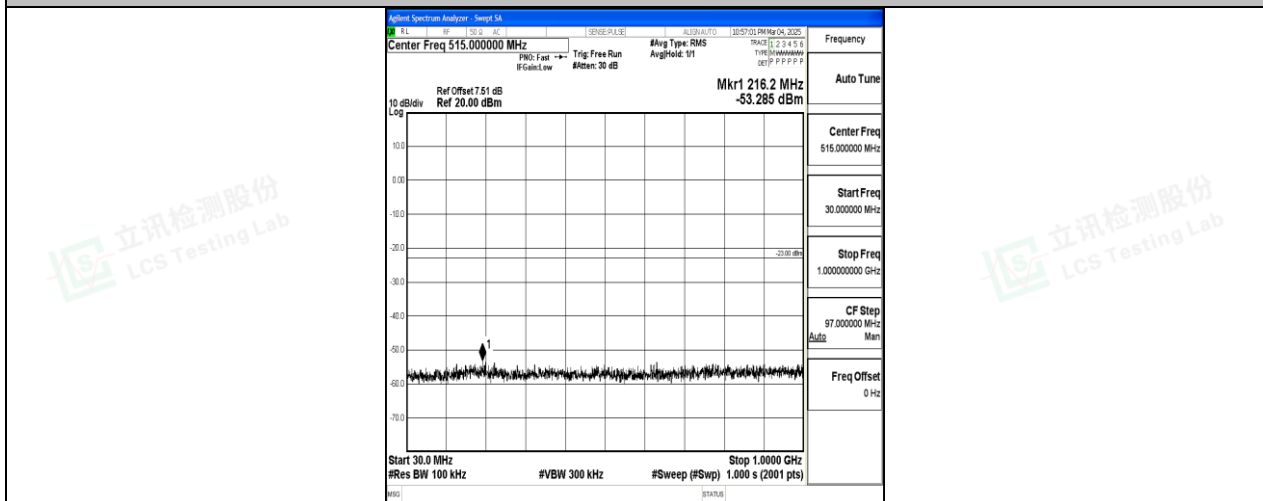
Band25_5MHz_QPSK_26365_1RB#0_30~1000_30~1000
