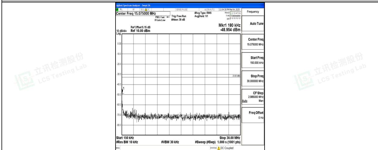
Band25_15MHz_16QAM_26115_1RB#0_0.15~30_0.15~30
