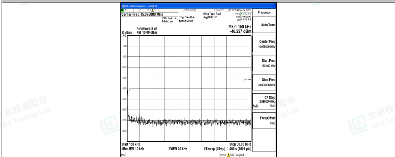
Band25_5MHz_QPSK_26365_1RB#0_0.15~30_0.15~30
