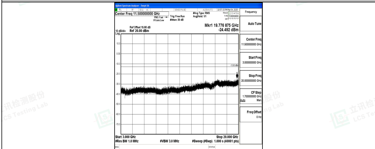
Band25_5MHz_QPSK_26365_1RB#0_3000~20000_3000~20000
