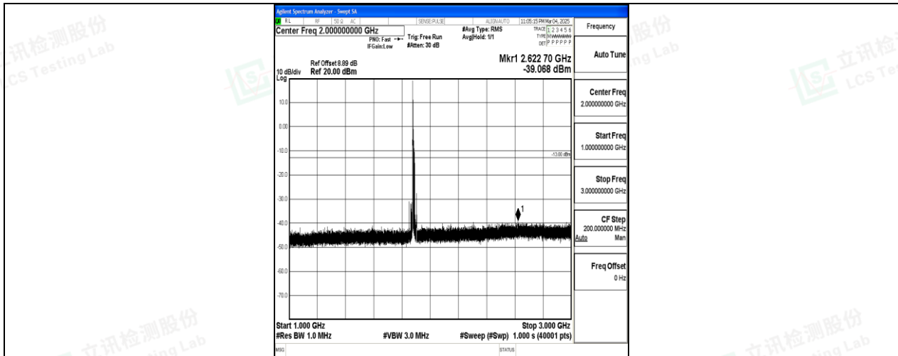
Band25_15MHz_QPSK_26365_1RB#0_1000~3000_1000~3000
