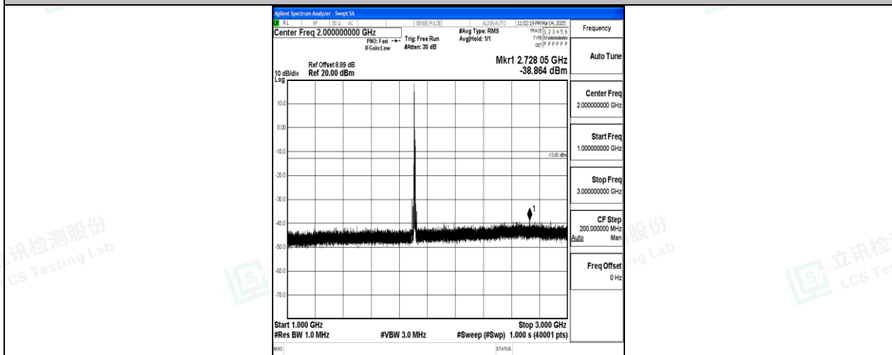
Band25_10MHz_QPSK_26640_1RB#0_1000~3000_1000~3000
