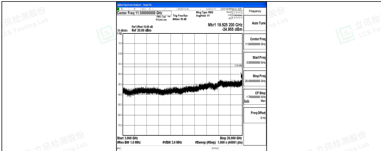
Band25_5MHz_16QAM_26365_1RB#0_3000~20000_3000~20000
