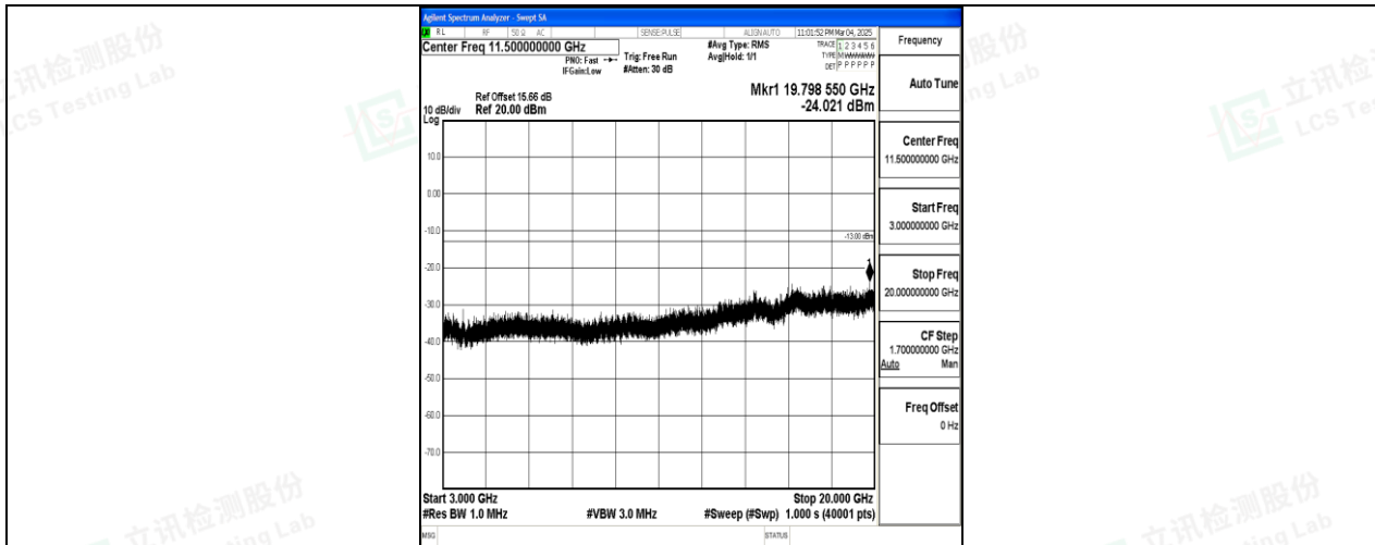
Band25_10MHz_16QAM_26365_1RB#0_3000~20000_3000~20000
