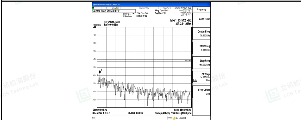
Band25_10MHz_QPSK_26640_1RB#0_0.009~0.15_0.009~0.15
