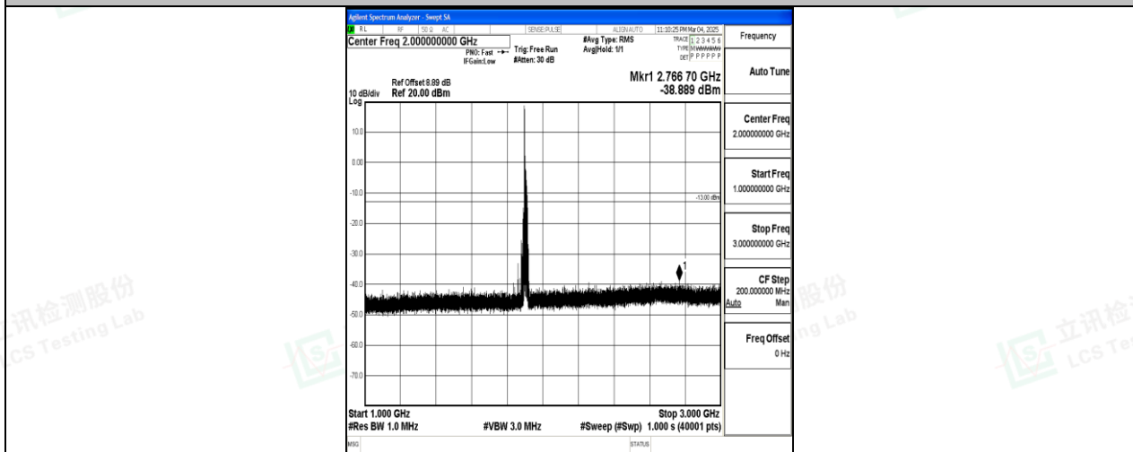
Band25_20MHz_QPSK_26590_1RB#0_1000~3000_1000~3000
