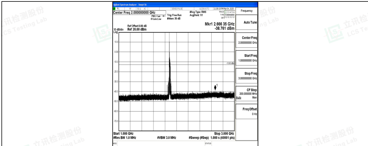
Band25_20MHz_QPSK_26365_1RB#0_1000~3000_1000~3000
