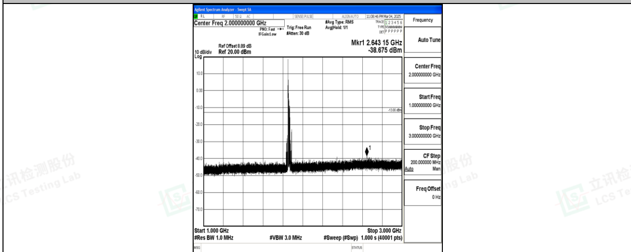
Band25_20MHz_16QAM_26140_1RB#0_1000~3000_1000~3000
