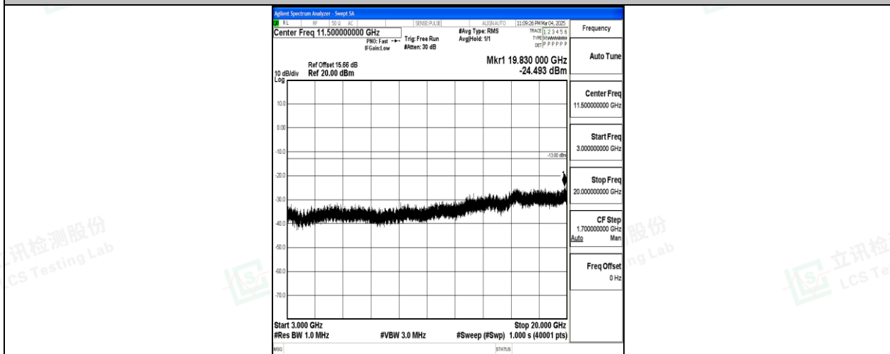
Band25_20MHz_QPSK_26365_1RB#0_3000~20000_3000~20000
