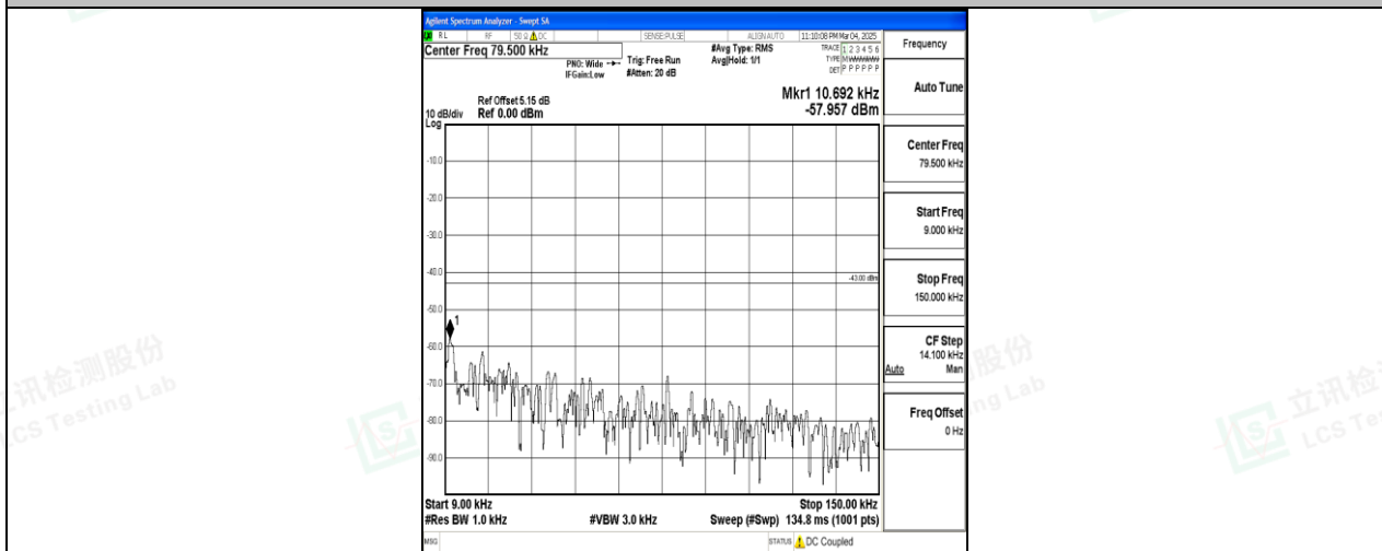
Band25_20MHz_QPSK_26590_1RB#0_0.009~0.15_0.009~0.15
