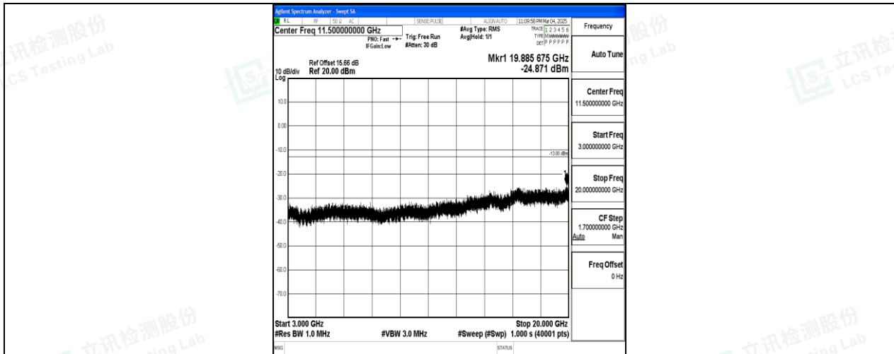
Band25_20MHz_16QAM_26365_1RB#0_3000~20000_3000~20000
