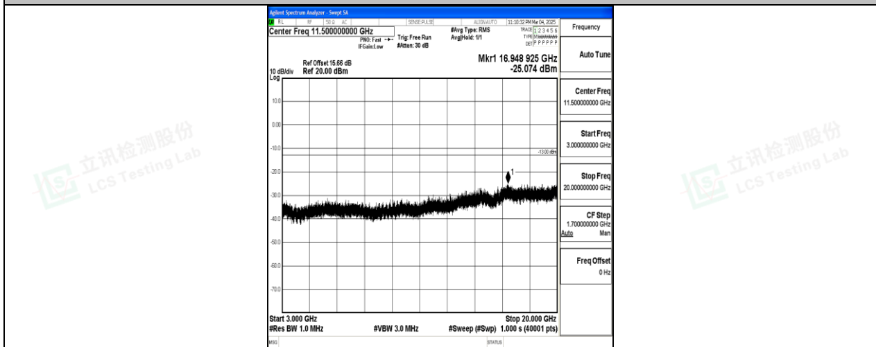
Band25_20MHz_QPSK_26590_1RB#0_3000~20000_3000~20000
