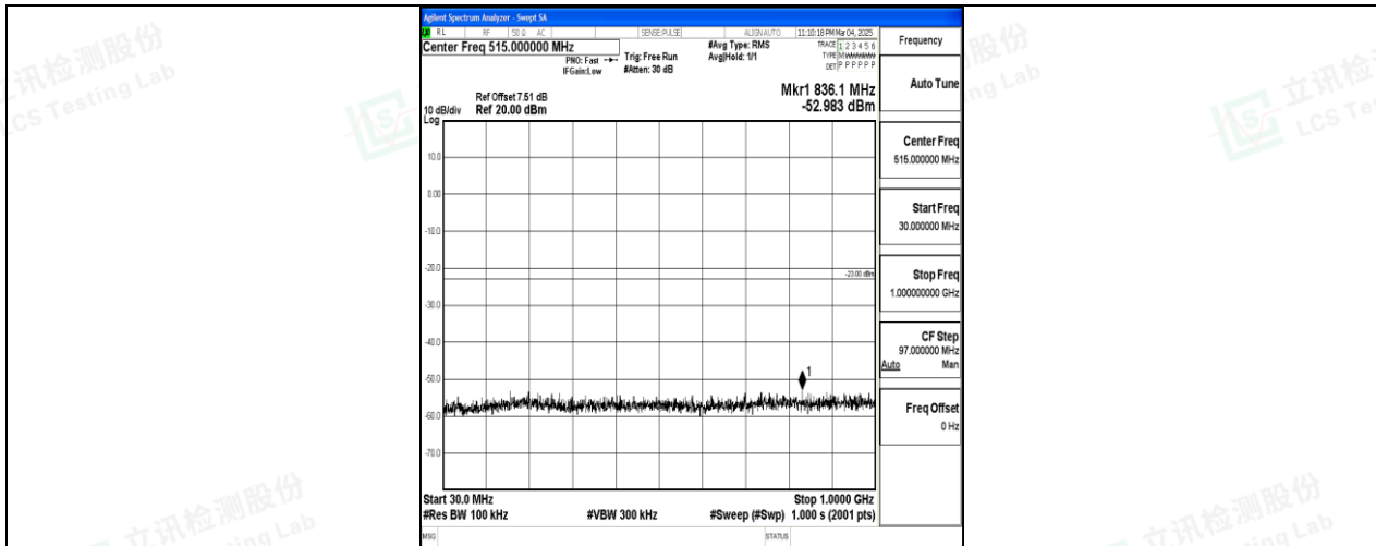
Band25_20MHz_QPSK_26590_1RB#0_30~1000_30~1000
