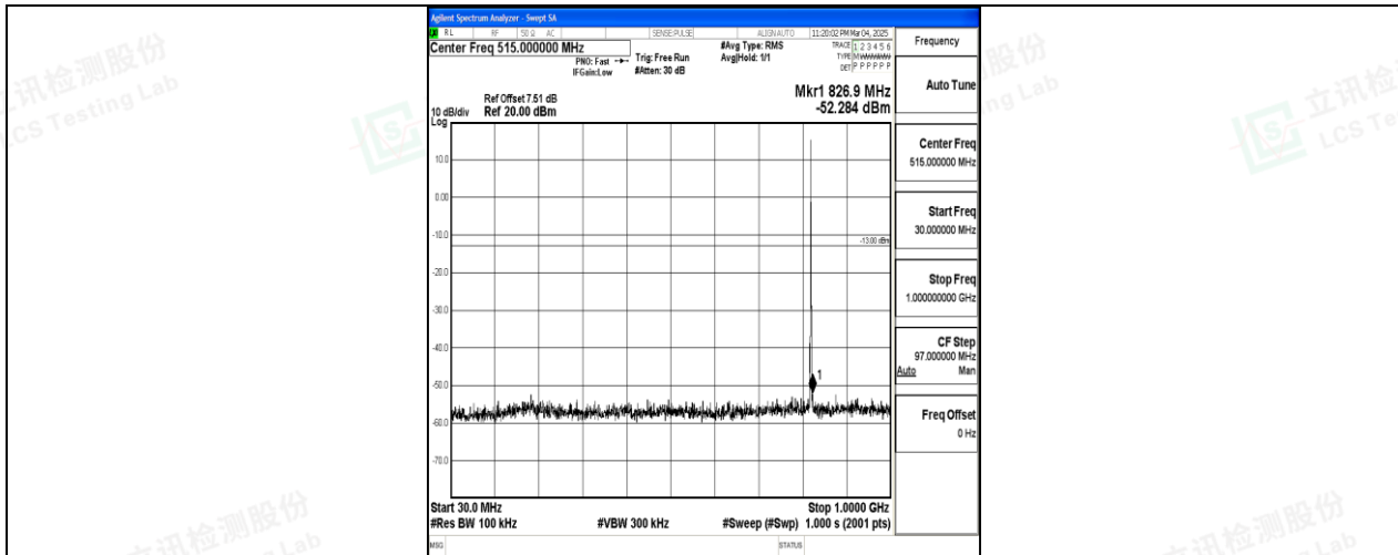
Band26_1.4MHz_QPSK_26783_1RB#0_30~1000_30~1000
