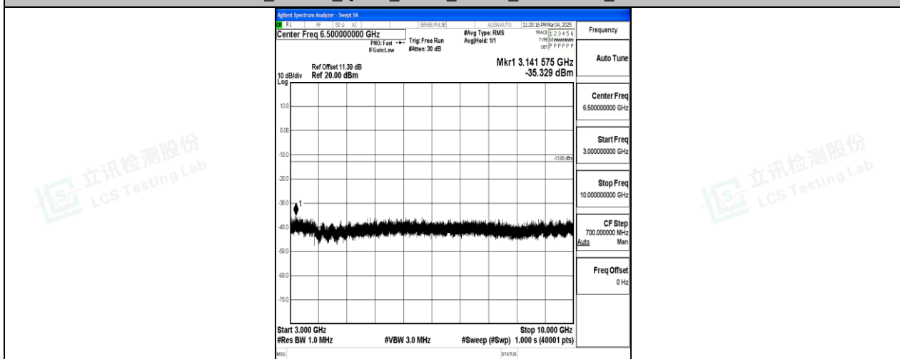
Band26_1.4MHz_QPSK_26783_1RB#0_3000~10000_3000~10000
