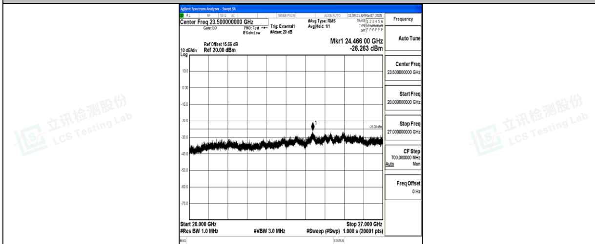
Band41_10MHz_QPSK_41540_1RB#0_20000~27000_20000~27000
