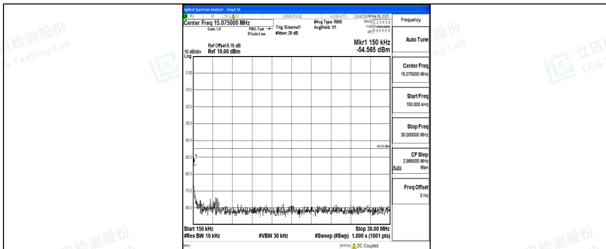
Band41_20MHz_QPSK_39750_1RB#0_0.15~30_0.15~30
