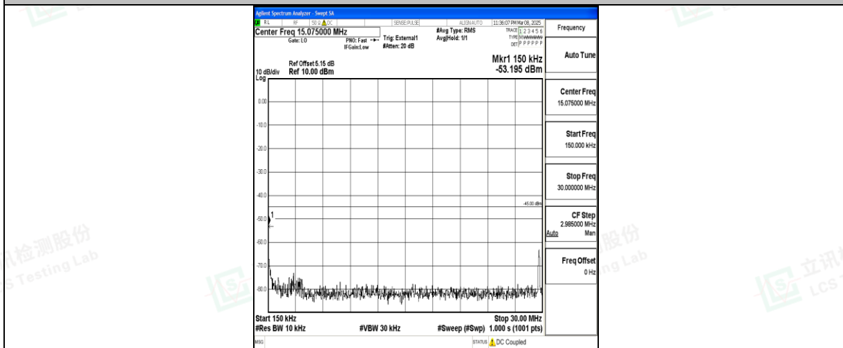
Band41_5MHz_16QAM_40620_1RB#0_0.15~30_0.15~30
