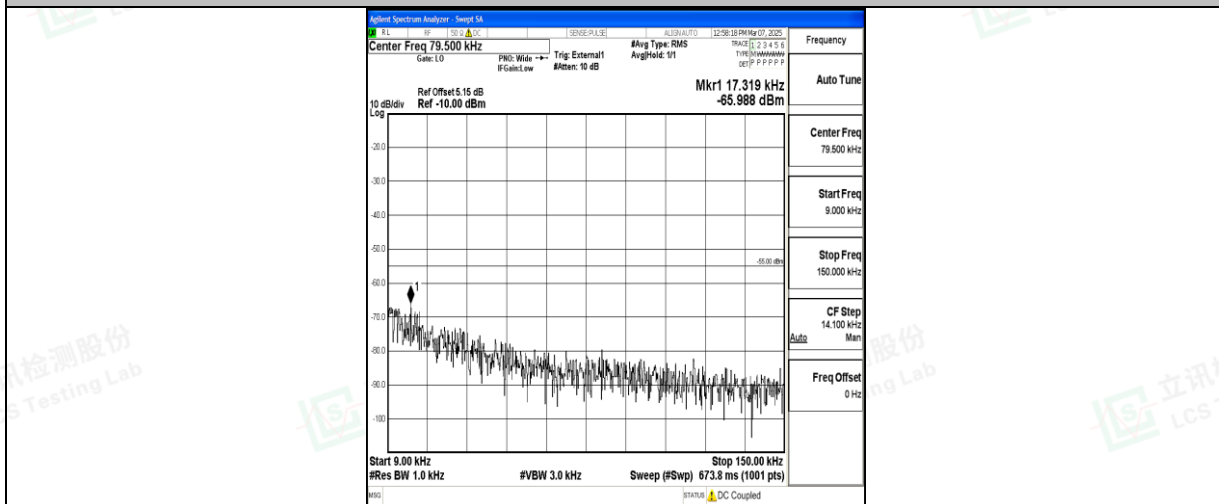
Band41_15MHz_16QAM_39725_1RB#0_0.009~0.15_0.009~0.15
