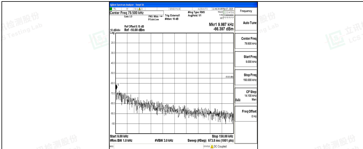
Band41_10MHz_QPSK_40620_1RB#0_0.009~0.15_0.009~0.15
