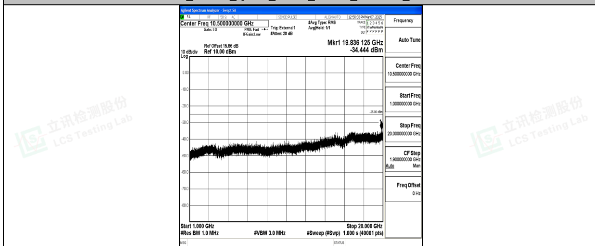
Band41_15MHz_QPSK_39725_1RB#0_1000~20000_1000~20000
