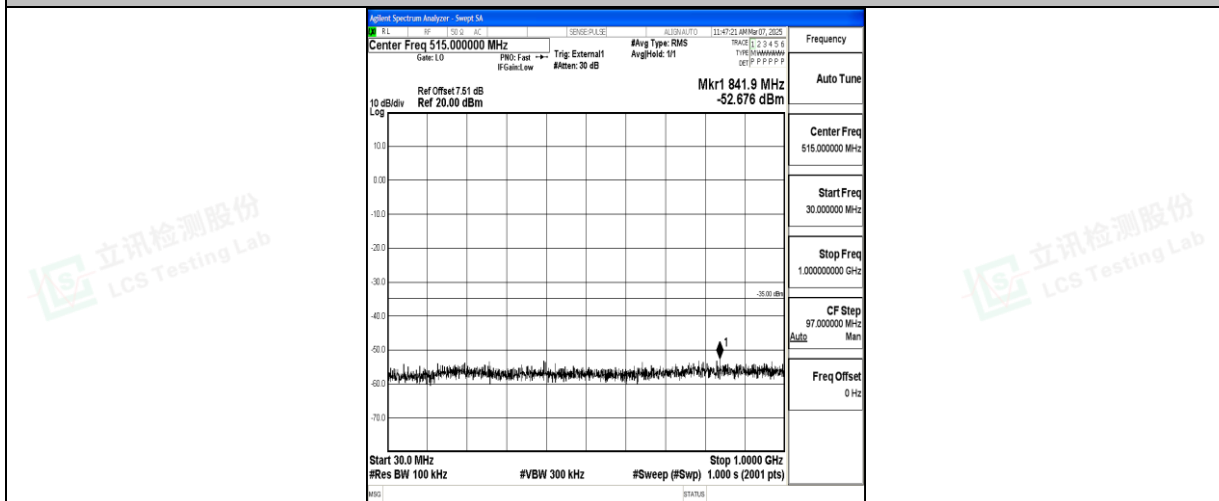
Band41_10MHz_QPSK_40620_1RB#0_30~1000_30~1000
