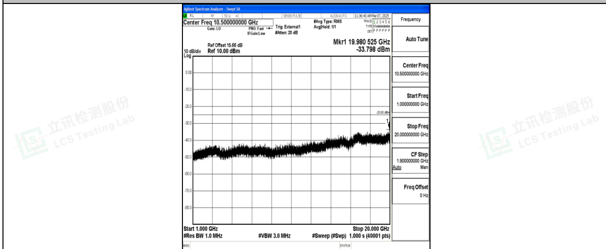
Band41_10MHz_QPSK_39700_1RB#0_1000~20000_1000~20000
