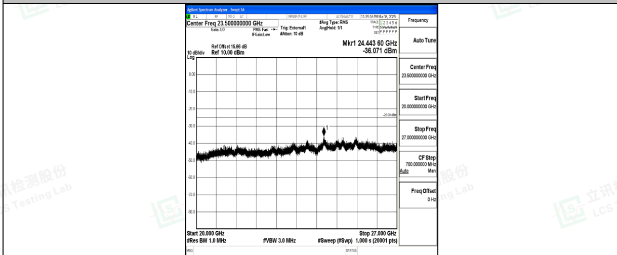
Band41_5MHz_QPSK_41565_1RB#0_20000~27000_20000~27000
