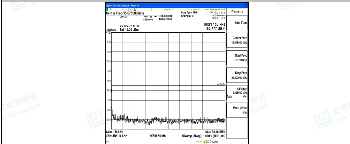
Band41_10MHz_QPSK_40620_1RB#0_0.15~30_0.15~30
