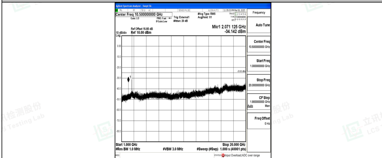
Band41_5MHz_QPSK_40620_1RB#0_1000~20000_1000~20000
