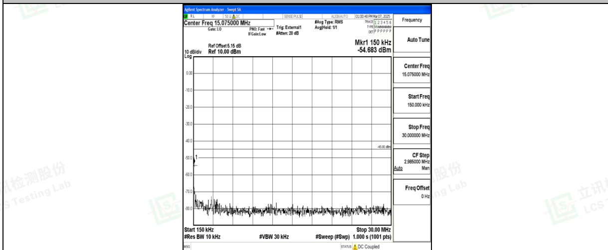
Band41_15MHz_QPSK_40620_1RB#0_0.15~30_0.15~30
