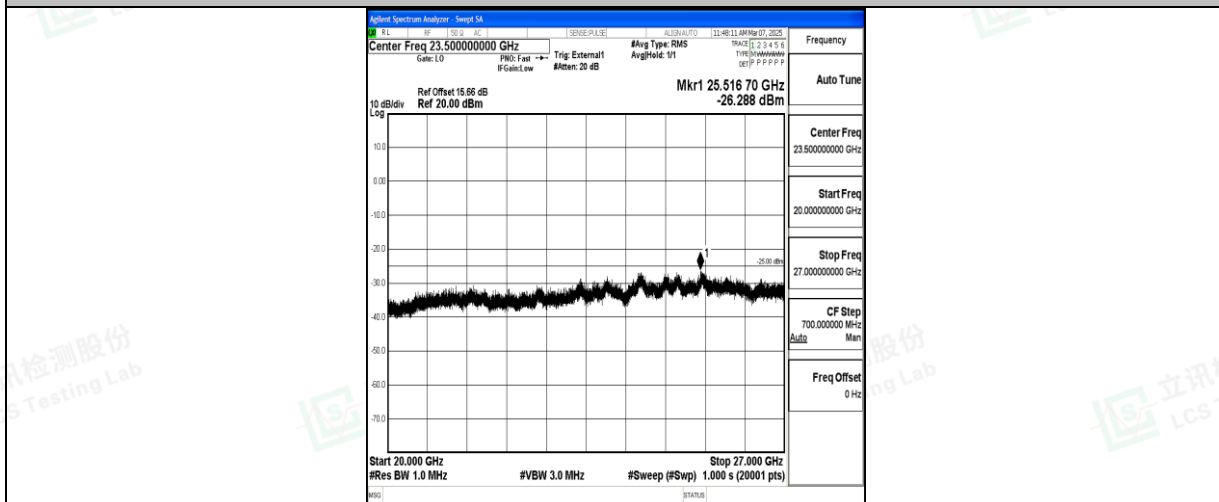
Band41_10MHz_QPSK_40620_1RB#0_20000~27000_20000~27000
