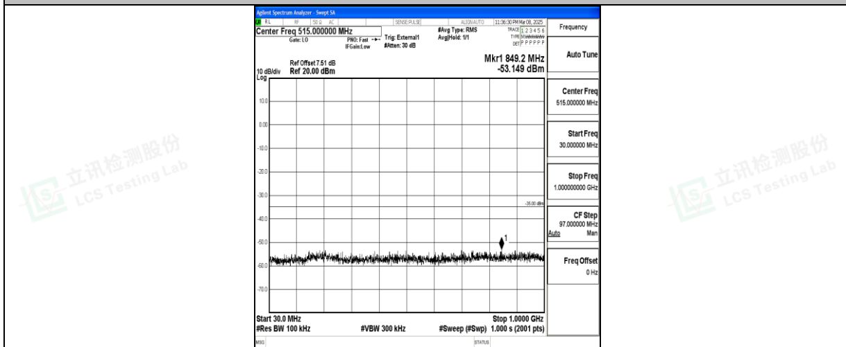
Band41_5MHz_16QAM_40620_1RB#0_30~1000_30~1000
