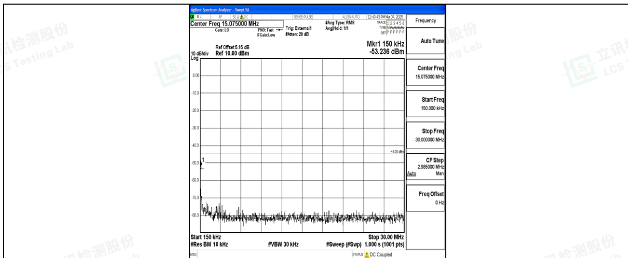
Band41_15MHz_QPSK_39725_1RB#0_0.15~30_0.15~30
