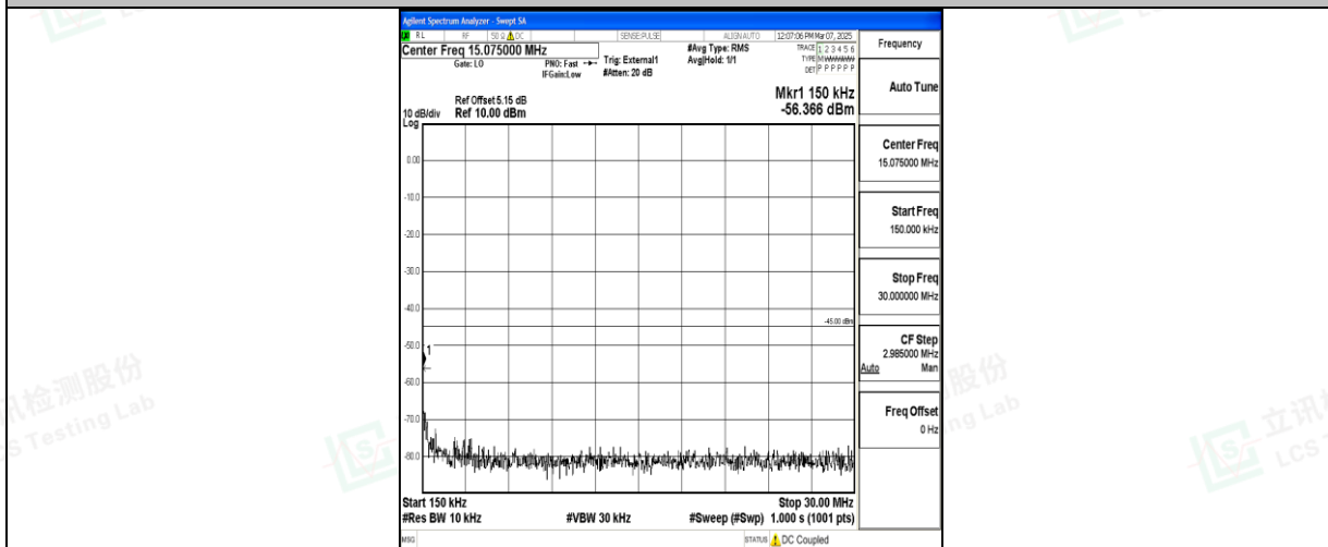
Band41_10MHz_16QAM_41540_1RB#0_0.15~30_0.15~30
