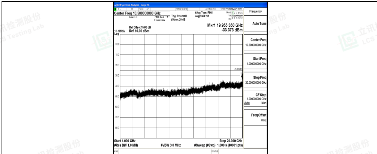
Band41_10MHz_16QAM_41540_1RB#0_1000~20000_1000~20000
