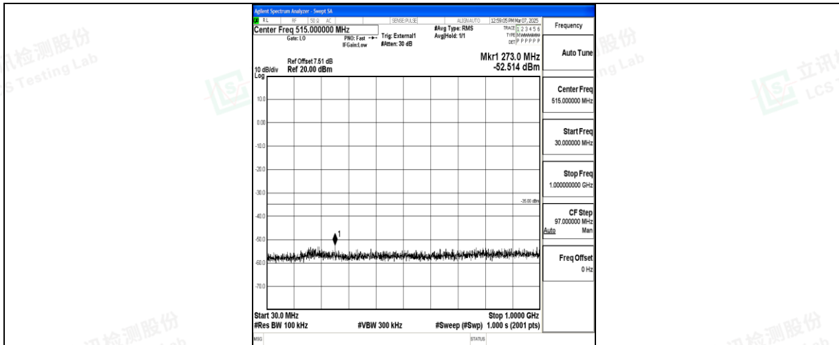
Band41_15MHz_16QAM_39725_1RB#0_30~1000_30~1000
