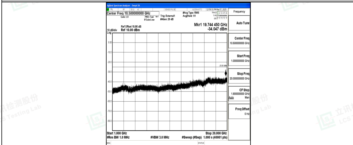
Band41_15MHz_16QAM_39725_1RB#0_1000~20000_1000~20000
