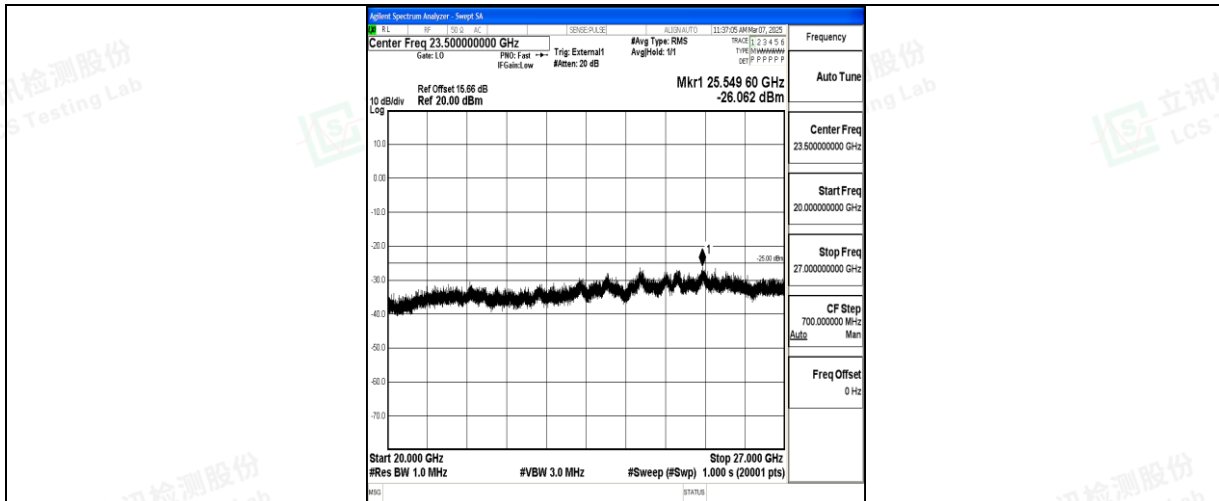
Band41_10MHz_QPSK_39700_1RB#0_20000~27000_20000~27000
