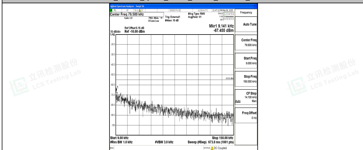
Band41_20MHz_16QAM_40620_1RB#0_0.009~0.15_0.009~0.15
