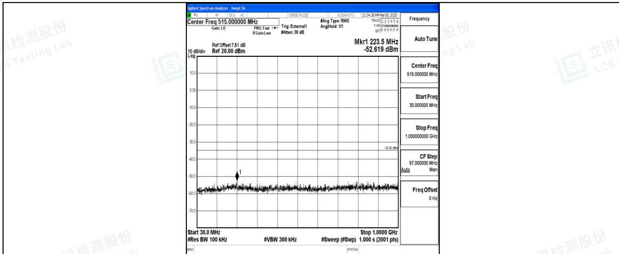
Band41_5MHz_QPSK_40620_1RB#0_30~1000_30~1000
