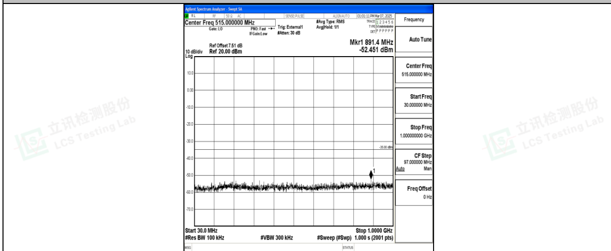
Band41_15MHz_QPSK_40620_1RB#0_30~1000_30~1000
