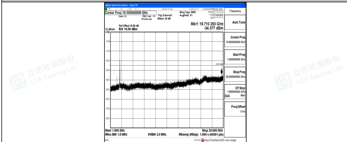
Band41_20MHz_16QAM_40620_1RB#0_1000~20000_1000~20000
