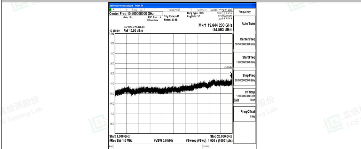
Band41_10MHz_QPSK_41540_1RB#0_1000~20000_1000~20000
