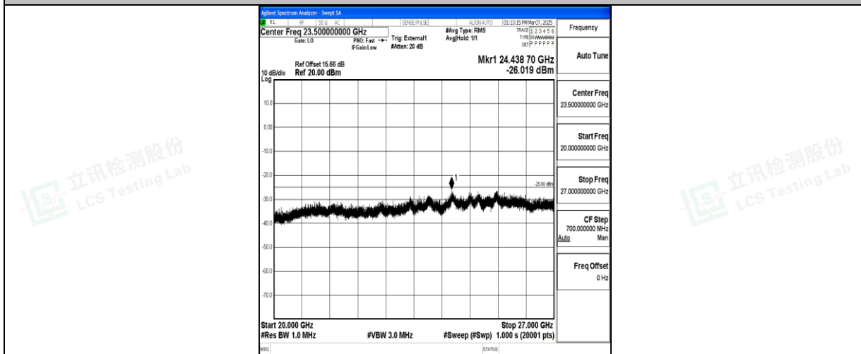
Band41_15MHz_QPSK_41515_1RB#0_20000~27000_20000~27000
