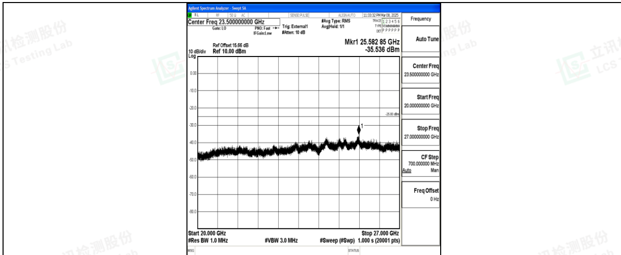
Band41_5MHz_16QAM_39675_1RB#0_20000~27000_20000~27000
