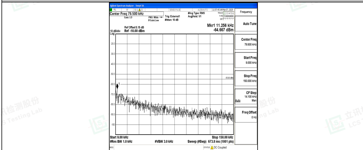
Band41_10MHz_QPSK_41540_1RB#0_0.009~0.15_0.009~0.15
