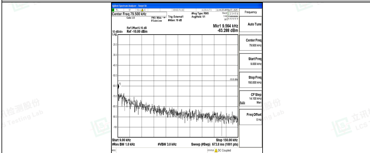
Band41_10MHz_16QAM_39700_1RB#0_0.009~0.15_0.009~0.15
