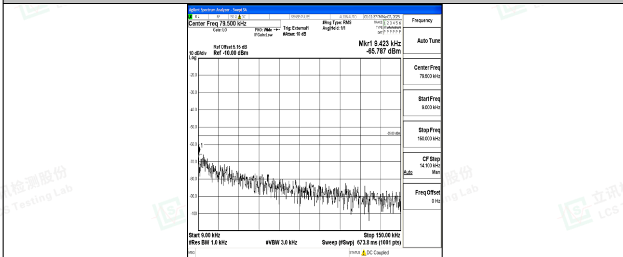
Band41_15MHz_QPSK_41515_1RB#0_0.009~0.15_0.009~0.15
