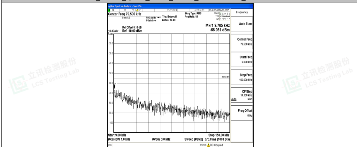
Band41_10MHz_16QAM_40620_1RB#0_0.009~0.15_0.009~0.15
