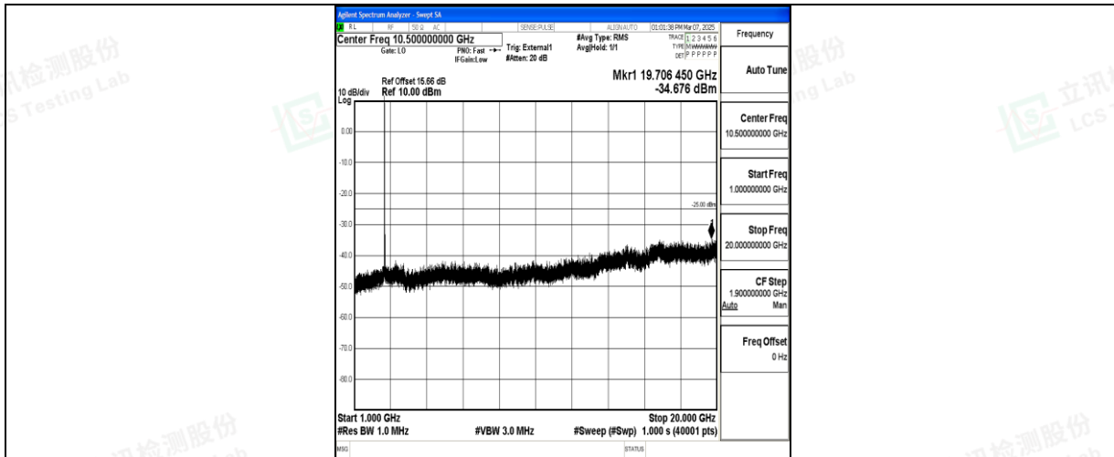
Band41_15MHz_QPSK_40620_1RB#0_1000~20000_1000~20000
