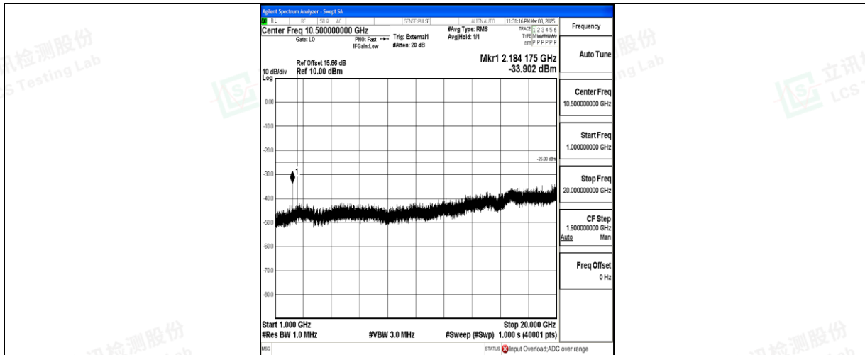
Band41_5MHz_QPSK_39675_1RB#0_1000~20000_1000~20000
