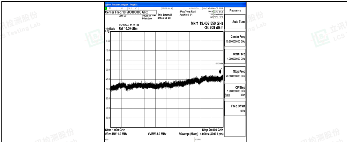
Band41_10MHz_QPSK_40620_1RB#0_1000~20000_1000~20000
