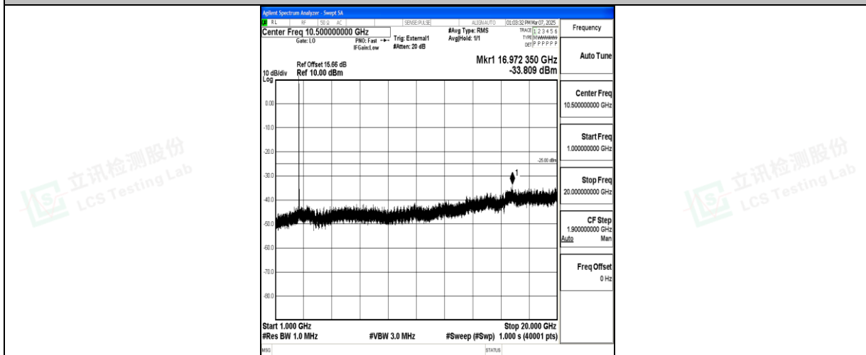
Band41_15MHz_16QAM_40620_1RB#0_1000~20000_1000~20000
