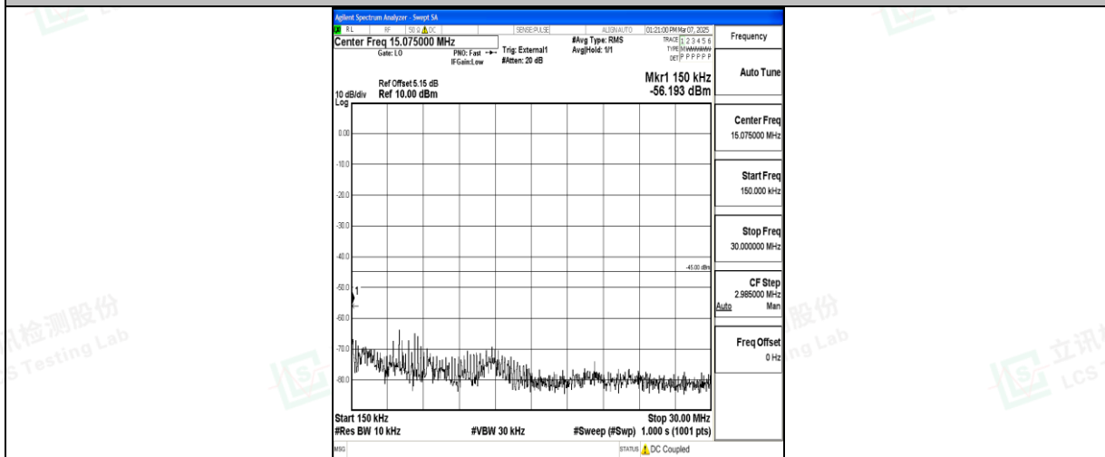
Band41_15MHz_16QAM_41515_1RB#0_0.15~30_0.15~30
