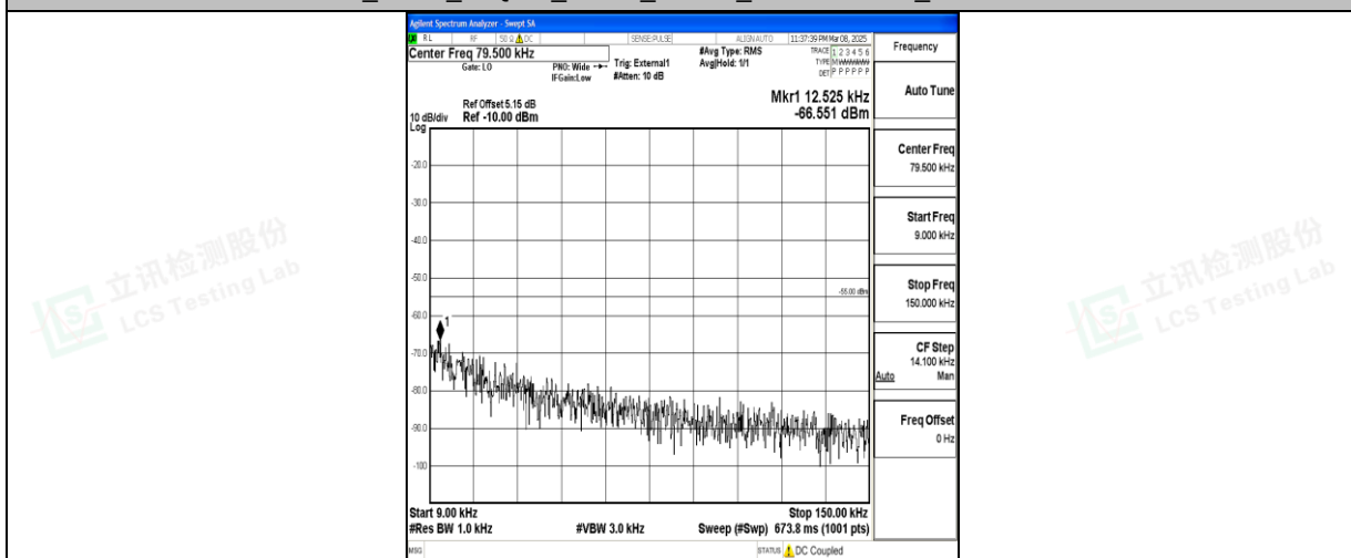
Band41_5MHz_QPSK_41565_1RB#0_0.009~0.15_0.009~0.15
