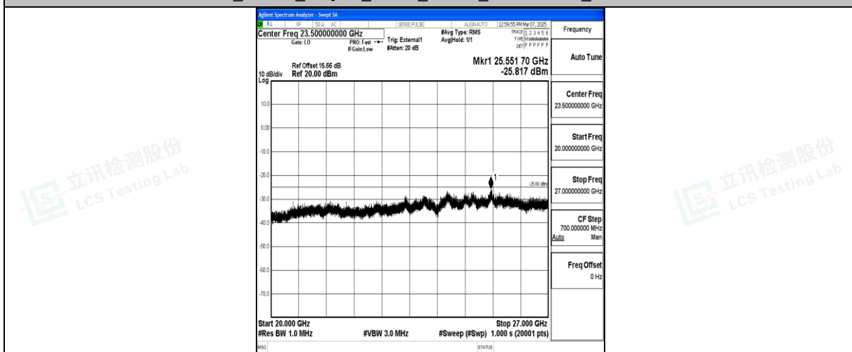
Band41_15MHz_16QAM_39725_1RB#0_20000~27000_20000~27000
