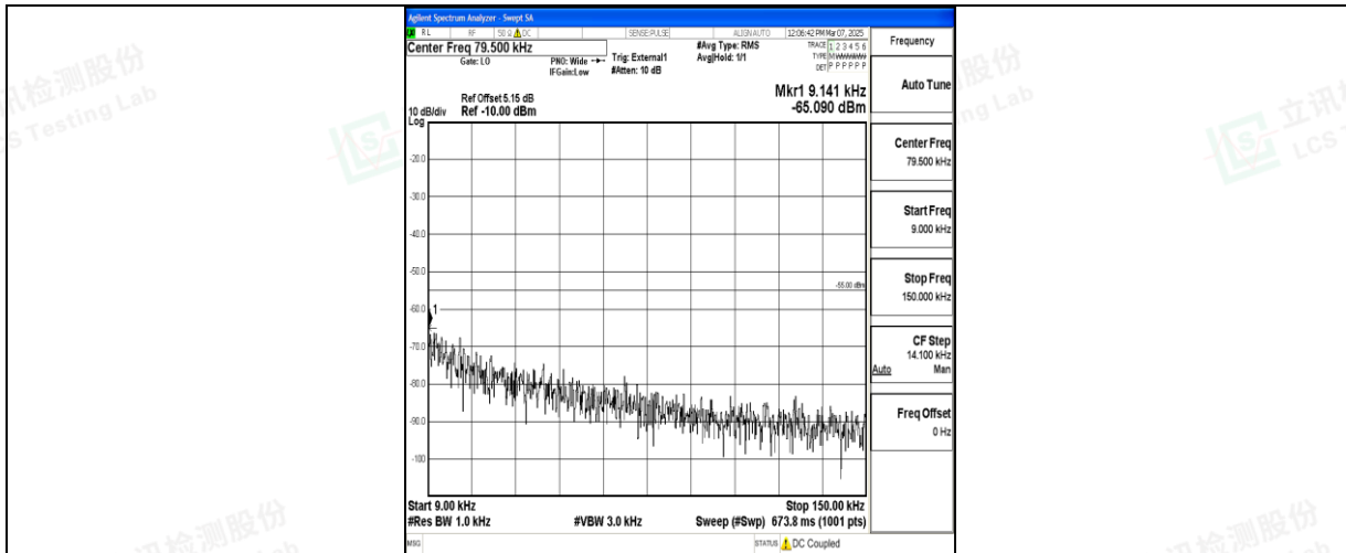
Band41_10MHz_16QAM_41540_1RB#0_0.009~0.15_0.009~0.15
