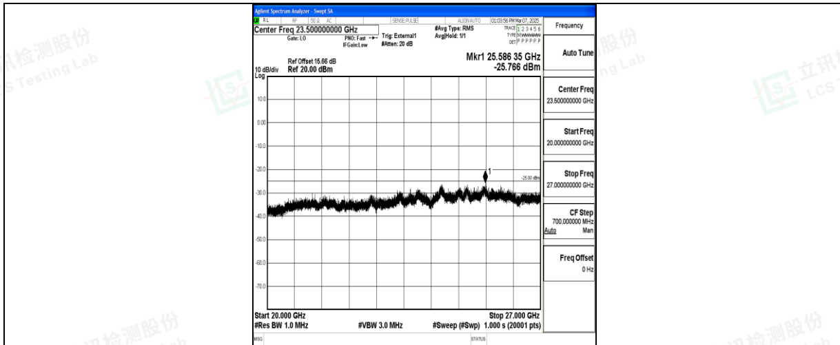
Band41_15MHz_16QAM_40620_1RB#0_20000~27000_20000~27000
