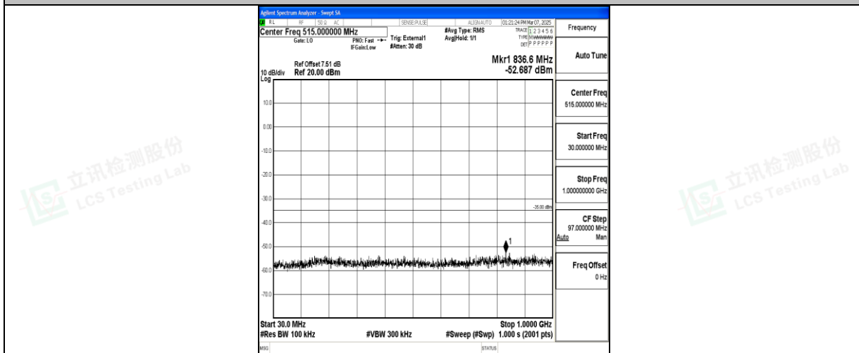
Band41_15MHz_16QAM_41515_1RB#0_30~1000_30~1000
