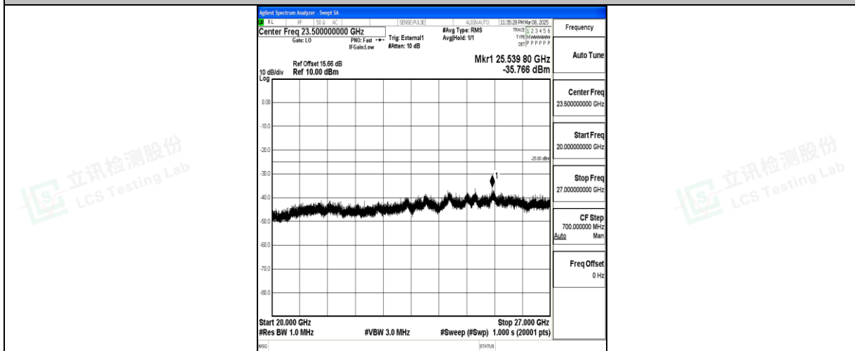
Band41_5MHz_QPSK_40620_1RB#0_20000~27000_20000~27000
