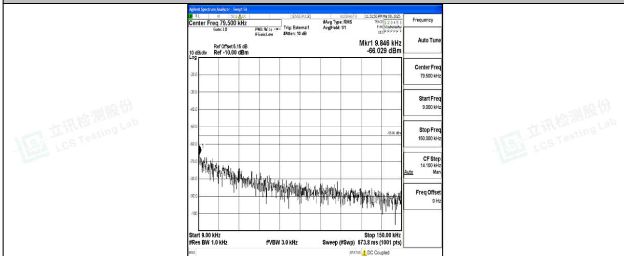
Band41_5MHz_16QAM_39675_1RB#0_0.009~0.15_0.009~0.15
