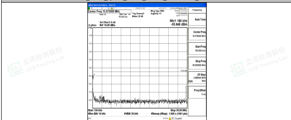
Band41_5MHz_QPSK_40620_1RB#0_0.15~30_0.15~30
