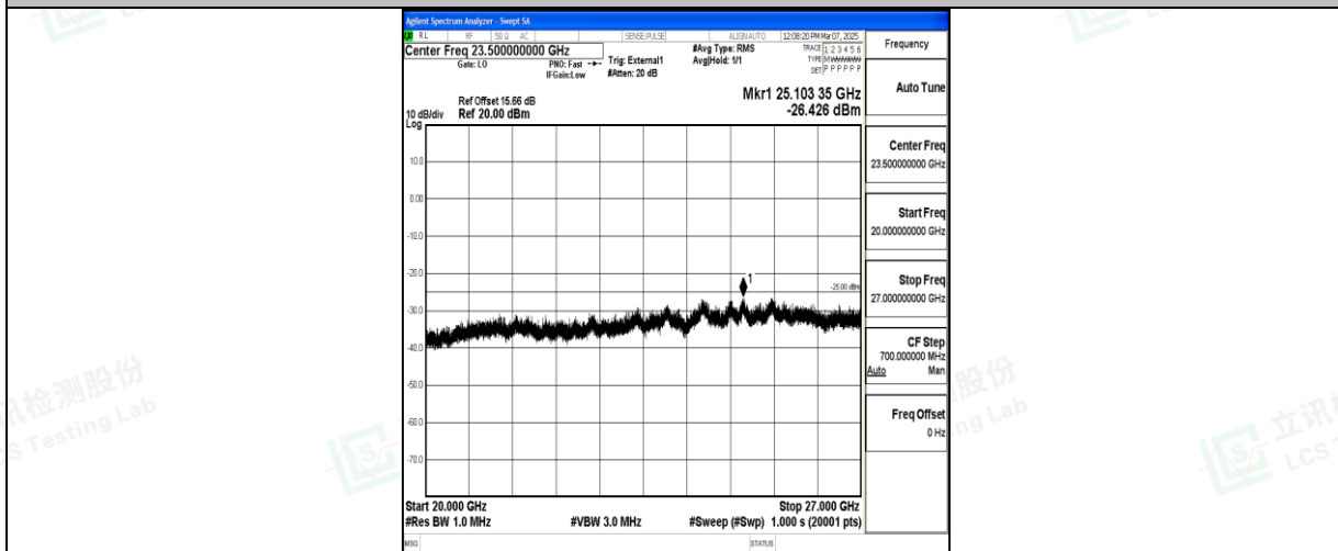
Band41_10MHz_16QAM_41540_1RB#0_20000~27000_20000~27000
