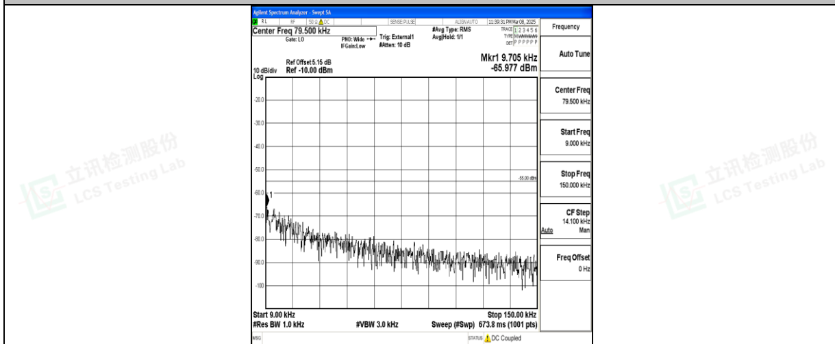
Band41_5MHz_16QAM_41565_1RB#0_0.009~0.15_0.009~0.15
