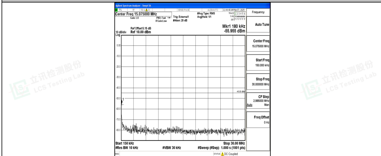
Band41_10MHz_16QAM_39700_1RB#0_0.15~30_0.15~30
