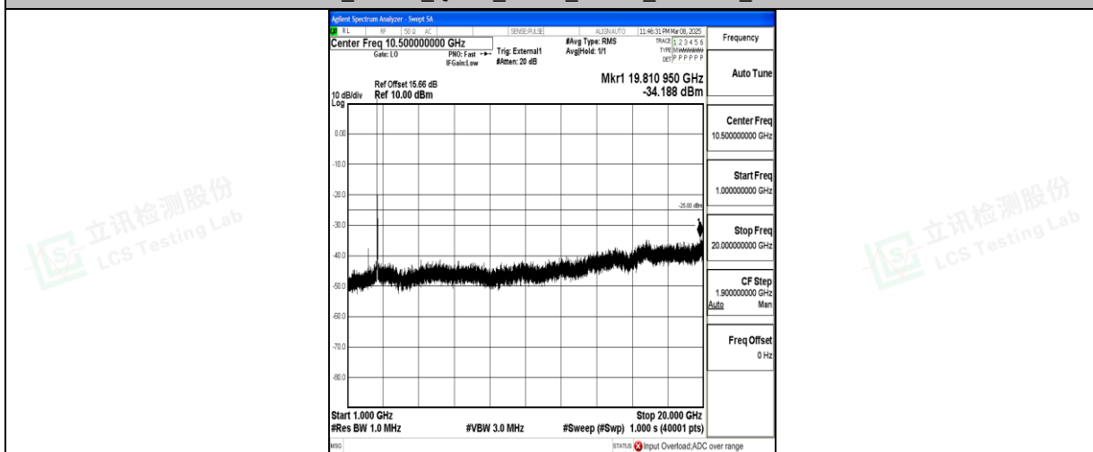
Band41_20MHz_QPSK_40620_1RB#0_1000~20000_1000~20000
