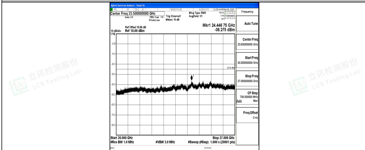
Band41_20MHz_QPSK_41490_1RB#0_20000~27000_20000~27000
