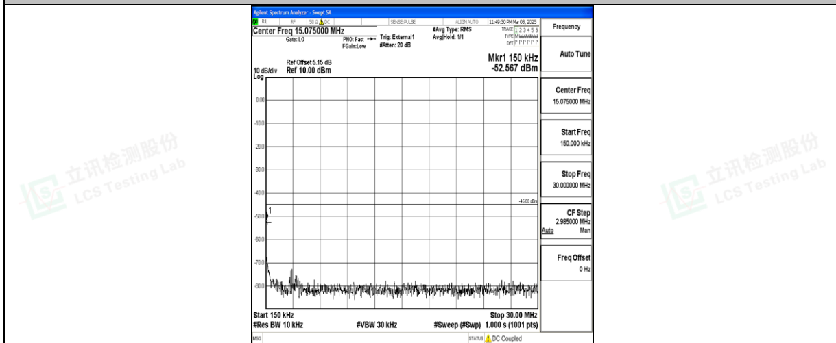
Band41_20MHz_QPSK_41490_1RB#0_0.15~30_0.15~30
