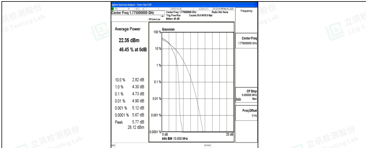
Band66-10MHz-16QAM-132622-1RB#0-PASS
