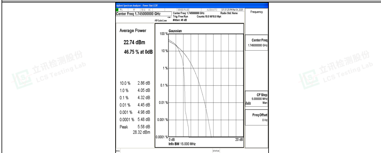
Band66-15MHz-16QAM-132322-1RB#0-PASS
