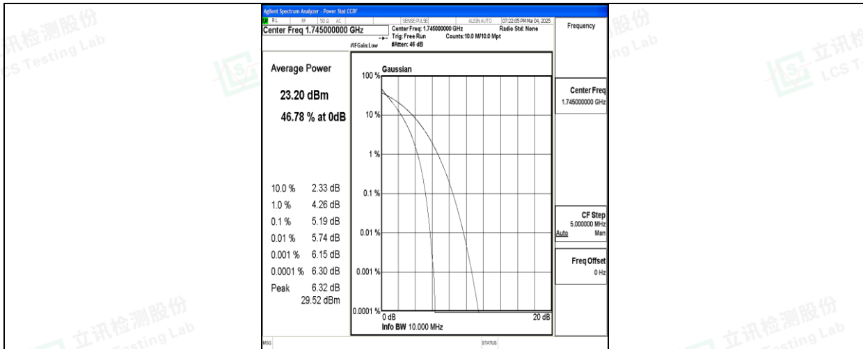
Band66-10MHz-QPSK-132322-50RB#0-PASS
