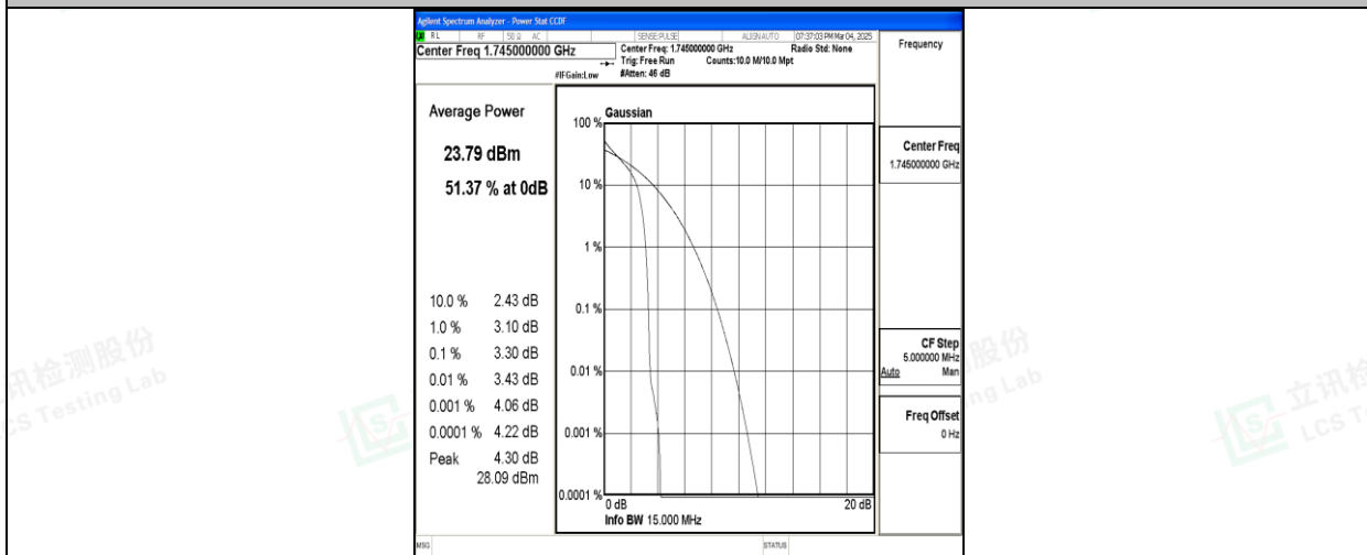
Band66-15MHz-QPSK-132322-1RB#0-PASS
