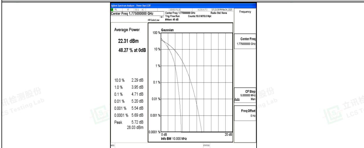
Band66-10MHz-QPSK-132622-50RB#0-PASS
