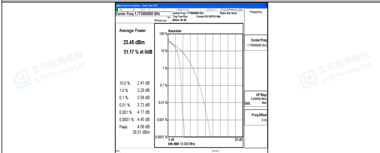
Band66-10MHz-QPSK-132622-1RB#0-PASS
