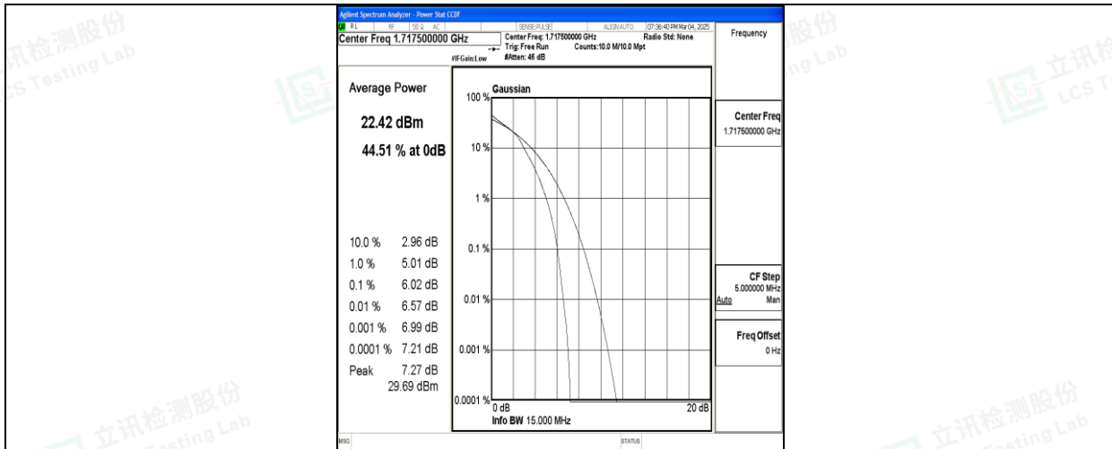
Band66-15MHz-16QAM-132047-75RB#0-PASS
