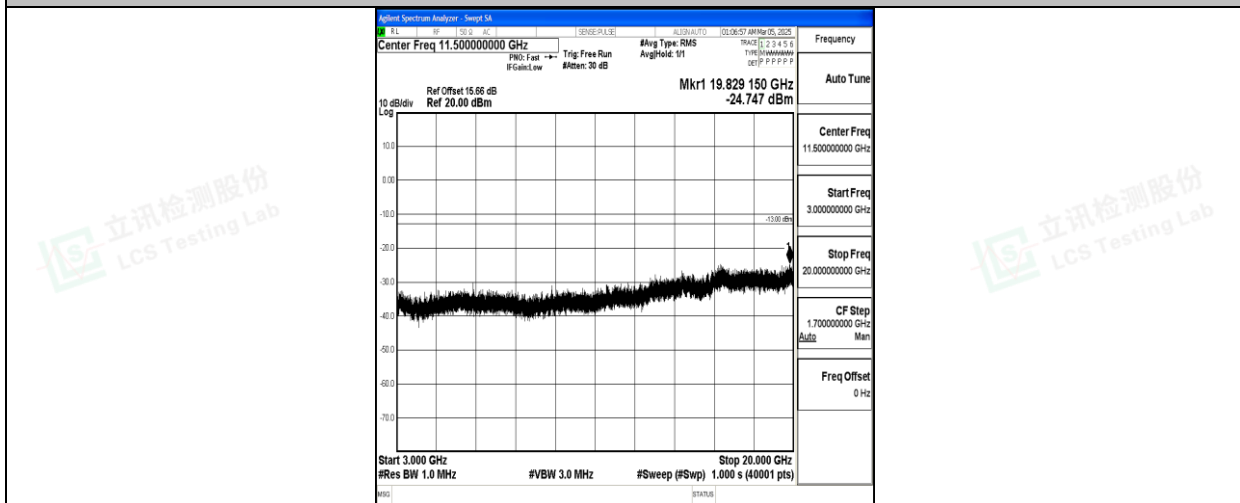
Band66_5MHz_QPSK_132647_1RB#0_3000~20000_3000~20000
