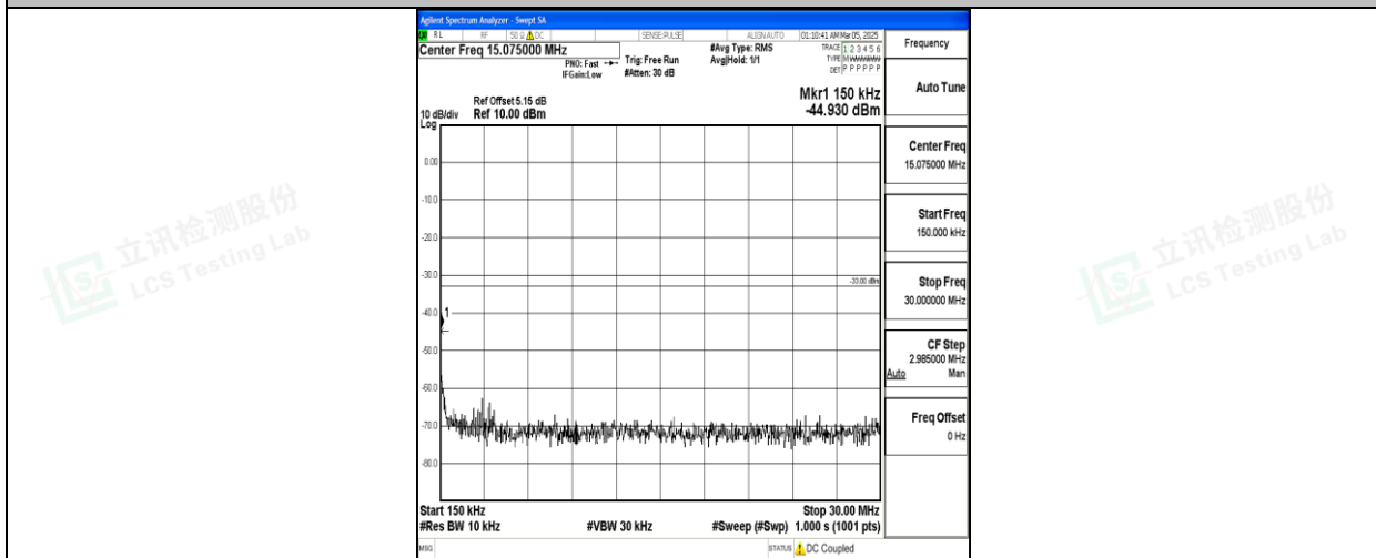
Band66_10MHz_QPSK_132622_1RB#0_0.15~30_0.15~30
