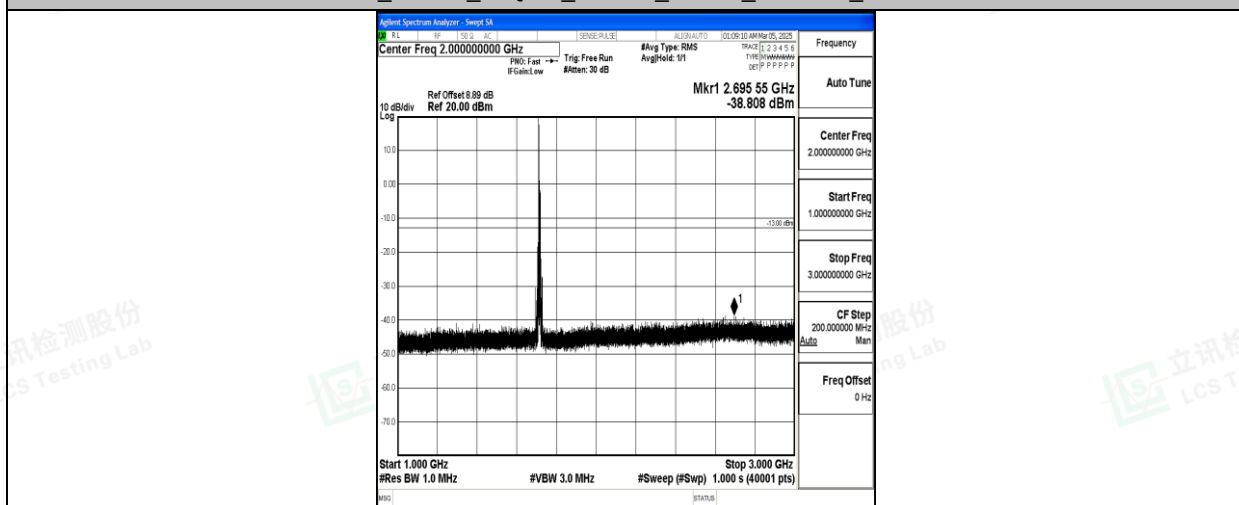
Band66_10MHz_16QAM_132022_1RB#0_1000~3000_1000~3000
