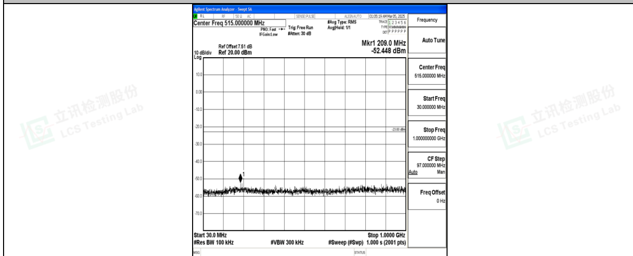
Band66_5MHz_QPSK_132322_1RB#0_30~1000_30~1000
