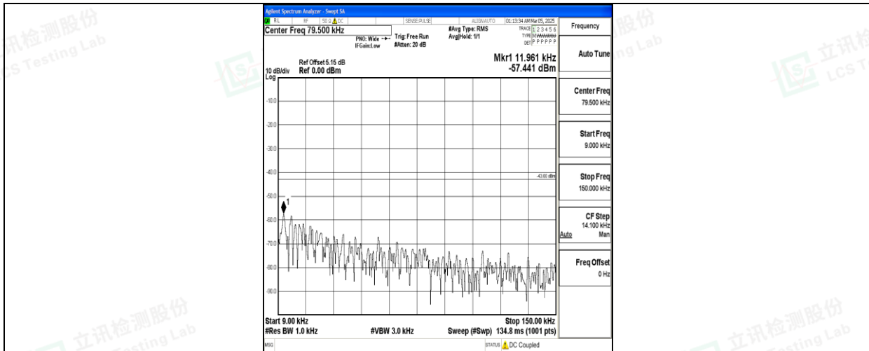
Band66_15MHz_QPSK_132322_1RB#0_0.009~0.15_0.009~0.15
