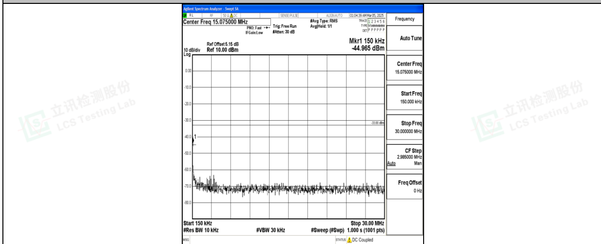
Band66_5MHz_16QAM_131997_1RB#0_0.15~30_0.15~30
