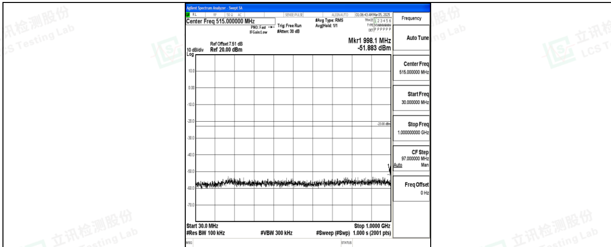
Band66_5MHz_QPSK_132647_1RB#0_30~1000_30~1000
