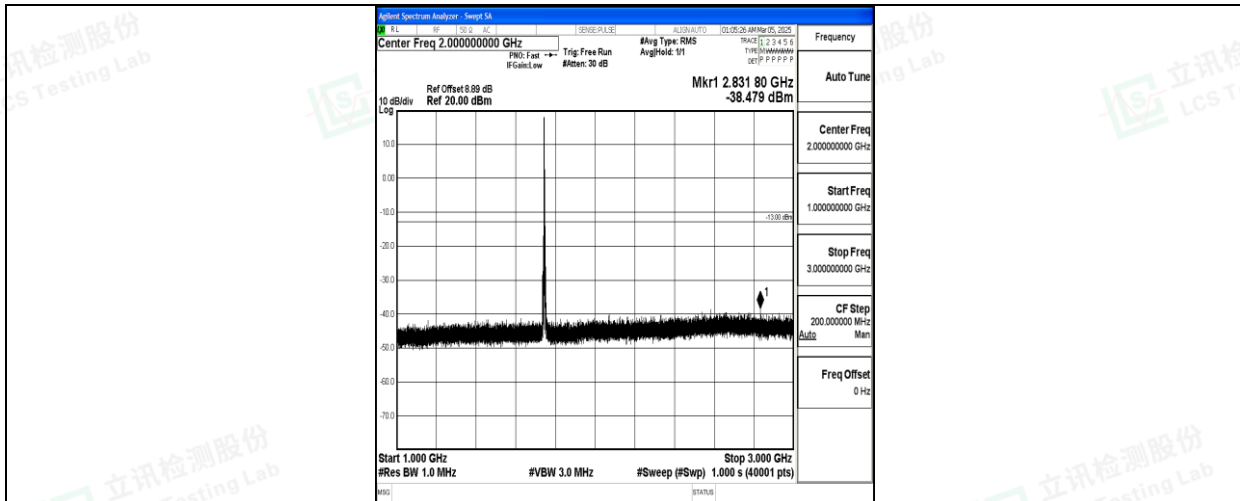
Band66_5MHz_QPSK_132322_1RB#0_1000~3000_1000~3000
