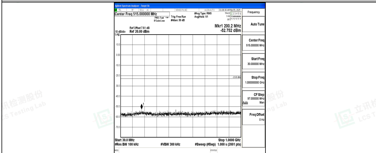
Band66_10MHz_QPSK_132022_1RB#0_30~1000_30~1000
