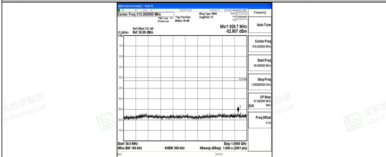
Band66_15MHz_16QAM_132322_1RB#0_30~1000_30~1000
