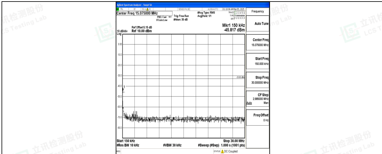
Band66_10MHz_16QAM_132322_1RB#0_0.15~30_0.15~30
