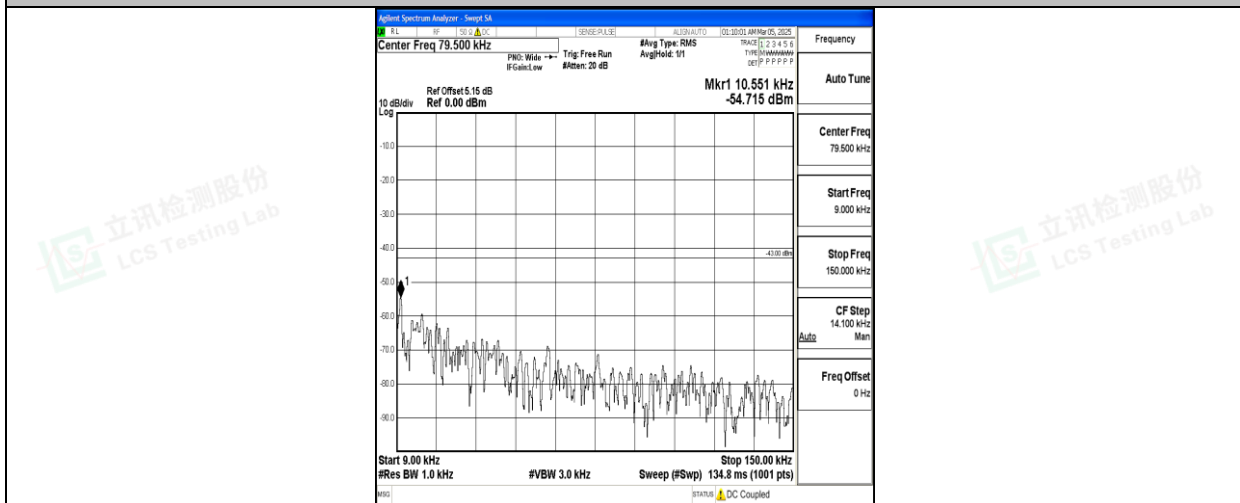
Band66_10MHz_16QAM_132322_1RB#0_0.009~0.15_0.009~0.15
