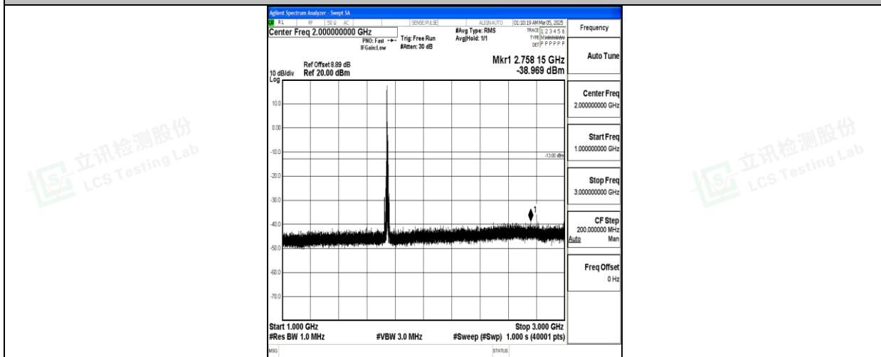
Band66_10MHz_16QAM_132322_1RB#0_1000~3000_1000~3000
