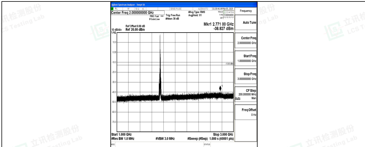
Band66_10MHz_QPSK_132322_1RB#0_1000~3000_1000~3000
