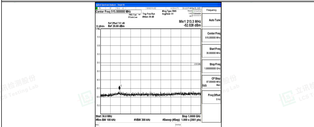
Band66_15MHz_QPSK_132047_1RB#0_30~1000_30~1000
