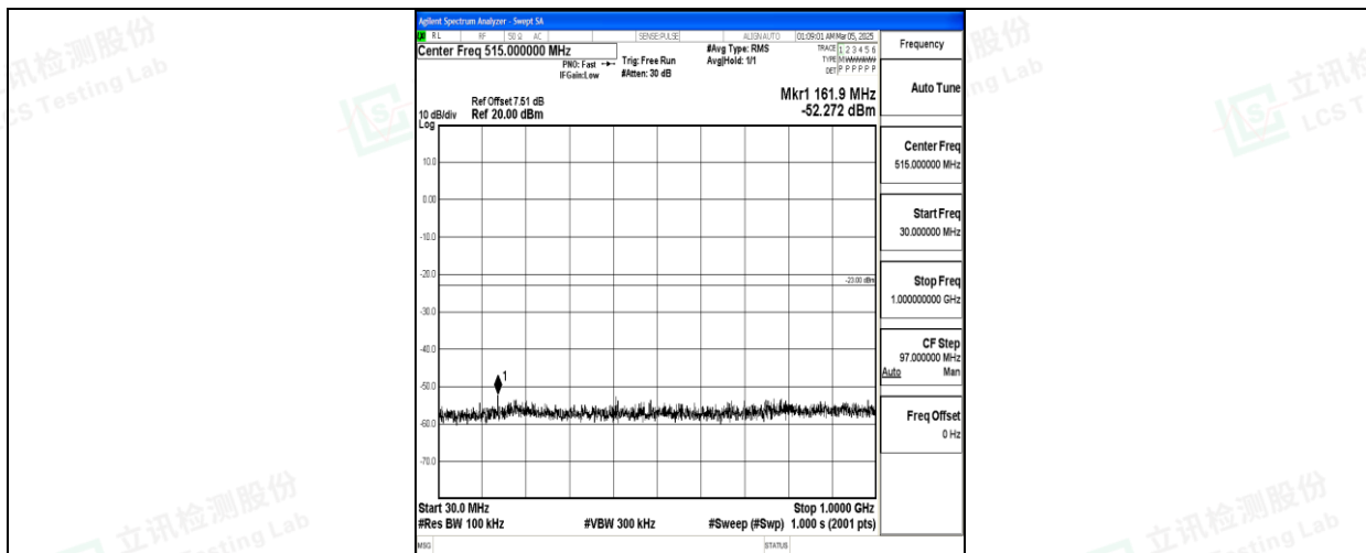
Band66_10MHz_16QAM_132022_1RB#0_30~1000_30~1000
