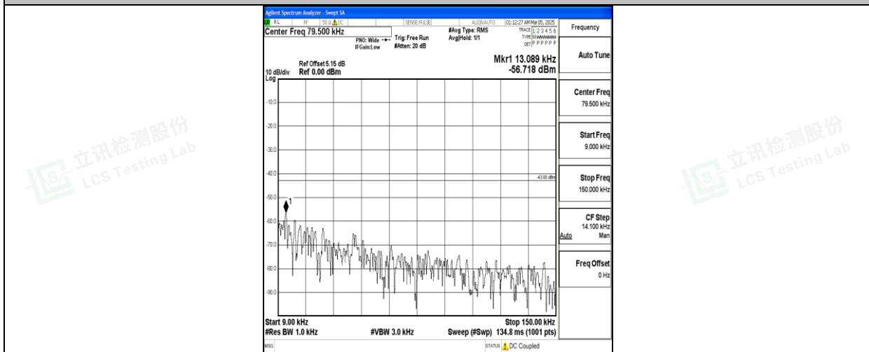
Band66_15MHz_QPSK_132047_1RB#0_0.009~0.15_0.009~0.15
