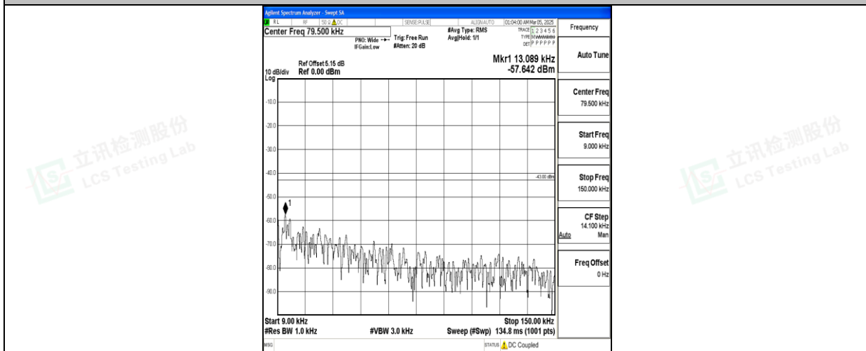
Band66_5MHz_QPSK_131997_1RB#0_0.009~0.15_0.009~0.15
