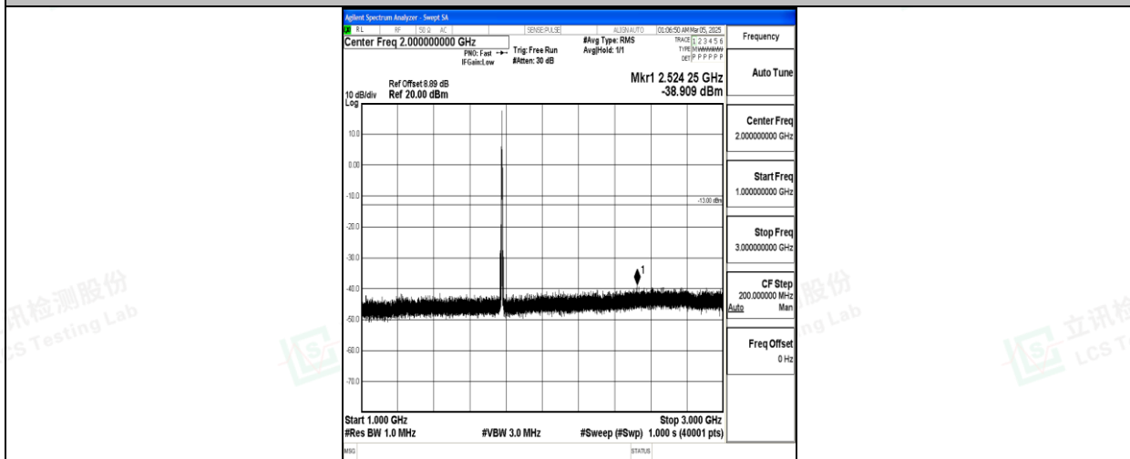
Band66_5MHz_QPSK_132647_1RB#0_1000~3000_1000~3000
