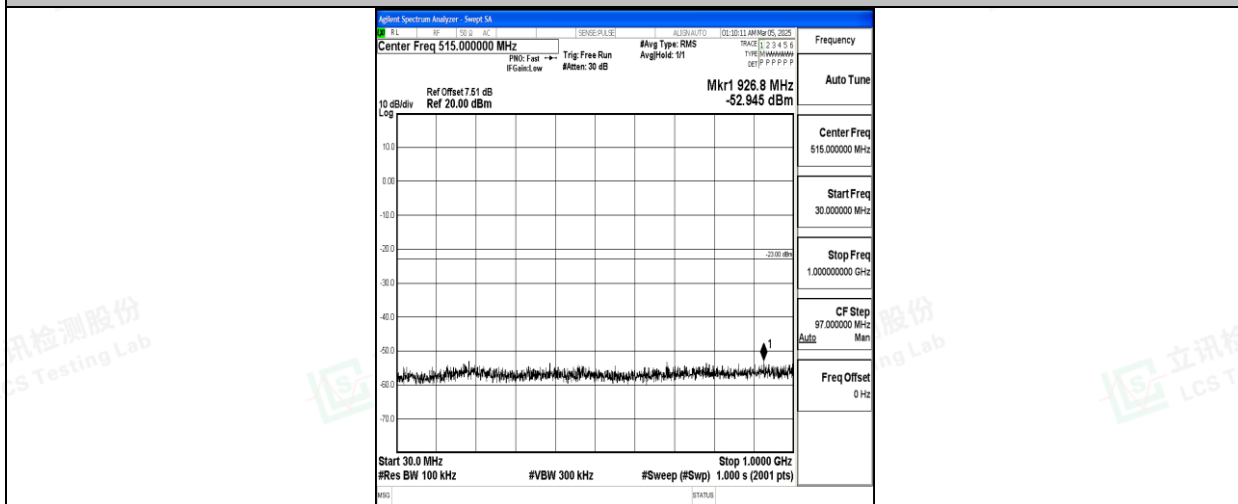
Band66_10MHz_16QAM_132322_1RB#0_30~1000_30~1000
