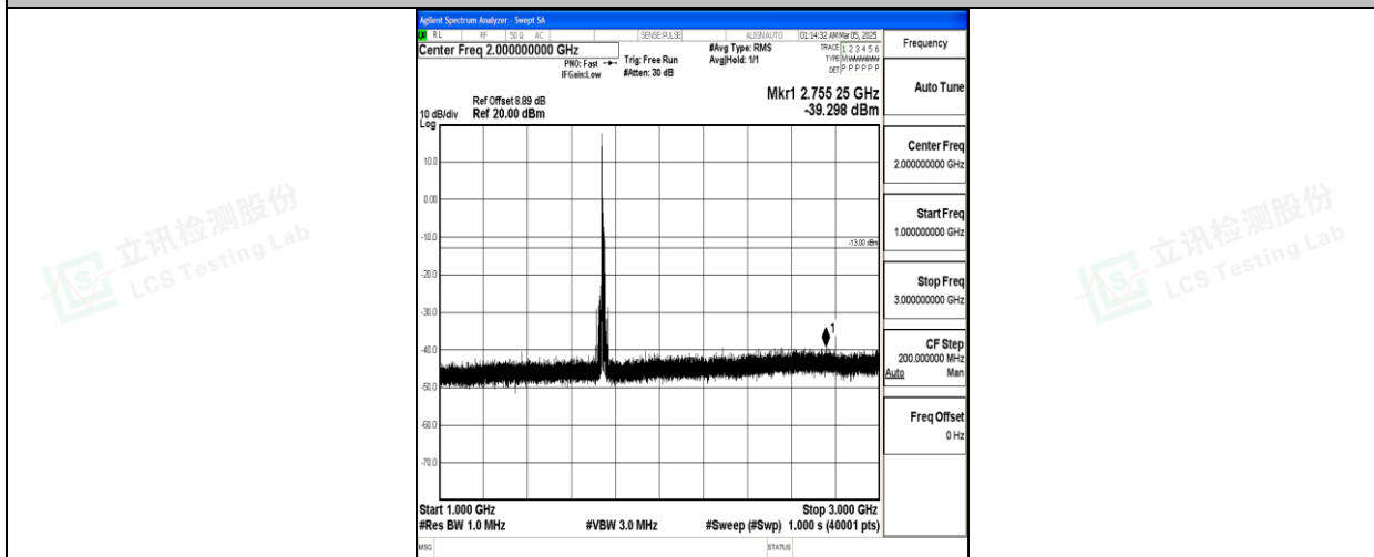
Band66_15MHz_16QAM_132322_1RB#0_1000~3000_1000~3000
