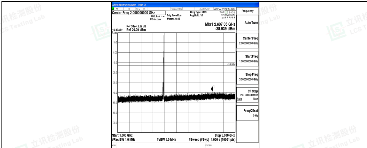
Band66_5MHz_16QAM_132647_1RB#0_1000~3000_1000~3000
