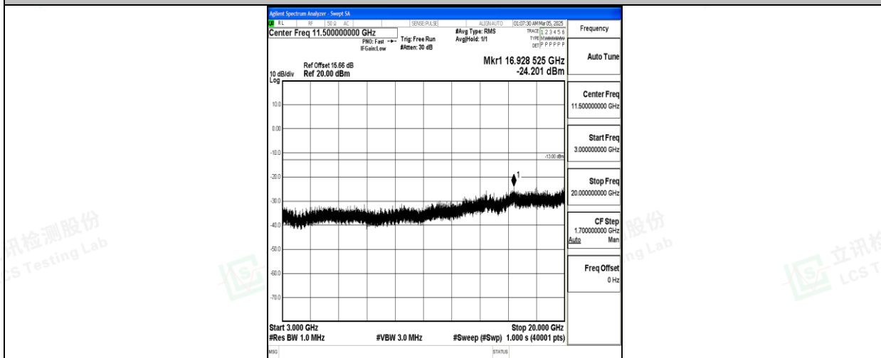
Band66_5MHz_16QAM_132647_1RB#0_3000~20000_3000~20000
