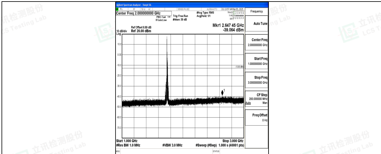
Band66_15MHz_QPSK_132322_1RB#0_1000~3000_1000~3000
