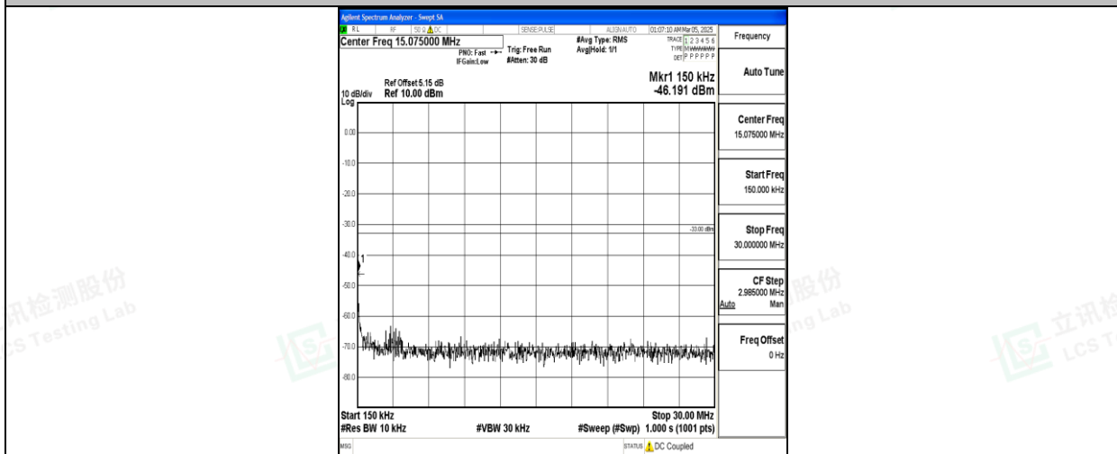
Band66_5MHz_16QAM_132647_1RB#0_0.15~30_0.15~30
