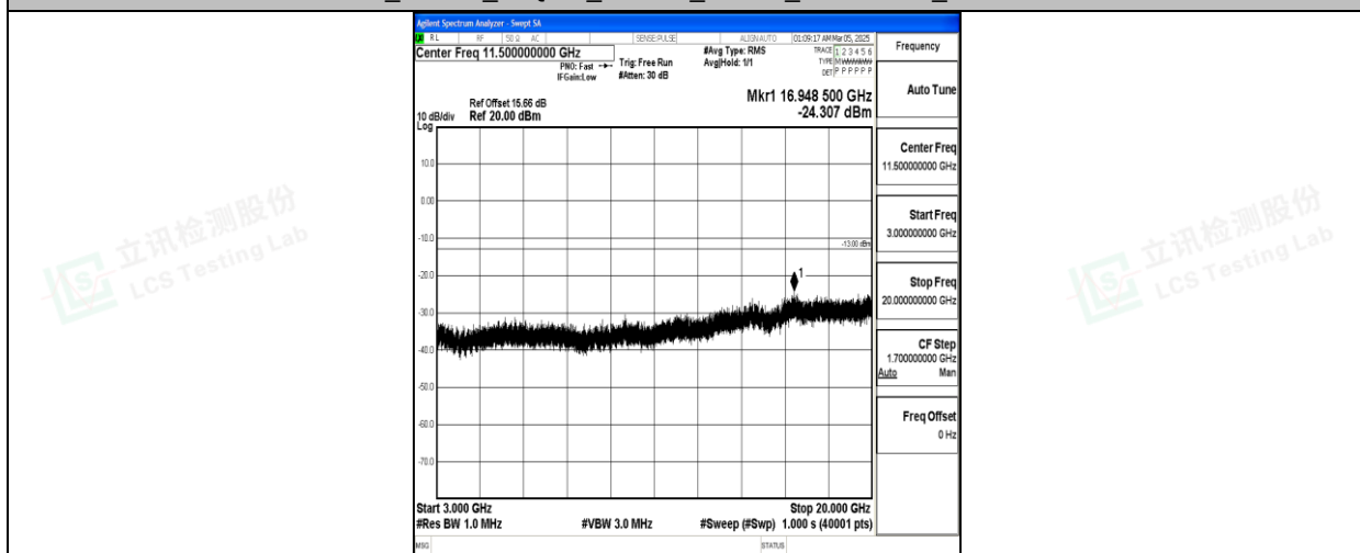
Band66_10MHz_16QAM_132022_1RB#0_3000~20000_3000~20000
