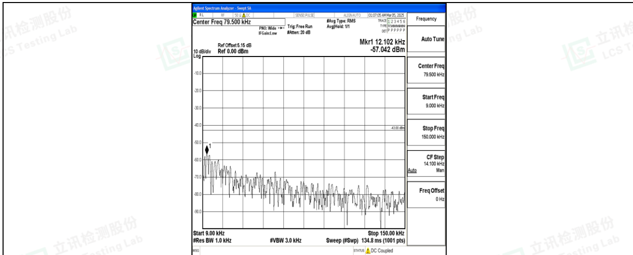
Band66_5MHz_16QAM_132647_1RB#0_0.009~0.15_0.009~0.15
