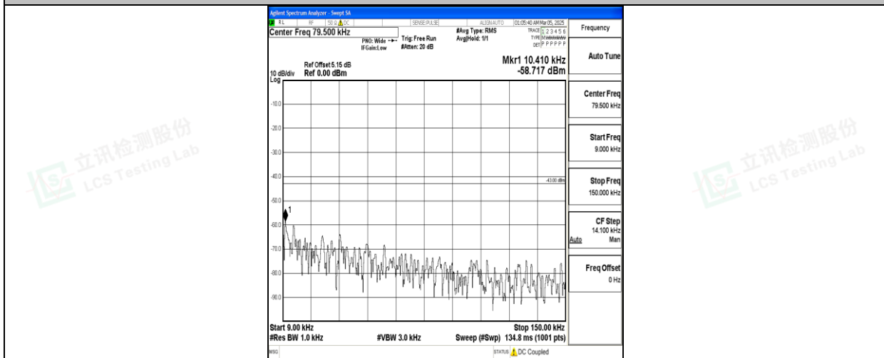
Band66_5MHz_16QAM_132322_1RB#0_0.009~0.15_0.009~0.15
