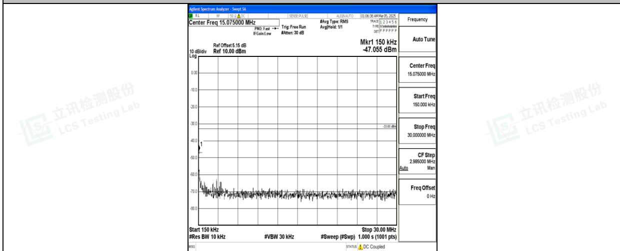
Band66_5MHz_QPSK_132647_1RB#0_0.15~30_0.15~30
