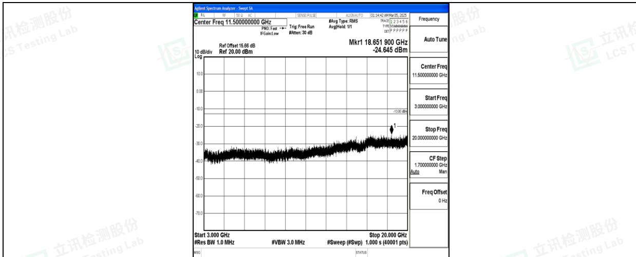
Band66_15MHz_16QAM_132322_1RB#0_3000~20000_3000~20000
