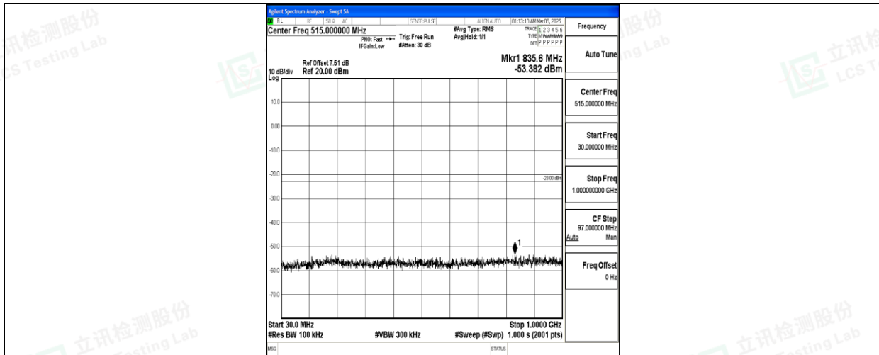
Band66_15MHz_16QAM_132047_1RB#0_30~1000_30~1000
