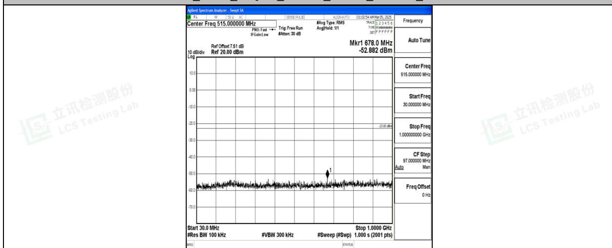
Band66_3MHz_16QAM_132657_1RB#0_30~1000_30~1000
