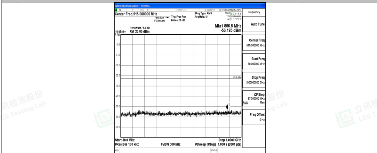
Band66_5MHz_QPSK_131997_1RB#0_30~1000_30~1000
