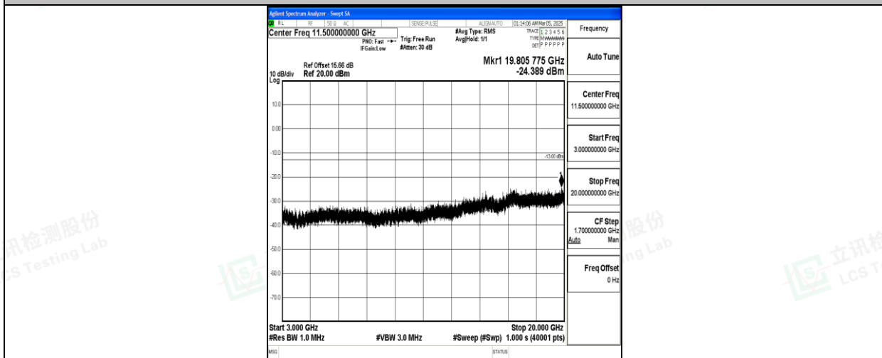
Band66_15MHz_QPSK_132322_1RB#0_3000~20000_3000~20000
