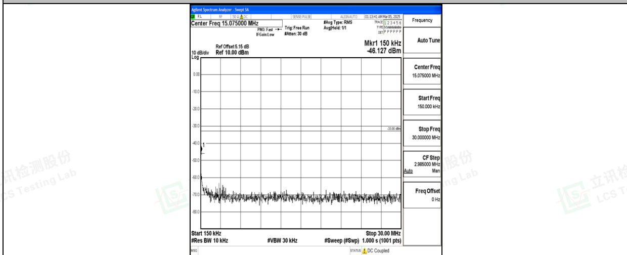
Band66_15MHz_QPSK_132322_1RB#0_0.15~30_0.15~30
