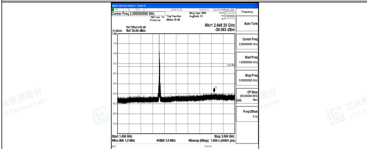
Band66_15MHz_16QAM_132047_1RB#0_1000~3000_1000~3000
