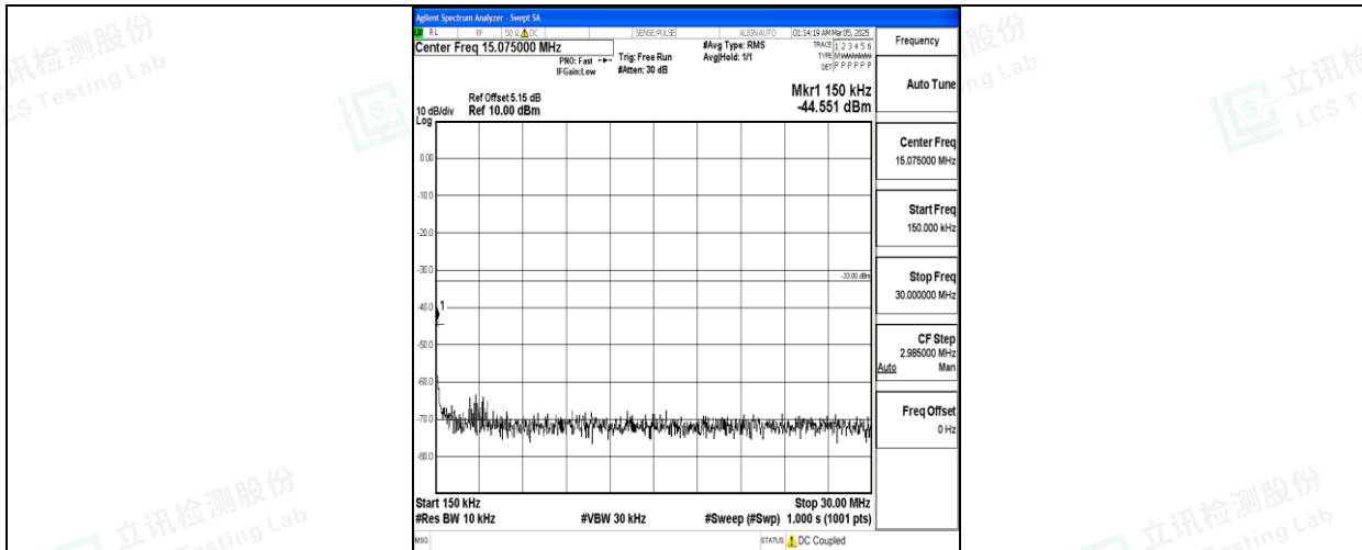
Band66_15MHz_16QAM_132322_1RB#0_0.15~30_0.15~30
