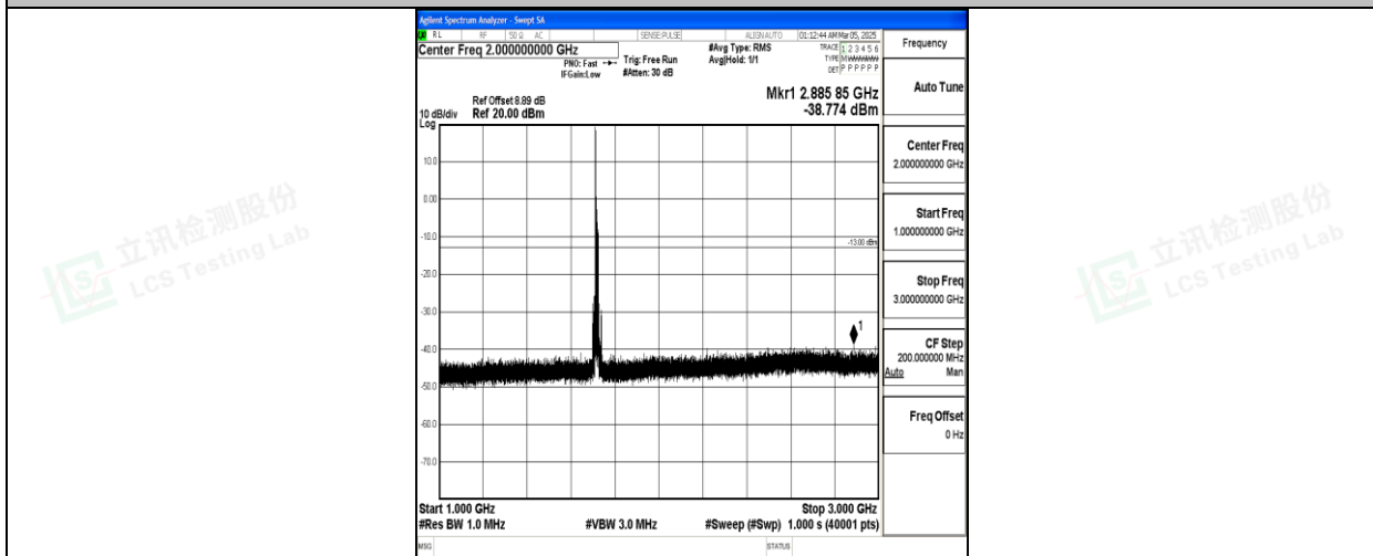
Band66_15MHz_QPSK_132047_1RB#0_1000~3000_1000~3000
