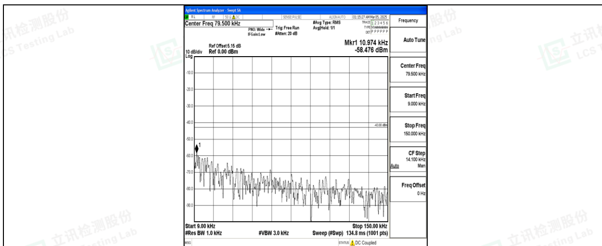
Band66_15MHz_16QAM_132597_1RB#0_0.009~0.15_0.009~0.15
