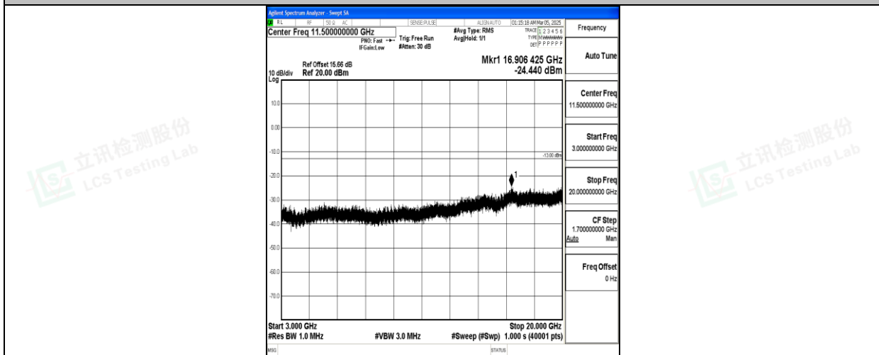
Band66_15MHz_QPSK_132597_1RB#0_3000~20000_3000~20000
