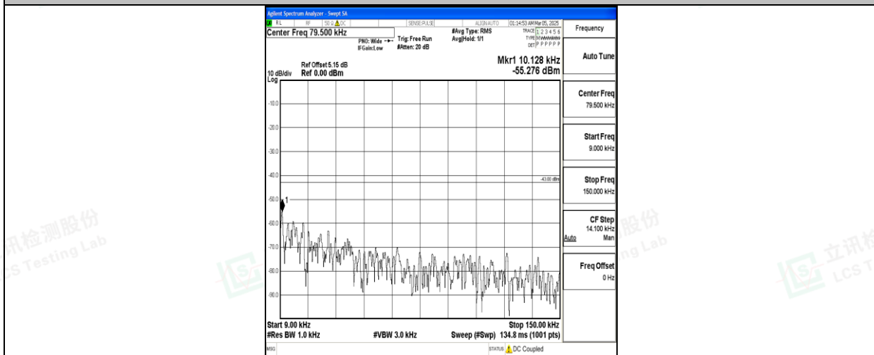
Band66_15MHz_QPSK_132597_1RB#0_0.009~0.15_0.009~0.15
