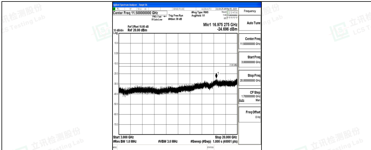
Band66_5MHz_QPSK_131997_1RB#0_3000~20000_3000~20000
