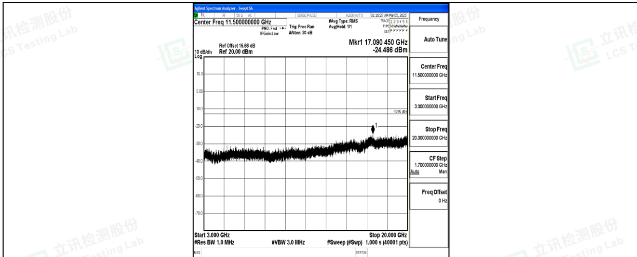
Band66_10MHz_16QAM_132322_1RB#0_3000~20000_3000~20000
