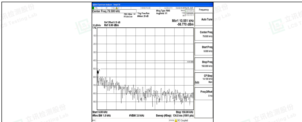
Band66_3MHz_16QAM_132657_1RB#0_0.009~0.15_0.009~0.15
