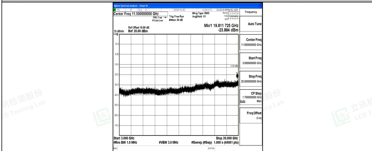
Band66_3MHz_16QAM_132657_1RB#0_3000~20000_3000~20000
