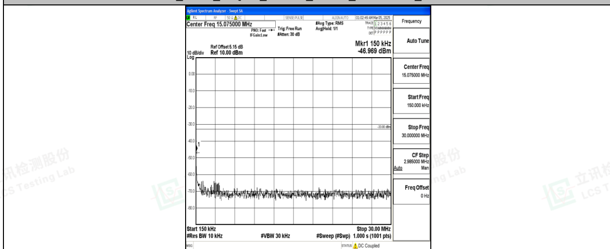
Band66_3MHz_16QAM_132657_1RB#0_0.15~30_0.15~30
