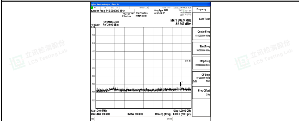
Band66_10MHz_16QAM_132622_1RB#0_30~1000_30~1000
