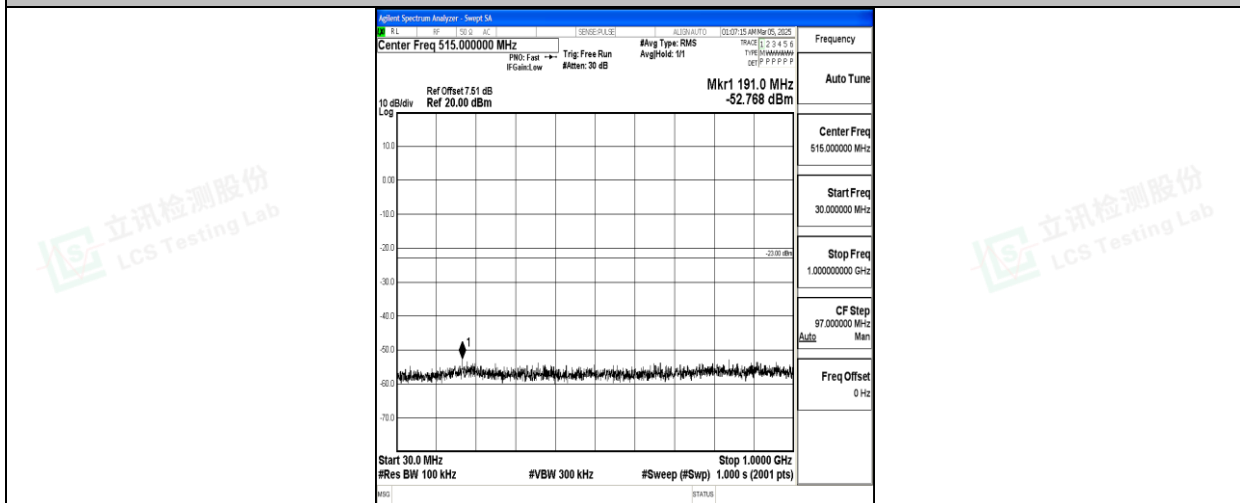
Band66_5MHz_16QAM_132647_1RB#0_30~1000_30~1000
