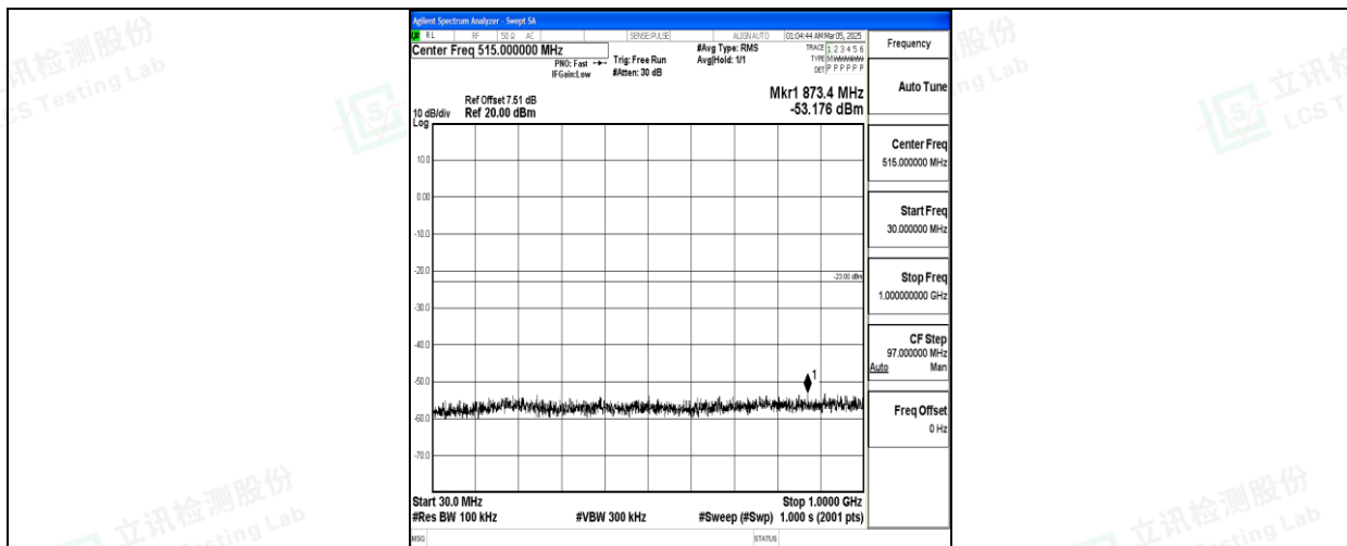
Band66_5MHz_16QAM_131997_1RB#0_30~1000_30~1000
