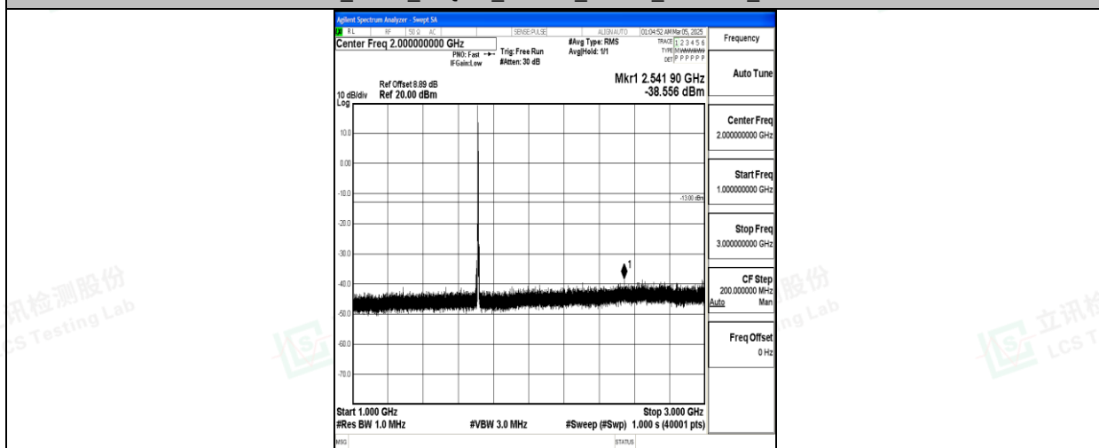
Band66_5MHz_16QAM_131997_1RB#0_1000~3000_1000~3000
