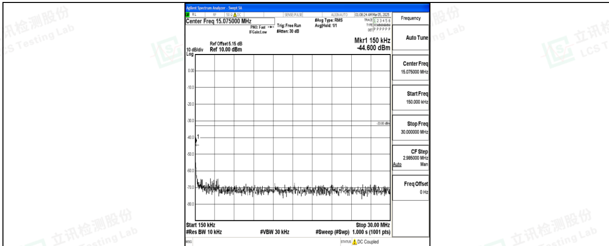
Band66_10MHz_QPSK_132022_1RB#0_0.15~30_0.15~30
