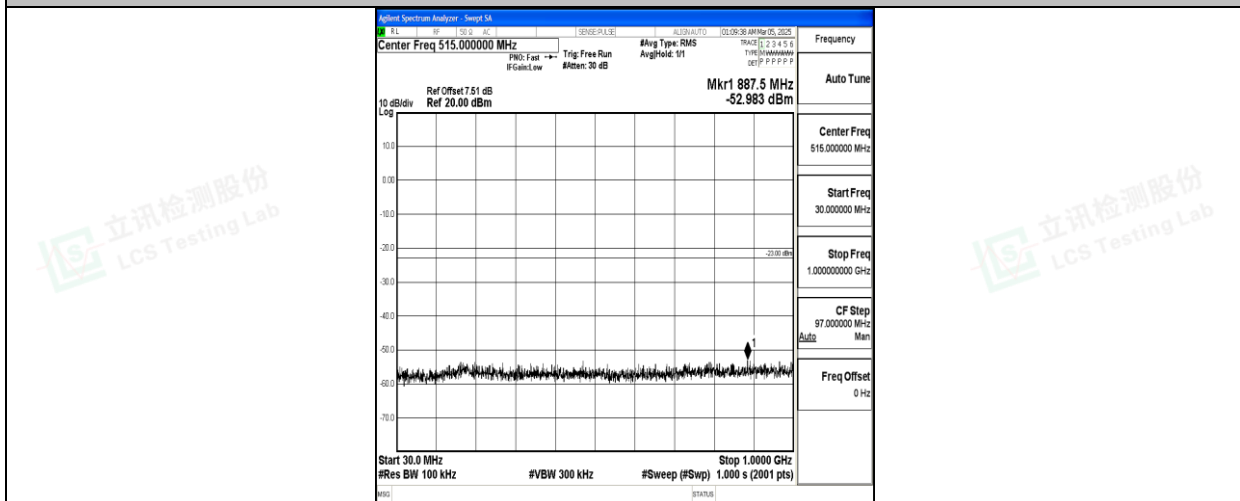
Band66_10MHz_QPSK_132322_1RB#0_30~1000_30~1000
