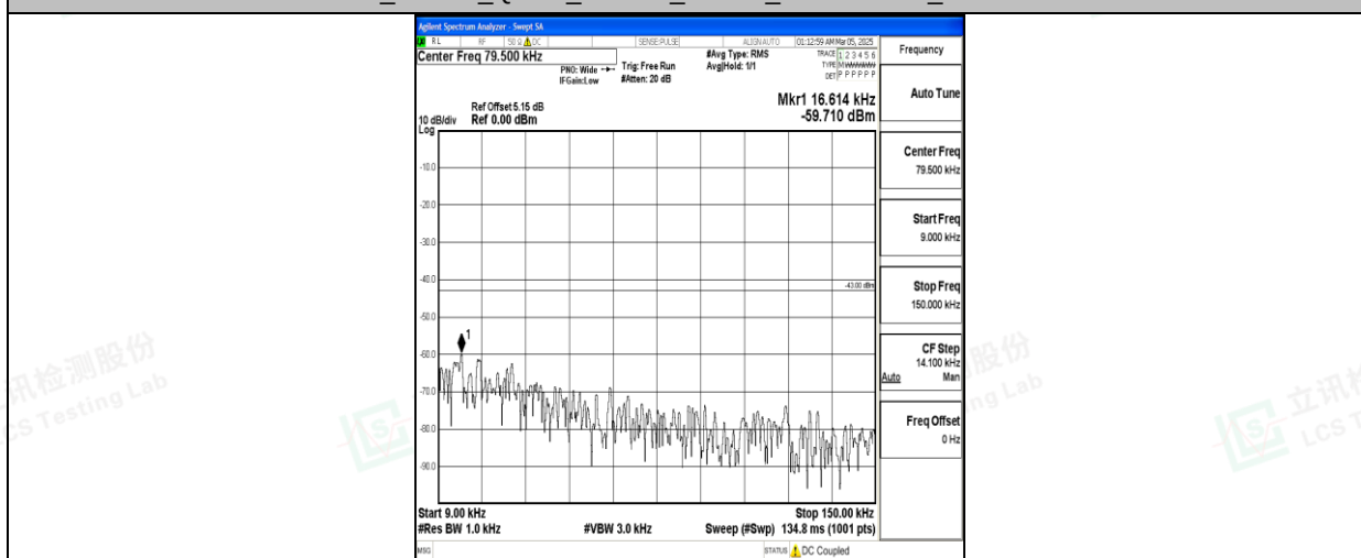
Band66 15MHz 16QAM 132047 1RB#0 0.009~0.15 0.009~0.15
