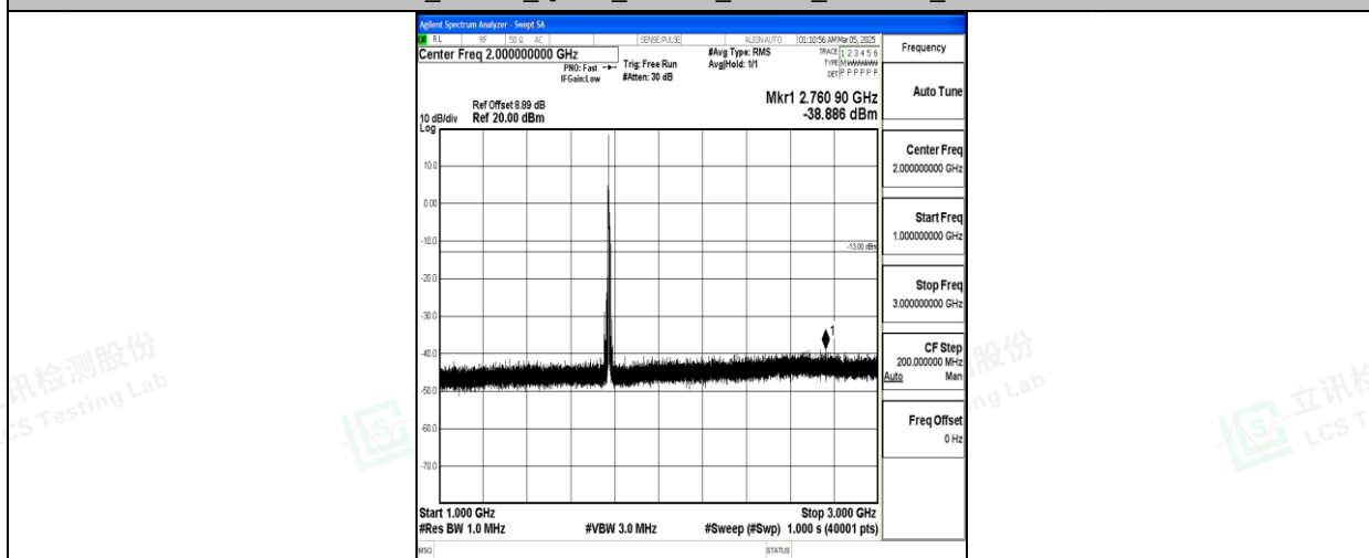
Band66_10MHz_QPSK_132622_1RB#0_1000~3000_1000~3000
