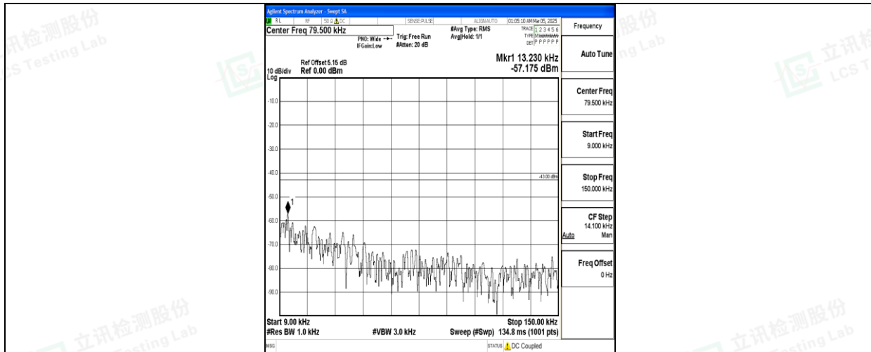
Band66_5MHz_QPSK_132322_1RB#0_0.009~0.15_0.009~0.15
