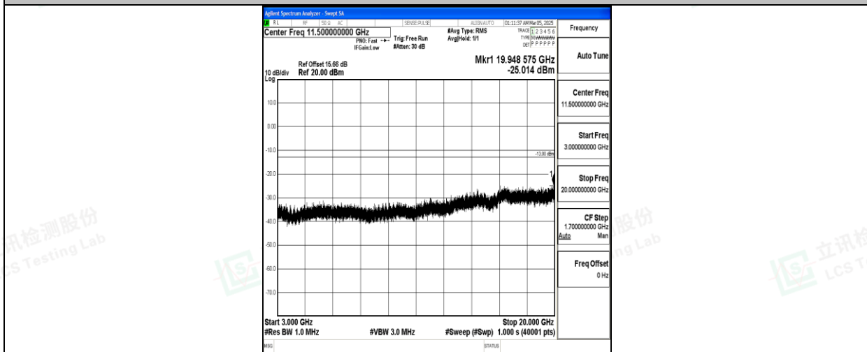
Band66_10MHz_16QAM_132622_1RB#0_3000~20000_3000~20000
