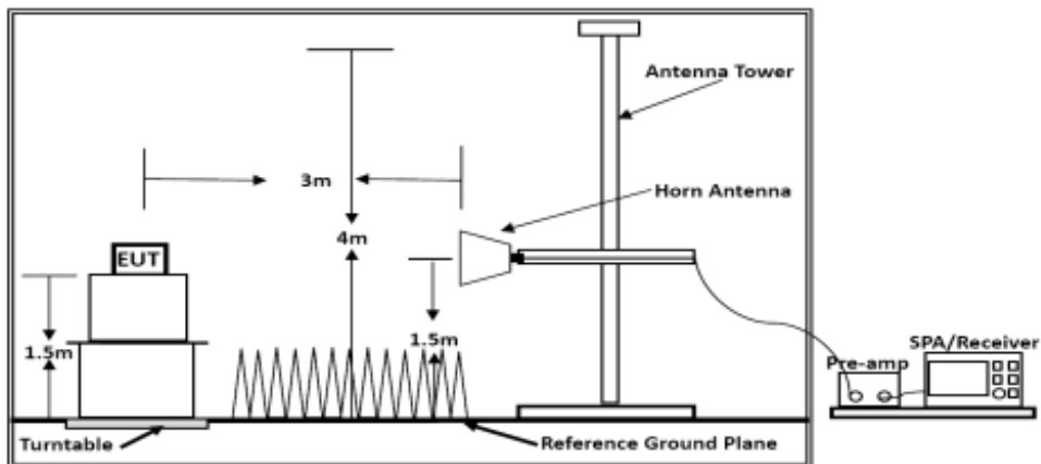
Above 1GHz
