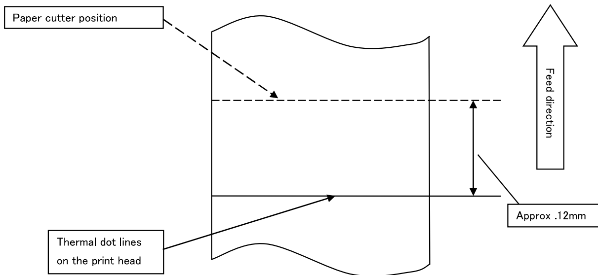
Print head and paper cutter position
