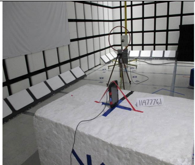
RADIATED BACK PHOTO (BELOW 30 MHz)
