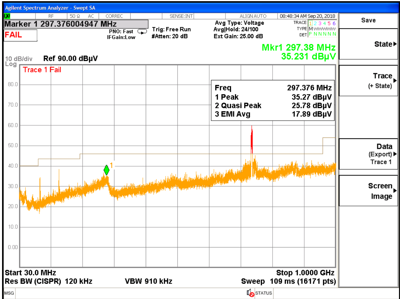
Figure 9. Ambient Vertical
