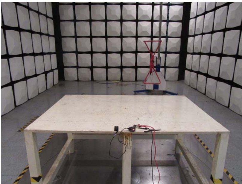
Field Strength Test Setup - Rear View
