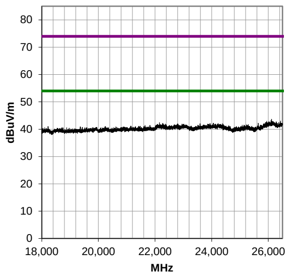
18000-26500 MHz, Run 18
