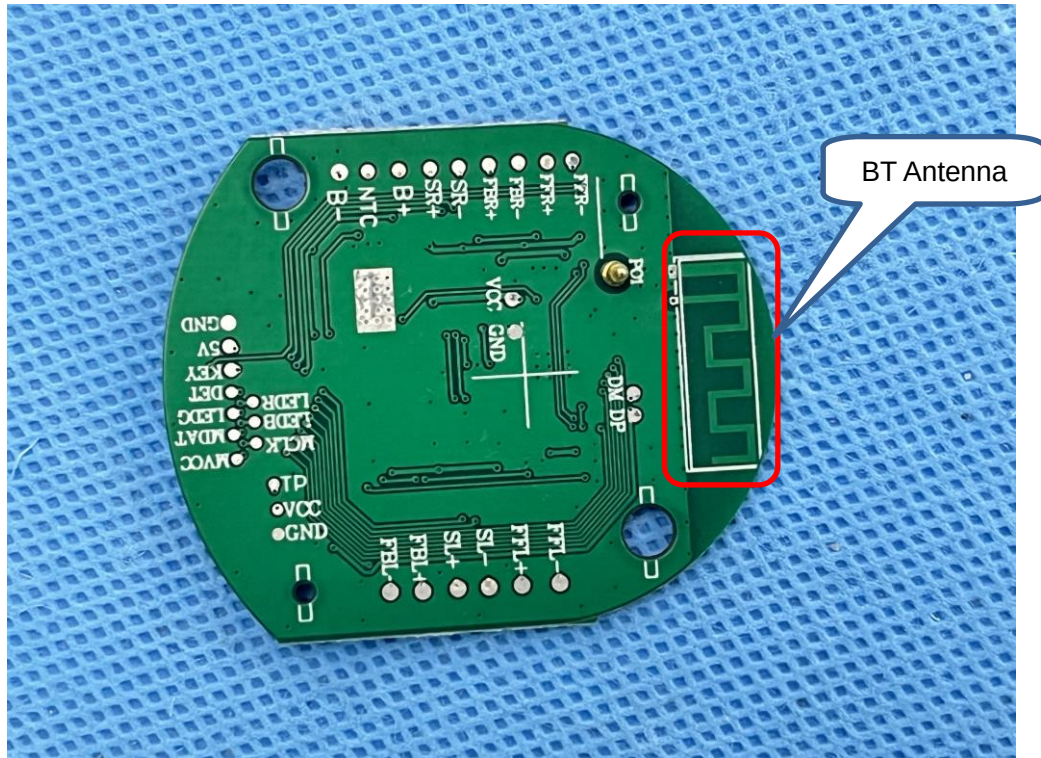
Internal view-10 of EUT
