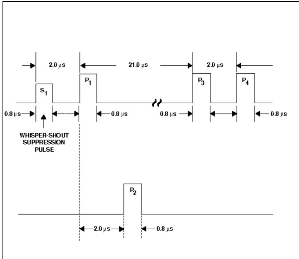
Mode A/C Only All Call Interrogation Pulse Sequence for TCAS (Mode A P_1 - P_3 is 8 \mu s )
