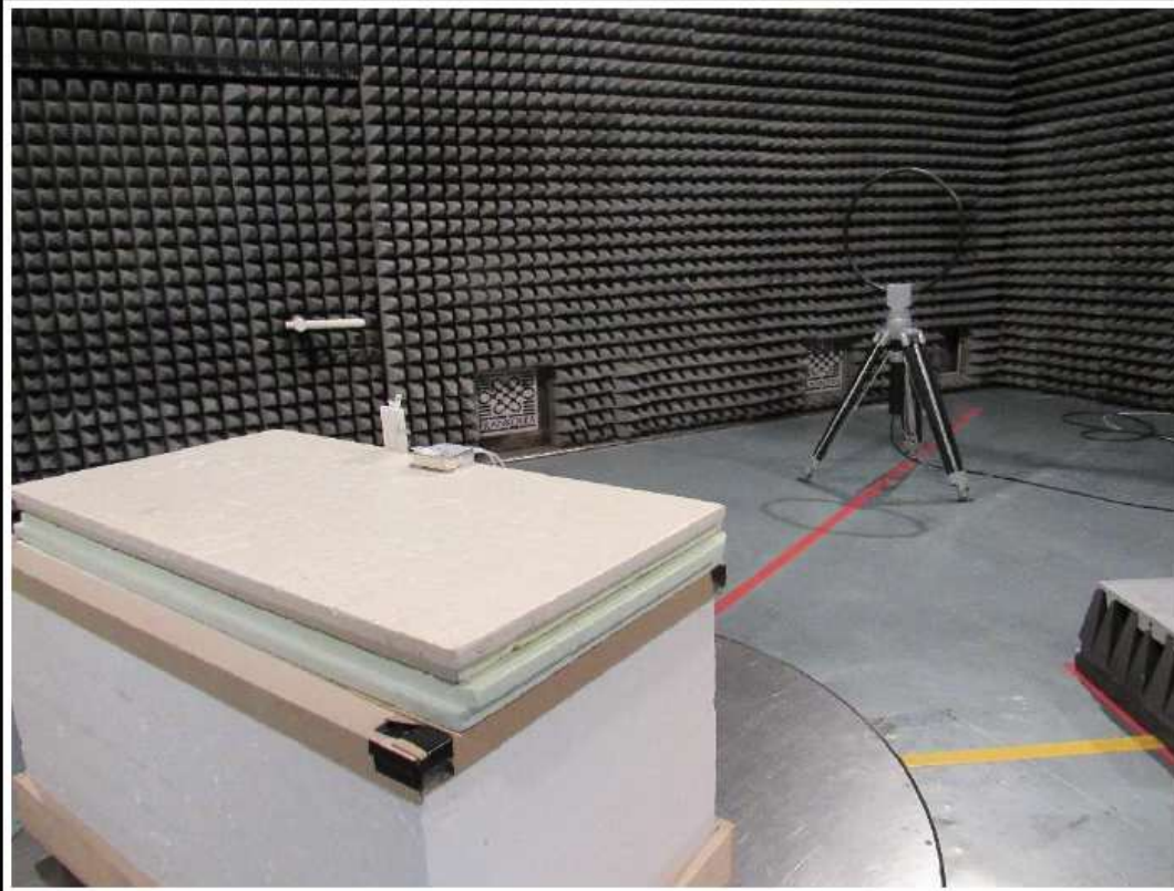
Test setup radiated below 30 MHz view 1
