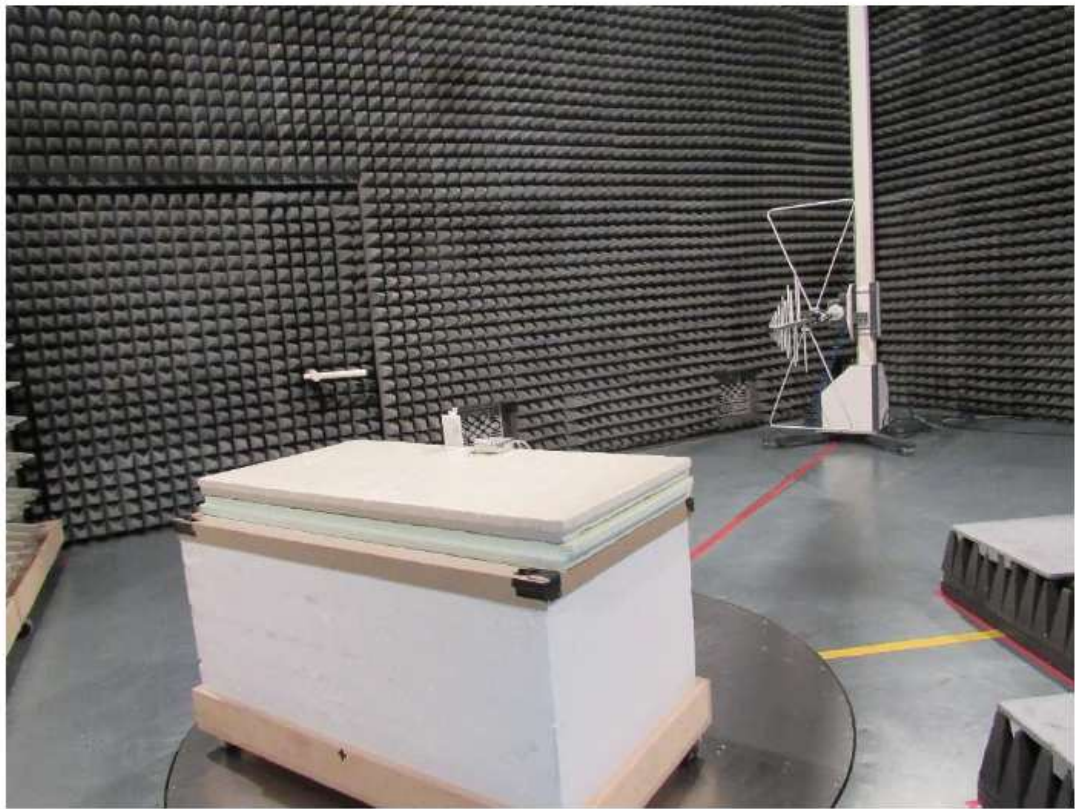
Test setup radiated above 30 MHz view 1
