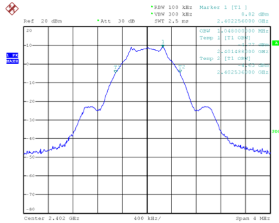
[99% Bandwidth]
