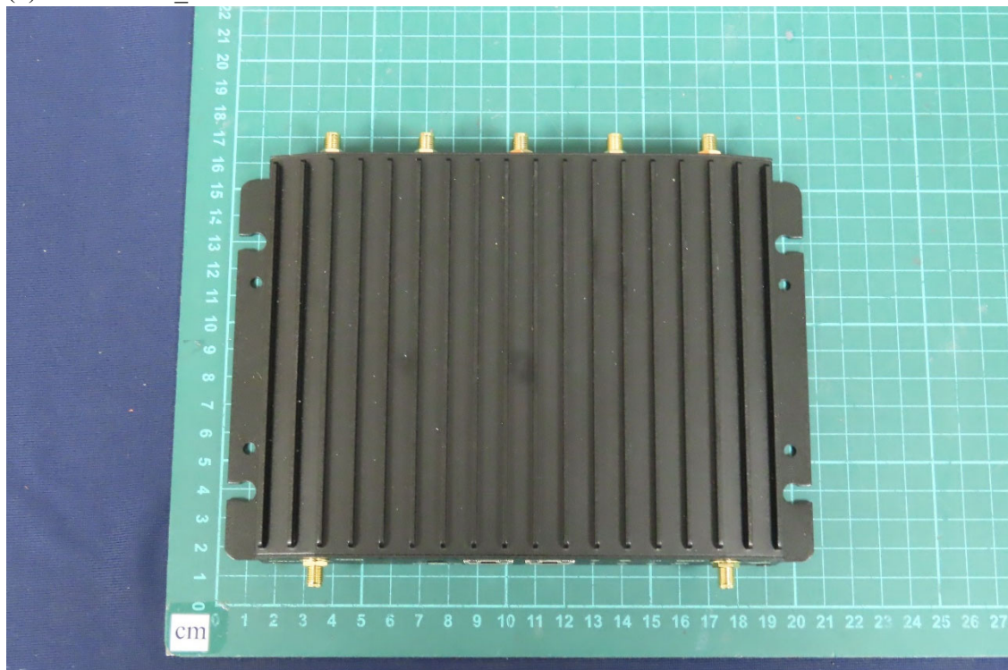
(7) EUT Photo _ Model: TLDPH01P1
