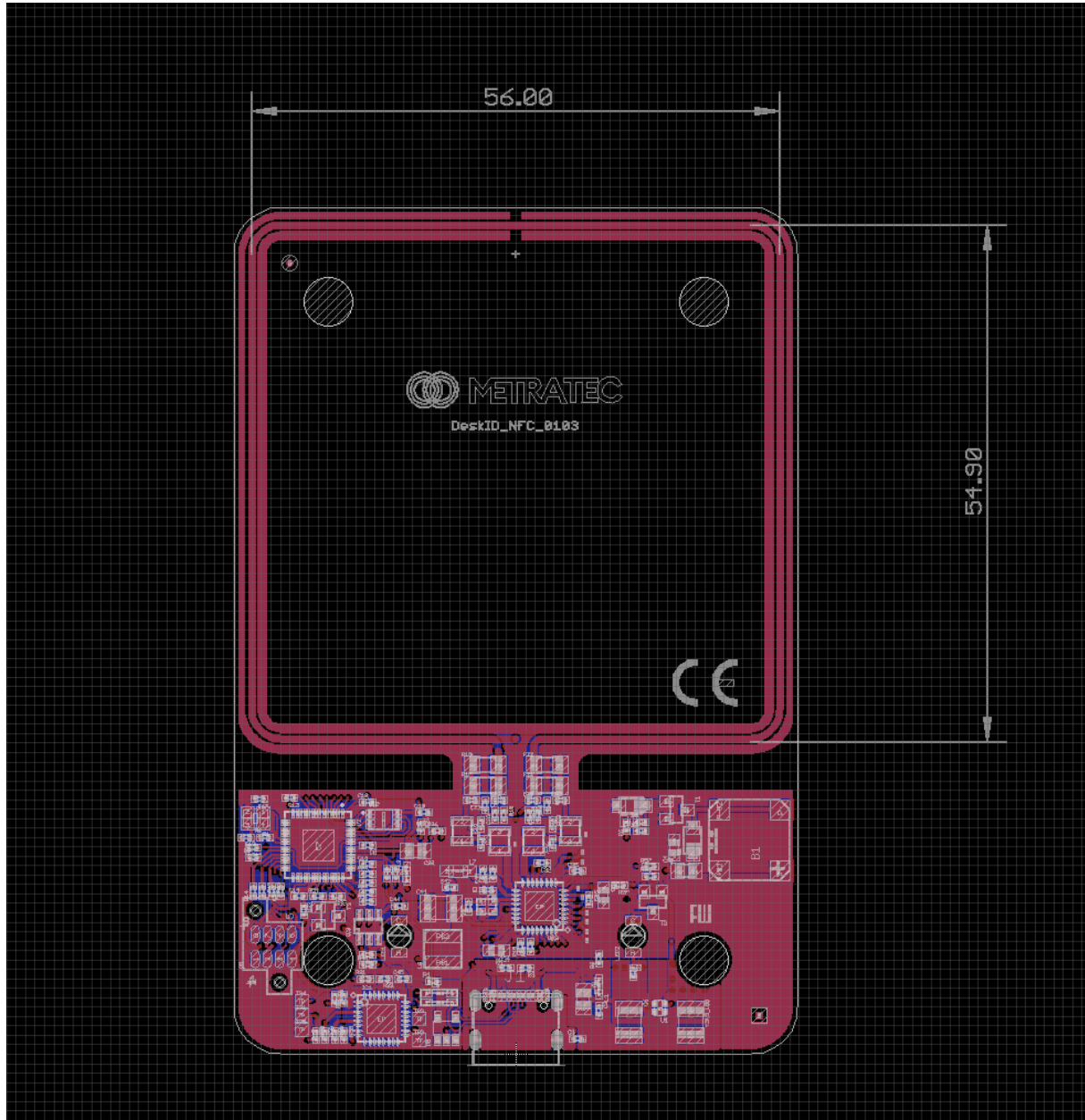
Fig. 1: Antenna Dimensions
