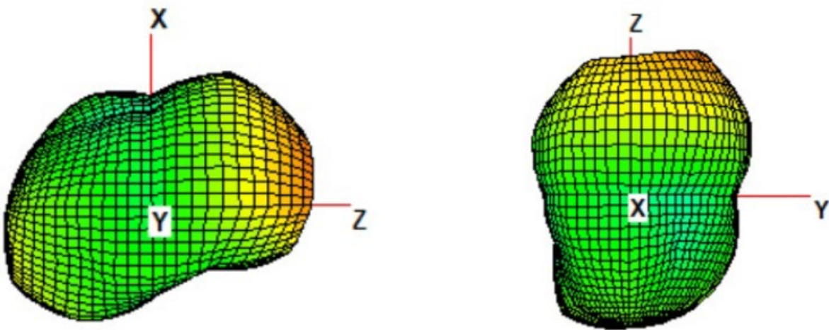
XZ plane at 1.575GHz
