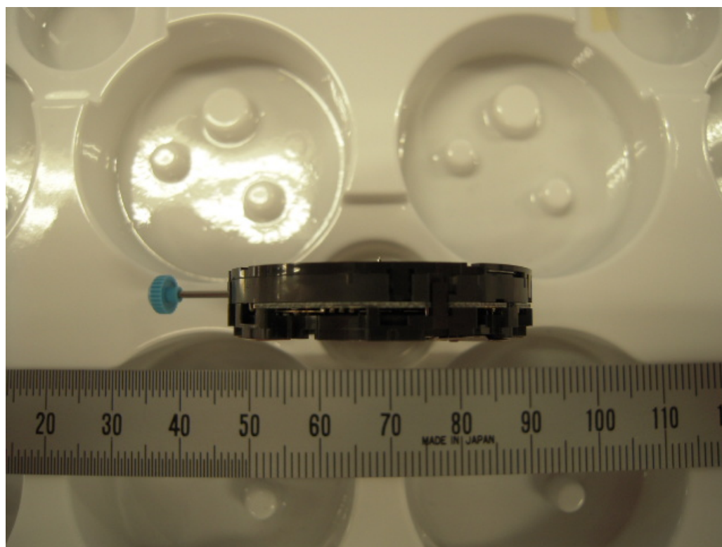
Side
