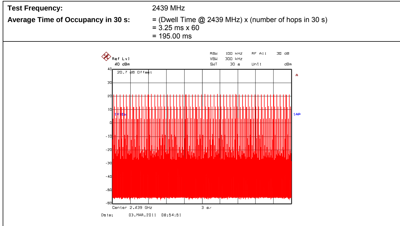
Plot 5.7.4.13. Time of Occupancy
