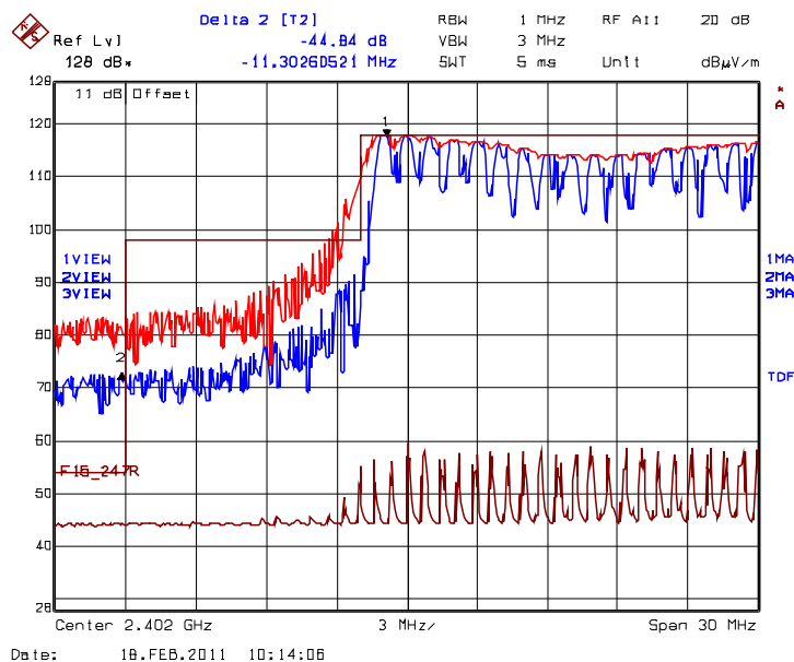
Plot 5.10.4.1.4. Band-Edge RF Radiated Emissions @ 3 m, Horizontal Rx Antenna Orientation Low End of Frequency Band, Pseudorandom Channel Hopping Mode
