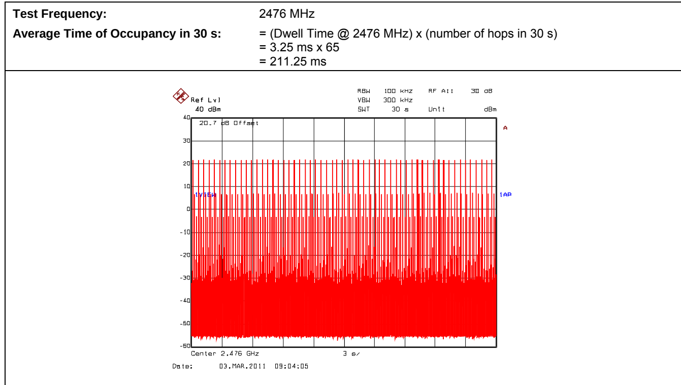
Plot 5.7.4.15. Time of Occupancy
