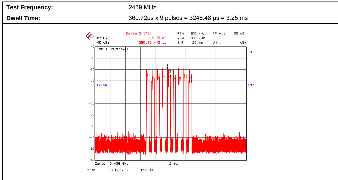
Plot 5.7.4.13. Time of Occupancy
