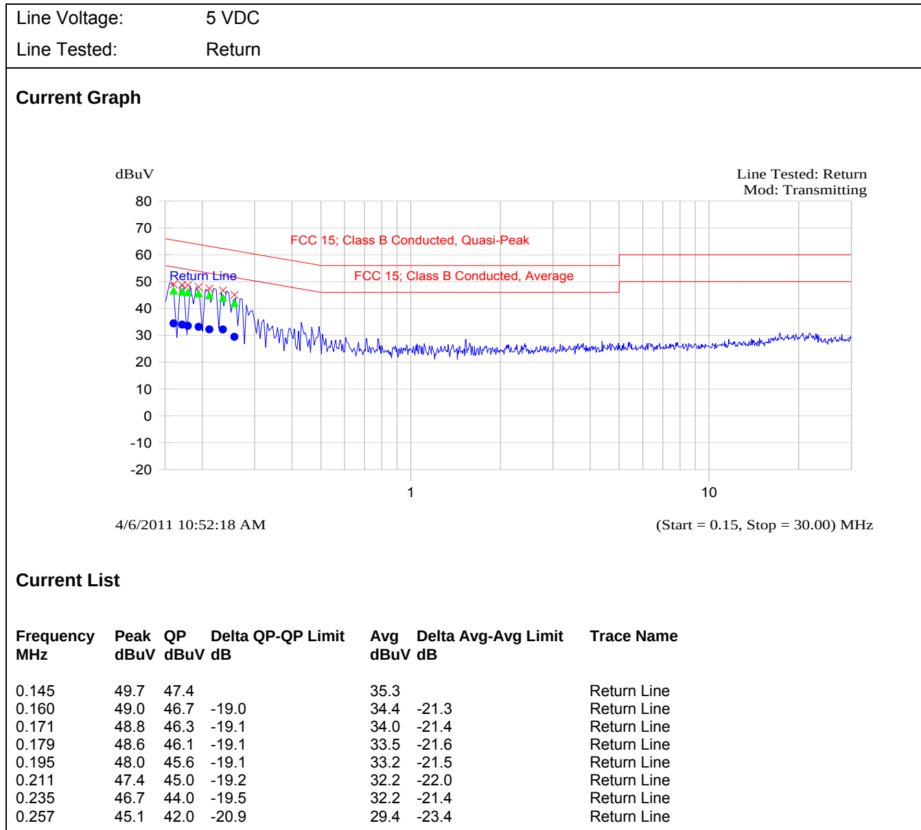
Plot 5.5.4.6. Power Line Conducted Emissions, 5 VDC Input, Tx Mode
