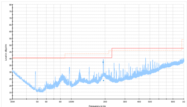
Figure 8.4-10: Radiated spurious emissions mid channel
