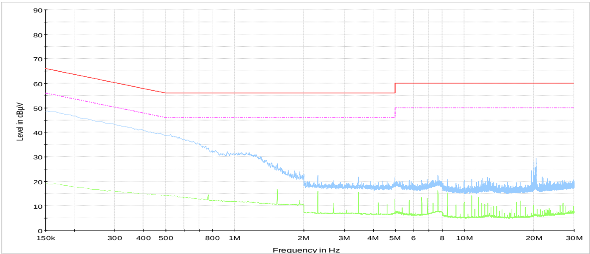
Plot 8.1-1: Conducted emissions on phase line
