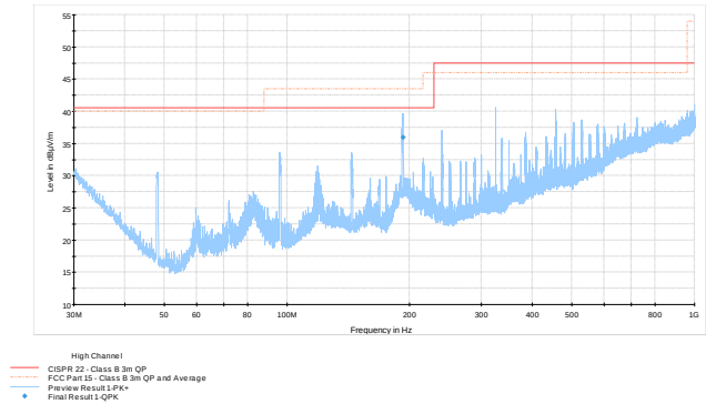
Figure 8.4-12: Radiated spurious emissions high channel
