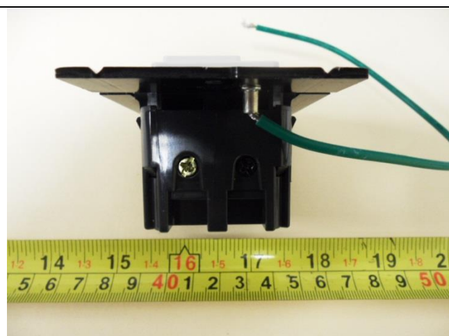
Host LC2102 – Bottom View
