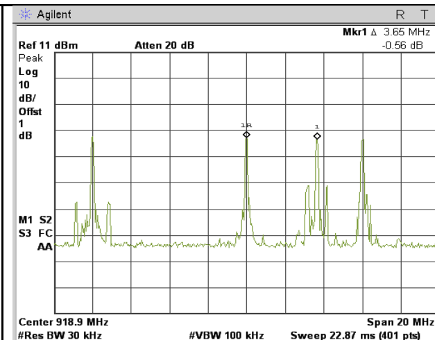
Channel Separation-Mid Channel
