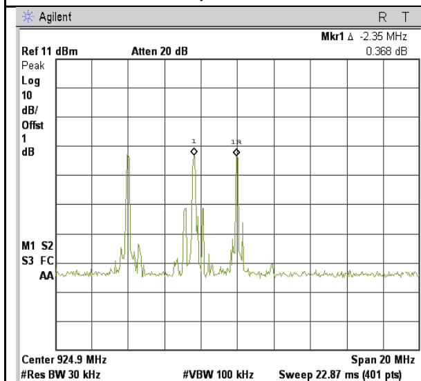
Channel Separation-High Channel
