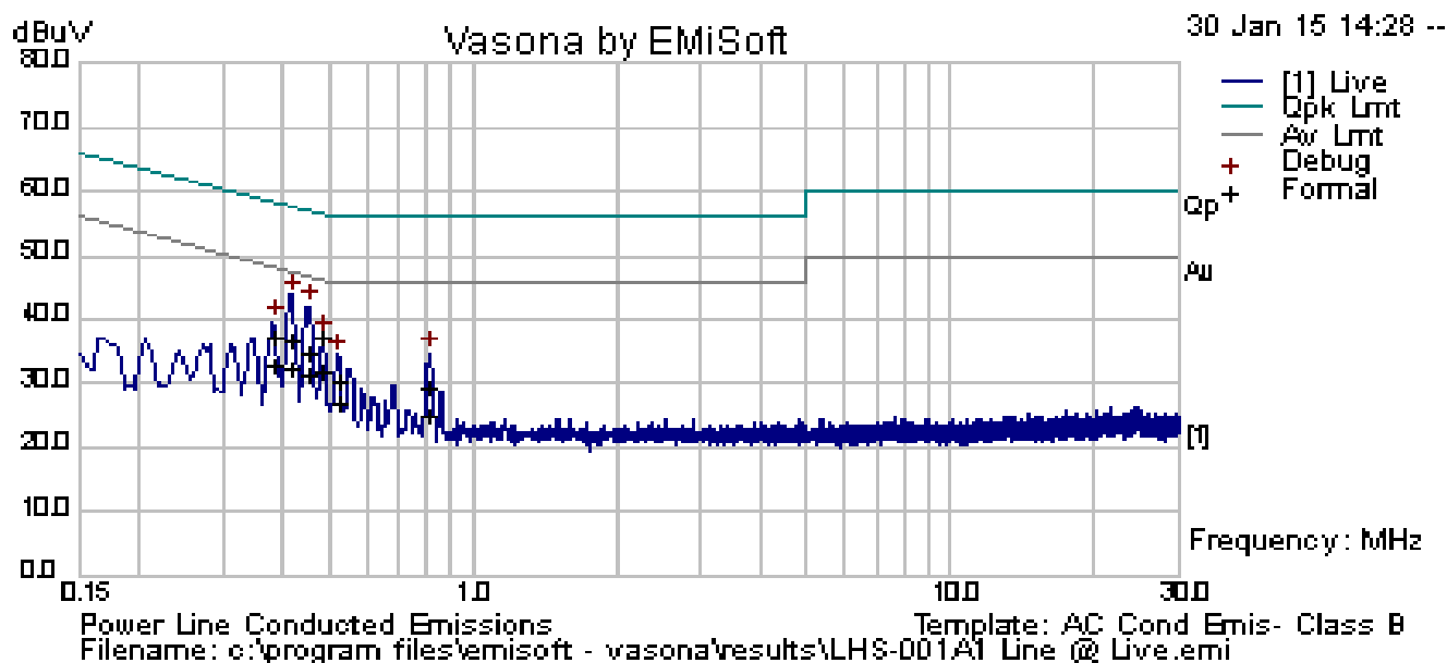
Line Plot at 120Vac, 60Hz
