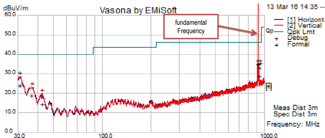
30MHz – 1000MHz at 3 meters
