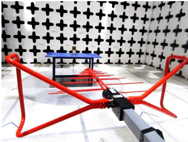
EUT Radiated Emissions (<1GHz) – Front View
