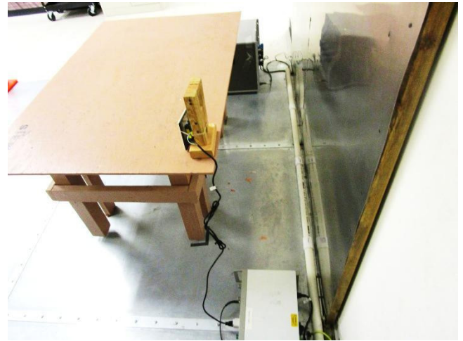
EUT AC Conducted Emission – Rear View
