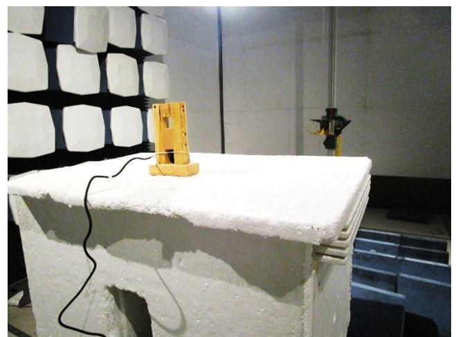
EUT Radiated Emissions (>1GHz) – Rear View
