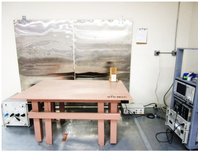
EUT AC Conducted Emission – Front View
