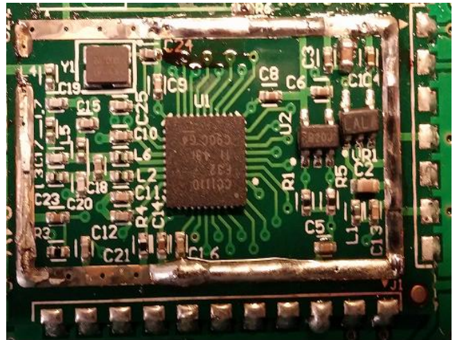
RFID Module Without Shielding
