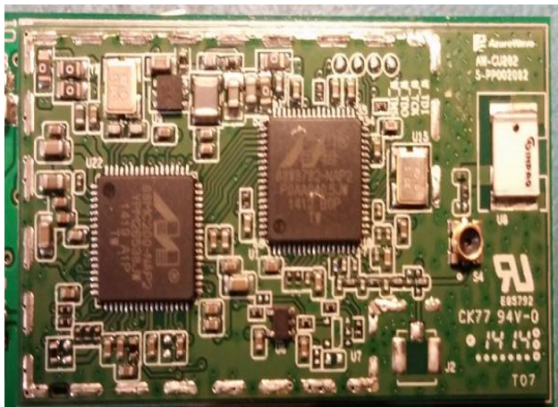
WLAN Module Without Shielding
