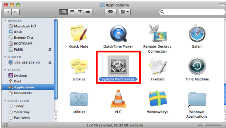
Figure 5-14 System Preferences
