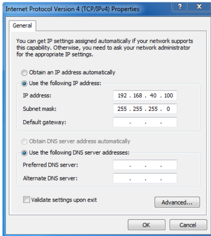
Figure 3-1 TCP/IP Setting
