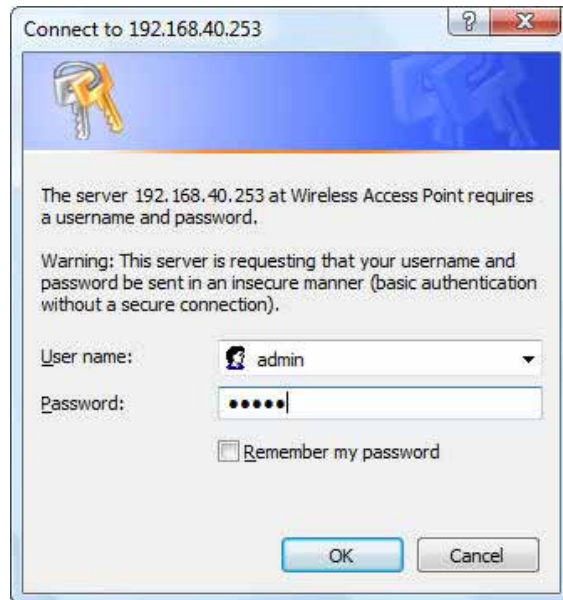
Figure 3-6 Login Window
