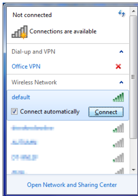
Figure 5-6 WLAN AutoConfig
