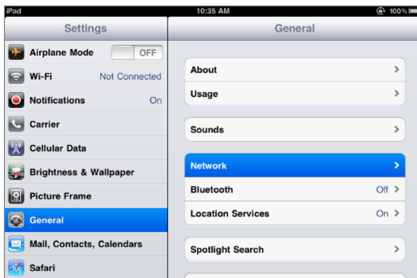
Figure 5-18 Wi-Fi Setting
