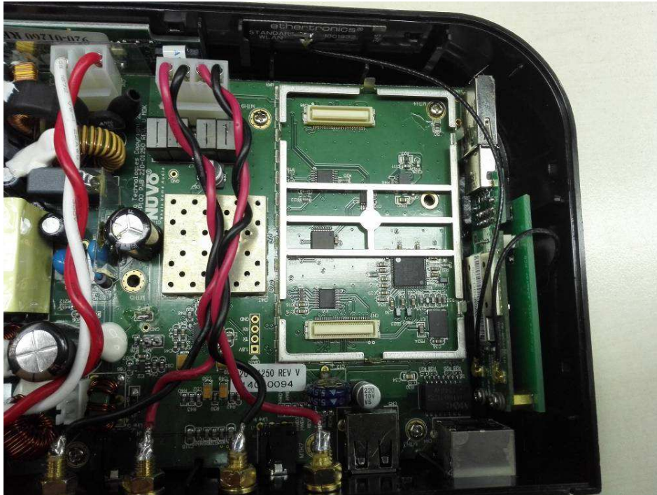
Antenna Position
