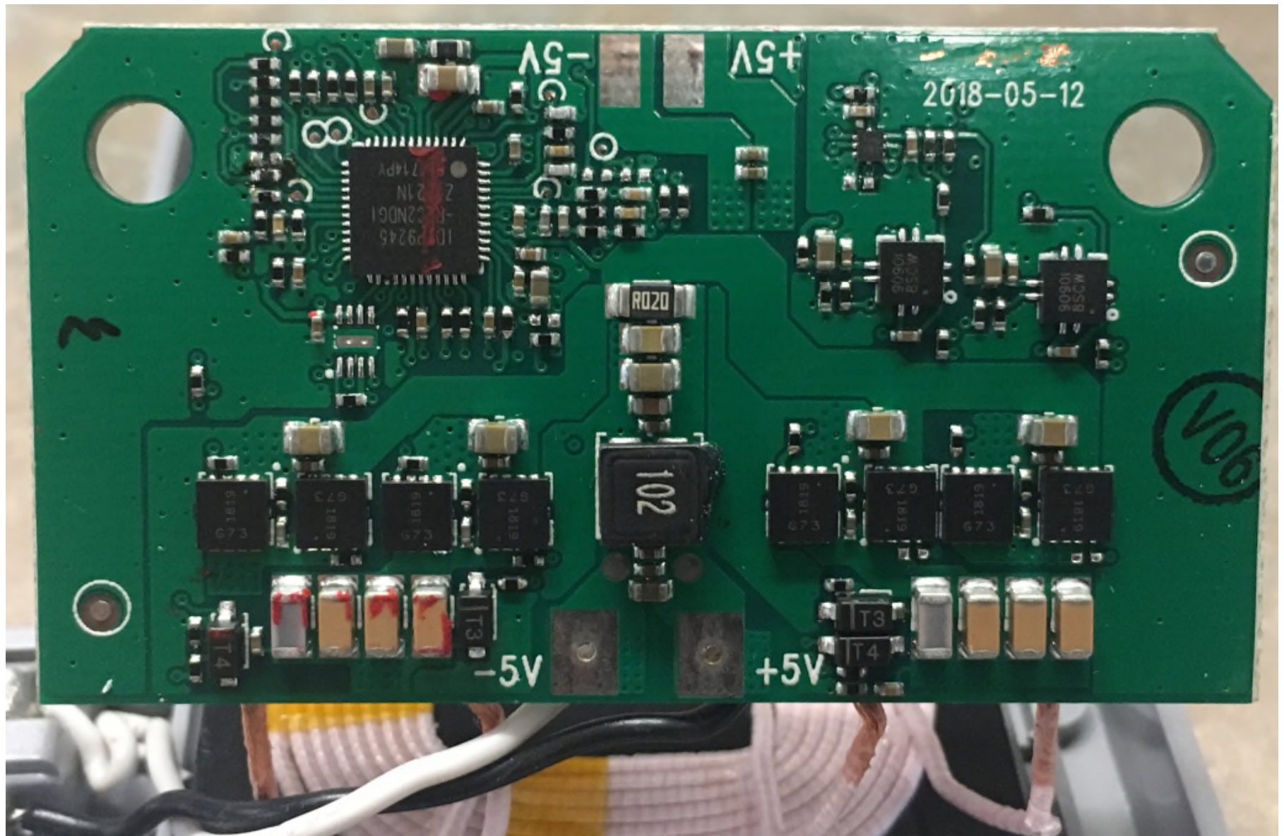
RWC826USB Wireless Charger PCB Component Side Photo
