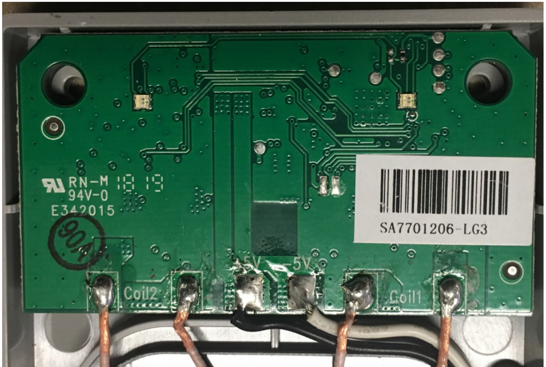
RWC826USB Wireless Charger PCB Top Side Photo
