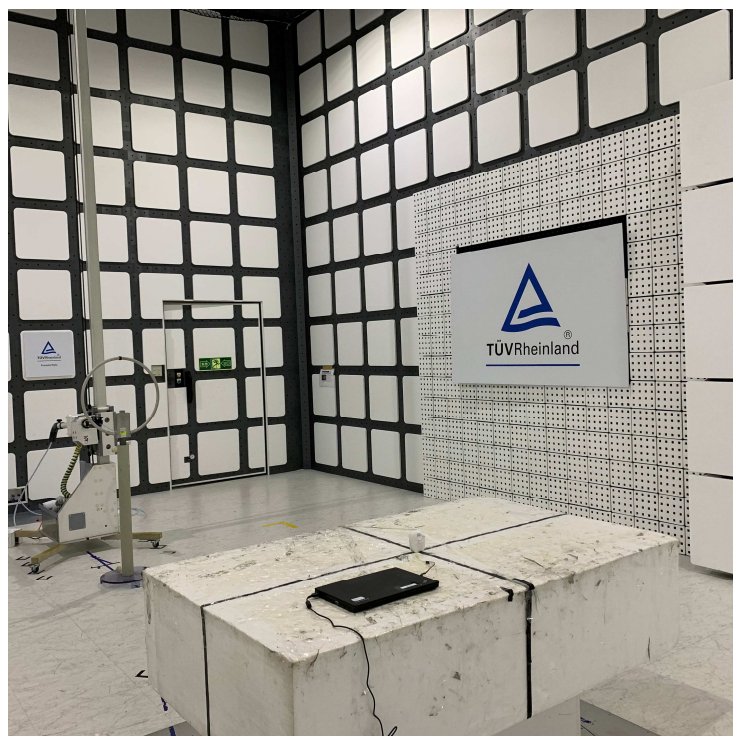
Photograph 2: Set-up for Spurious Emissions (Back View 1)
