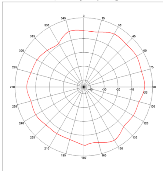
Far-field Power Distribution on X-Z Plane Gain= -0.17 dBi; Total Radiating Efficiency: 45.86% @2.45000 GHz
