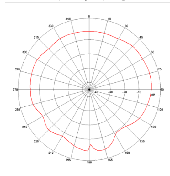
Far-field Power Distribution on Y-Z Plane Gain= -0.17 dBi; Total Radiating Efficiency: 45.86% @2.45000 GHz
