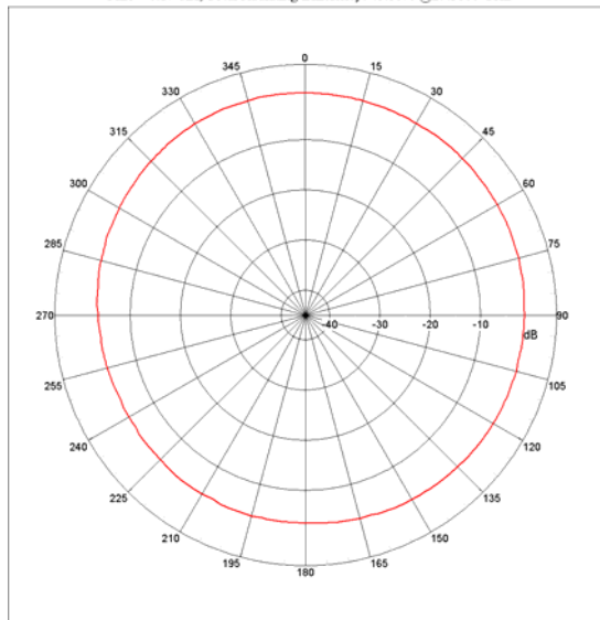
Far-field Power Distribution on X-Y Plane Gain= -0.17 dBi; Total Radiating Efficiency: 45.86% @2.45000 GHz
