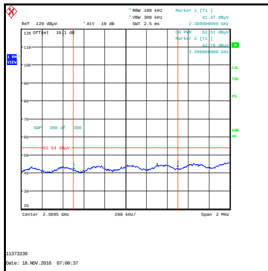
2310 MHz to 2390 MHz Restricted Band Average Measurement / Integrated level
