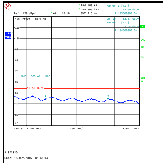
Upper Band Edge Average Measurement / Integrated level
