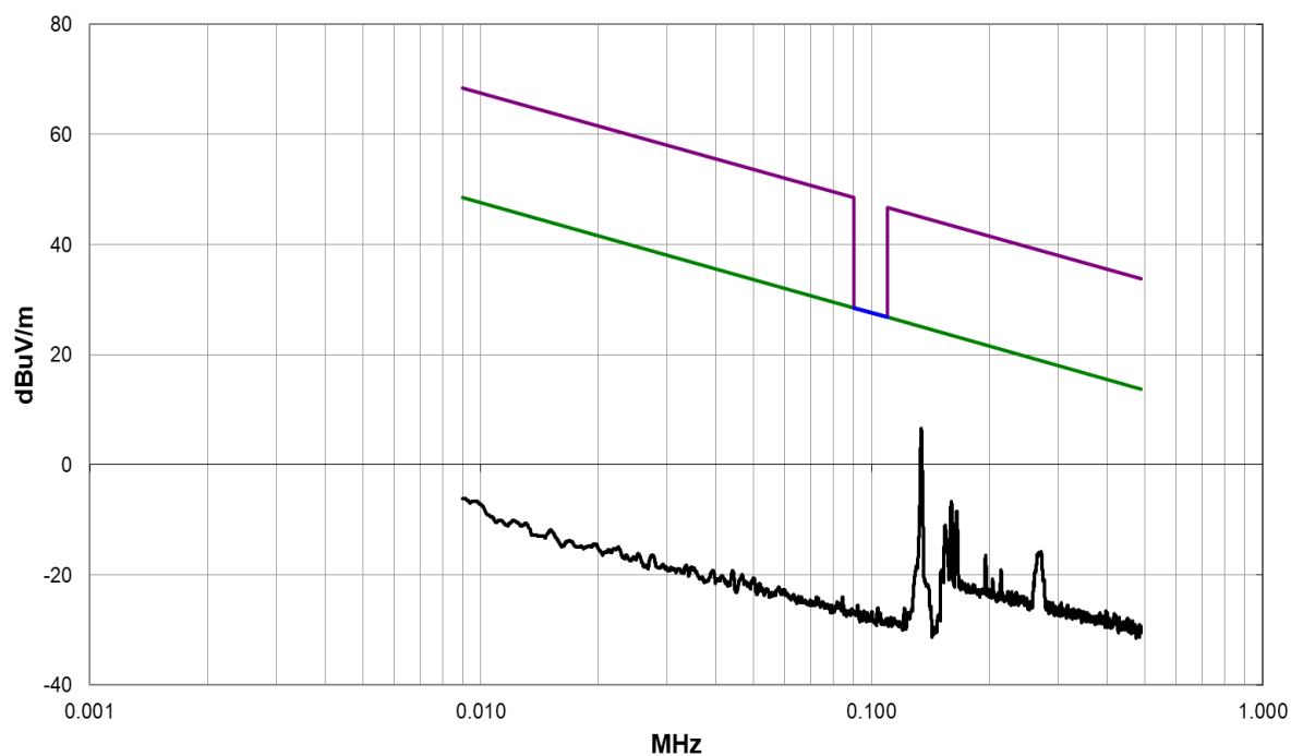
9 kHz to 490 kHz Scan
