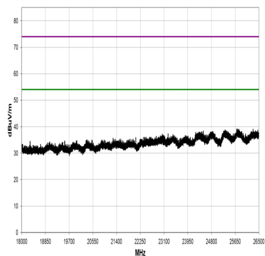
18 GHz to 26.5 GHz
