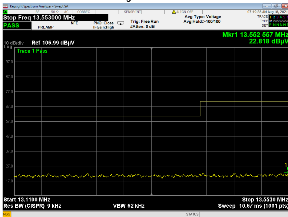
Figure 6 – Lower Band-edge
