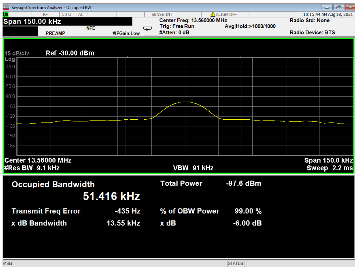
Figure 3 - 99% Occupied Bandwidth, NFC, 1m Test Distance
