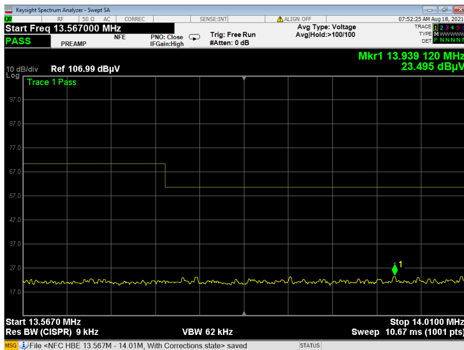
Figure 7 – Higher Band-edge
