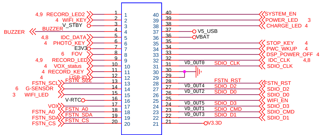
CN1 CON_40P-0.5-F
