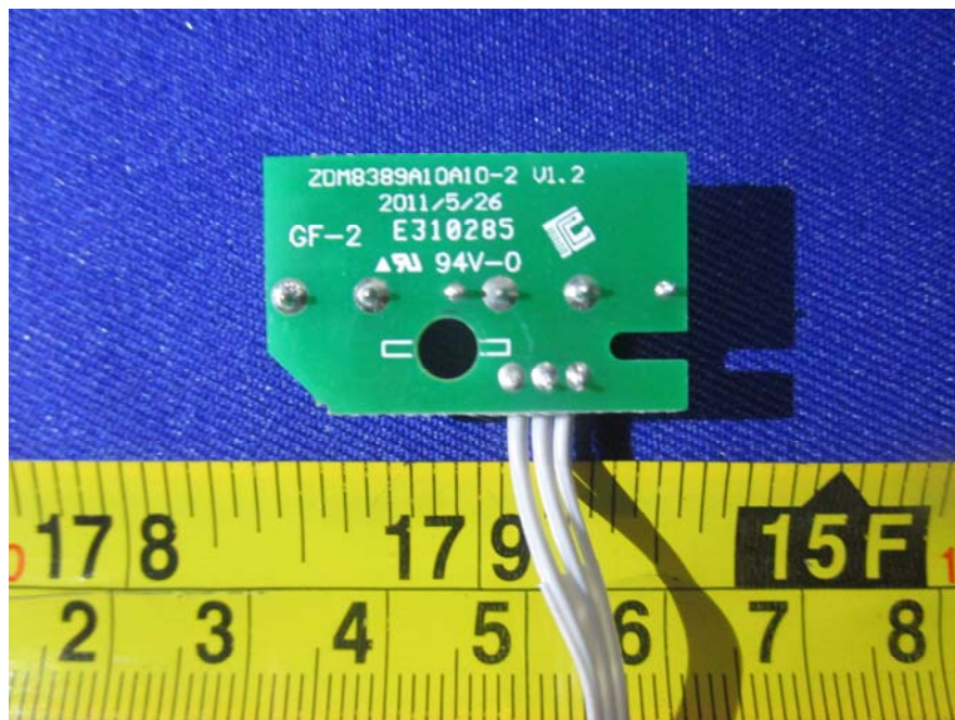
EUT –Key PCB Top View
