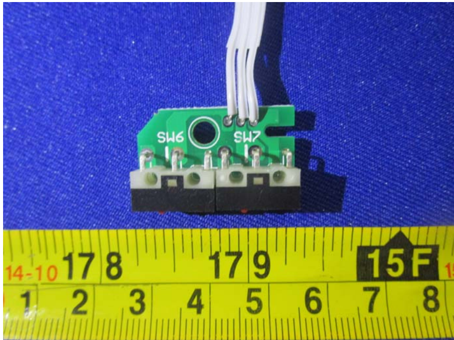
EUT –Key PCB Bottom View
