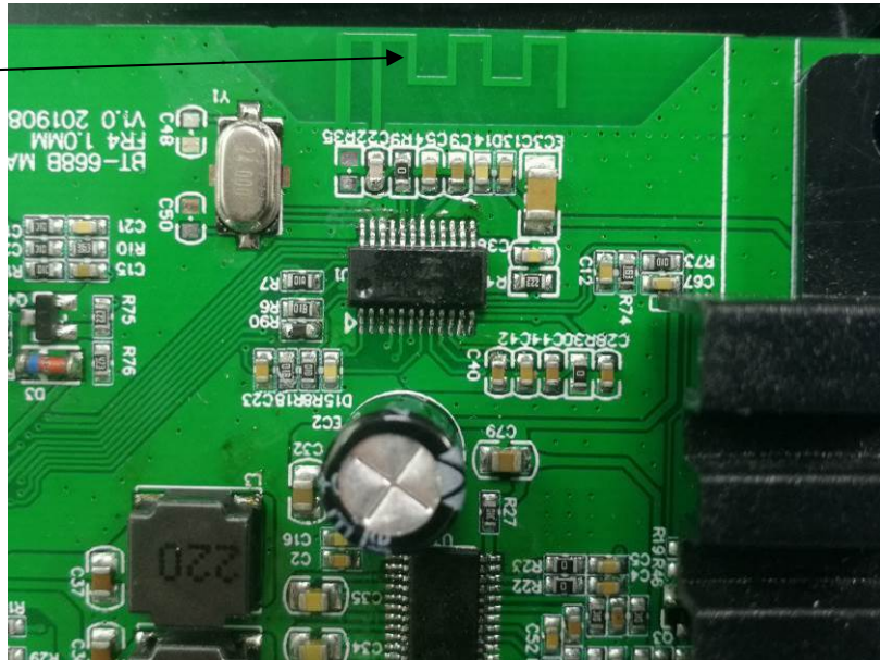
PCB ANTENNA
