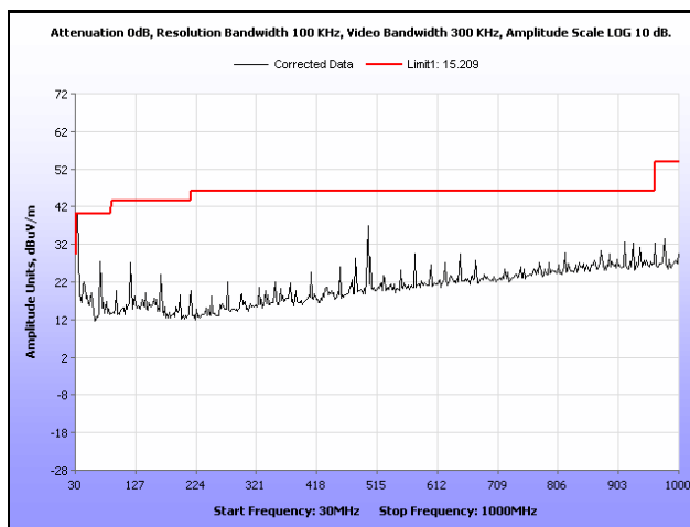
Plot 45. Radiated Spurious Emissions, Mid Channel, 802.11n, 30 MHz – 1 GHz
