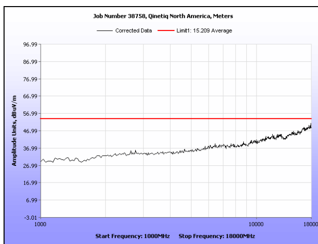
Plot 44. Radiated Spurious Emissions, Low Channel, 802.11n, 1 GHz – 18 GHz, Peak under Average
