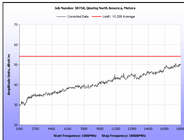
Plot 32. Radiated Spurious Emissions, Low Channel, 802.11b, 1 GHz – 18 GHz, Peak under Average
