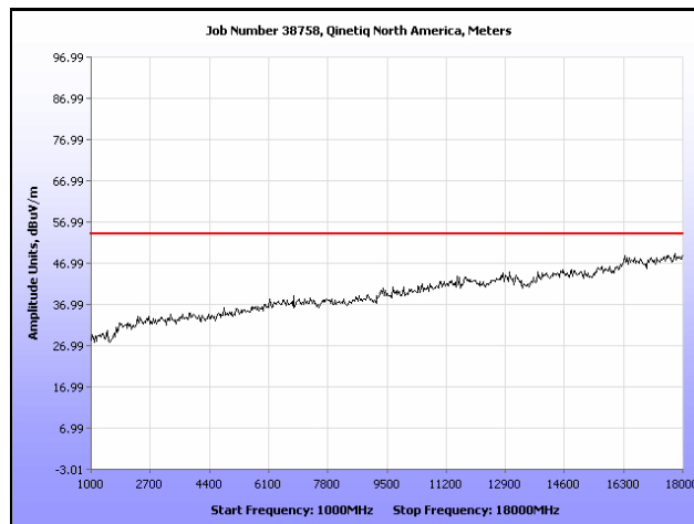
Plot 36. Radiated Spurious Emissions, High Channel, 802.11b, 1 GHz – 18 GHz, Peak under Average
