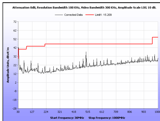
Plot 39. Radiated Spurious Emissions, Mid Channel, 802.11g, 30 MHz – 1 GHz
