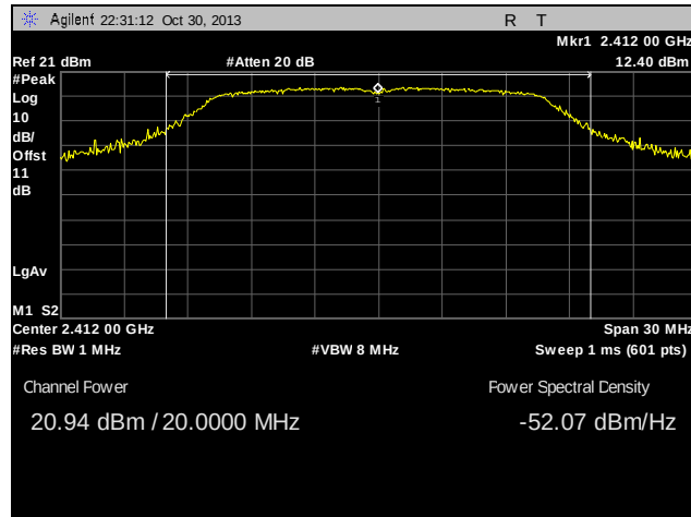
Plot 24. Peak Power Output, Low Channel, 802.11g
