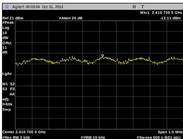
Plot 77. Peak Power Spectral Density, Low Channel, 802.11n
