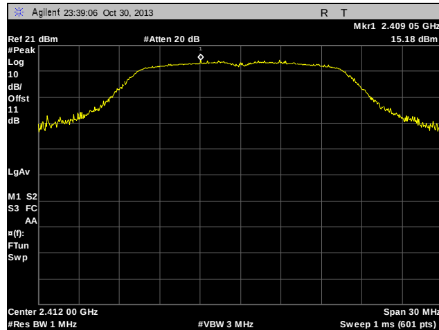
Plot 70. Peak Power Spectral Density, Determination, Low Channel, 802.11g
