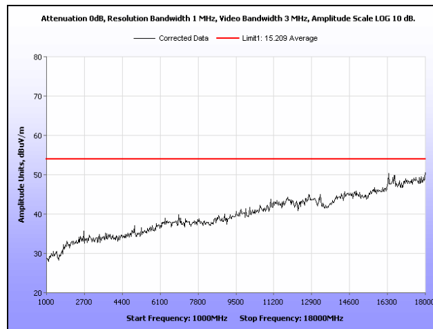
Plot 38. Radiated Spurious Emissions, Low Channel, 802.11g, 1 GHz – 18 GHz, Peak under Average
