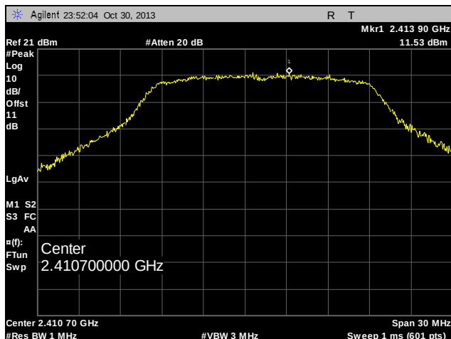
Plot 76. Peak Power Spectral Density, Determination, Low Channel, 802.11n
