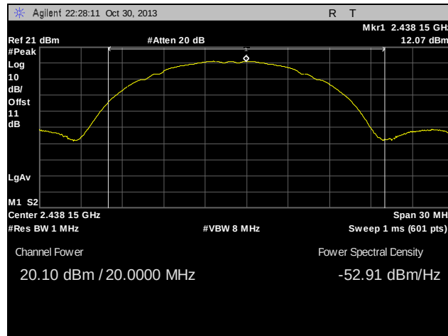
Plot 22. Peak Power Output, Mid Channel, 802.11b
