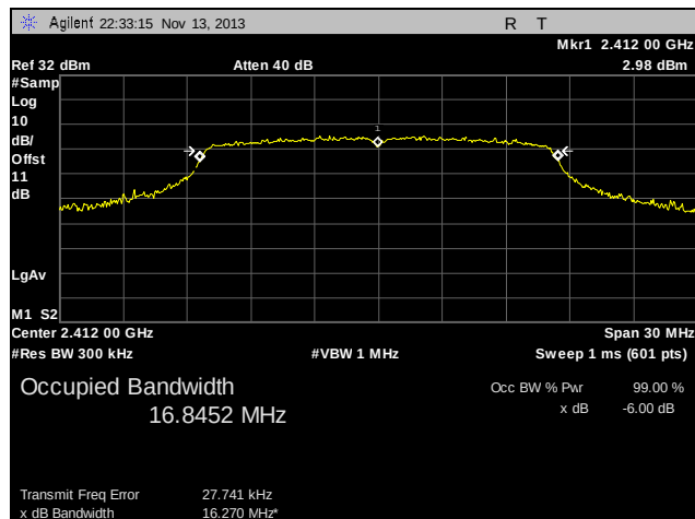
Plot 15. 99% Occupied Bandwidth, Low Channel, 802.11g
