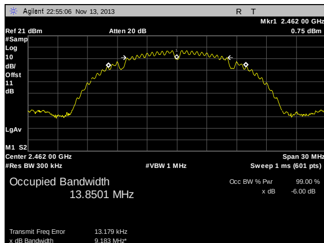
Plot 14. 99% Occupied Bandwidth, High Channel, 802.11b
