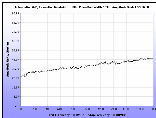
Plot 42. Radiated Spurious Emissions, High Channel, 802.11g, 1 GHz – 18 GHz, Peak under Average
