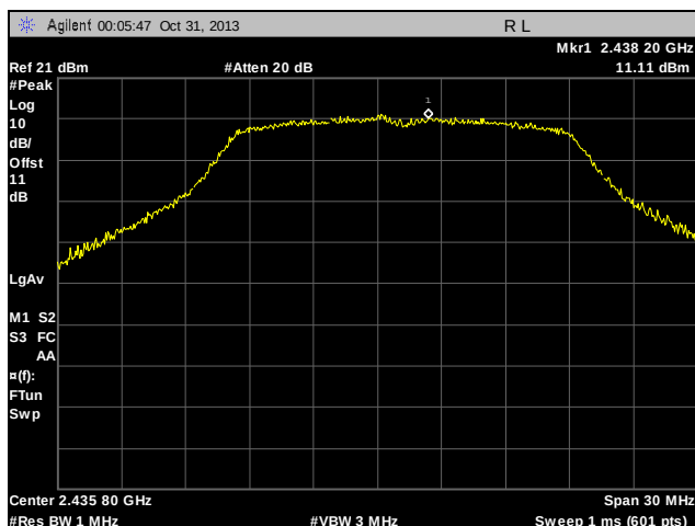
Plot 78. Peak Power Spectral Density, Determination, Mid Channel, 802.11n
