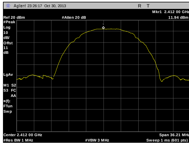
Plot 64. Peak Power Spectral Density, Determination, Low Channel, 802.11b
