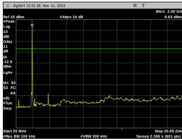
Plot 55. Conducted Spurious Emissions, Low Channel, 802.11b
