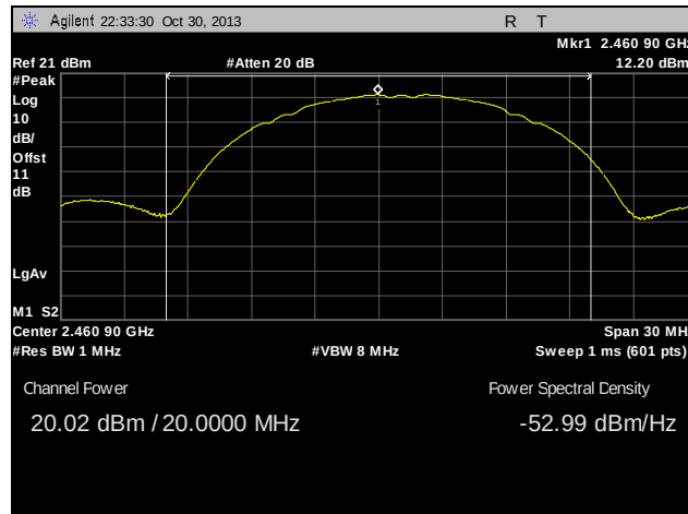
Plot 23. Peak Power Output, High Channel, 802.11b
