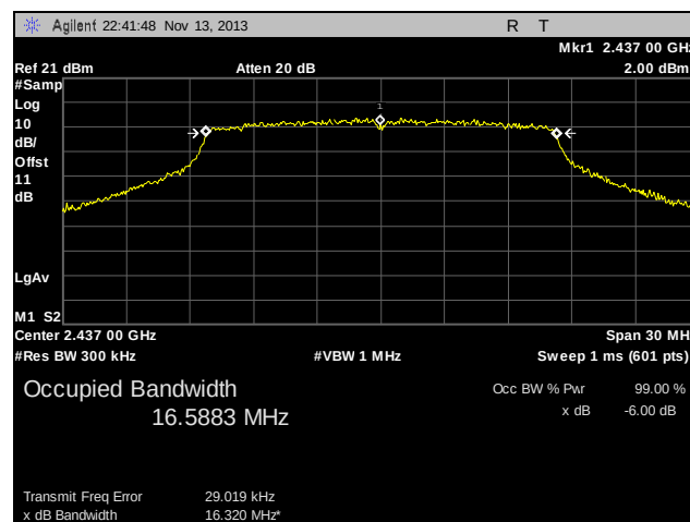
Plot 19. 99% Occupied Bandwidth, Mid Channel, 802.11n
