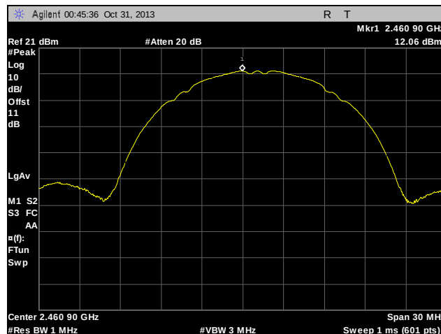
Plot 68. Peak Power Spectral Density, Determination, High Channel, 802.11b
