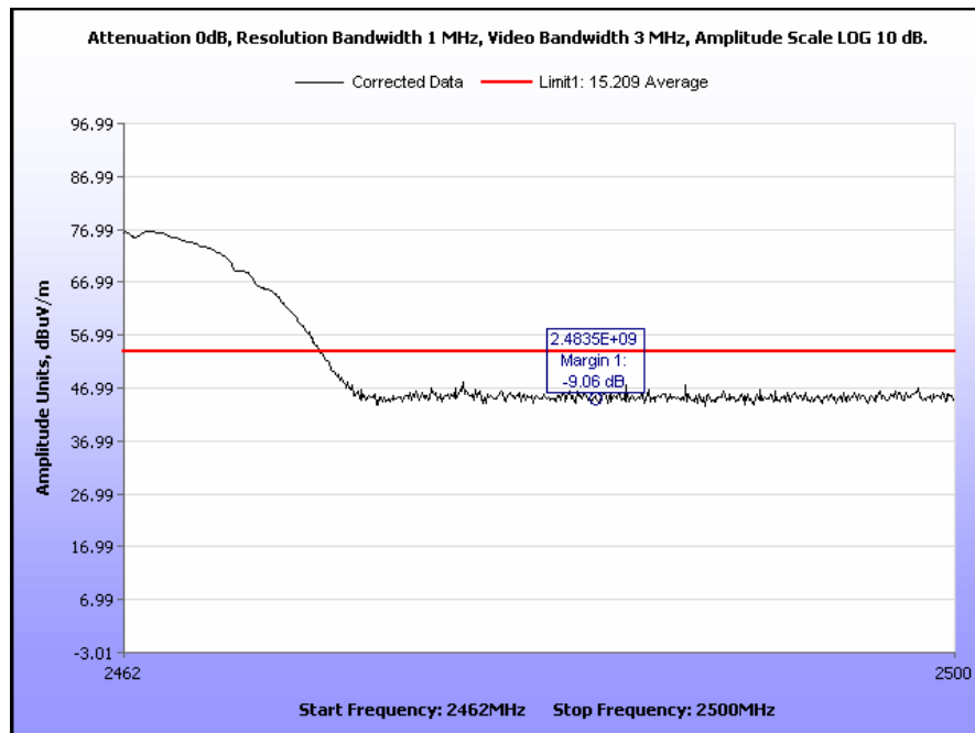
Plot 54. Radiated Restricted Band Edge, High Channel, 802.11n, Peak under Average
