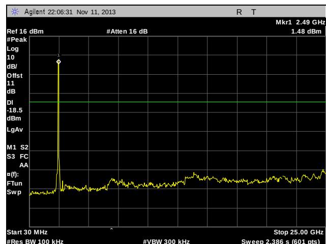
Plot 63. Conducted Spurious Emissions, High Channel, 802.11n
