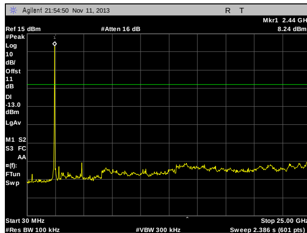
Plot 56. Conducted Spurious Emissions, Mid Channel, 802.11b
