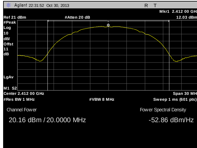
Plot 21. Peak Power Output, Low Channel, 802.11b
