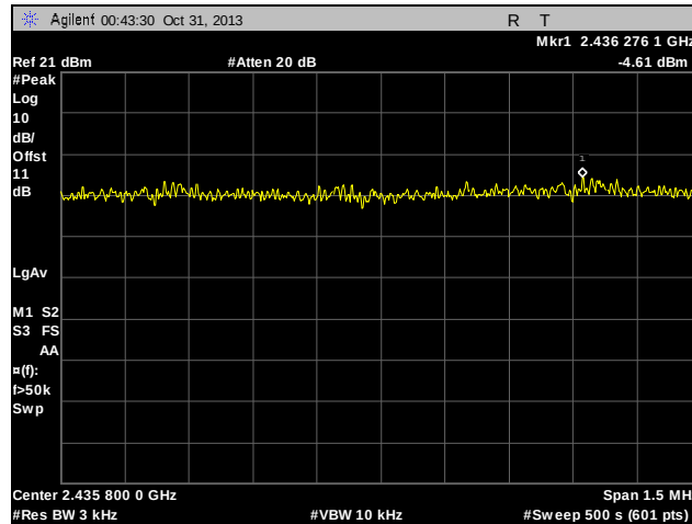
Plot 67. Peak Power Spectral Density, Mid Channel, 802.11b
