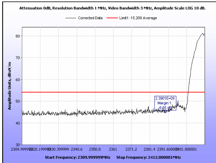
Plot 49. Radiated Restricted Band Edge, Low Channel, 802.11b, Peak under Average
