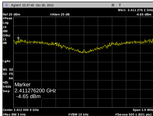
Plot 65. Peak Power Spectral Density, Low Channel, 802.11b
