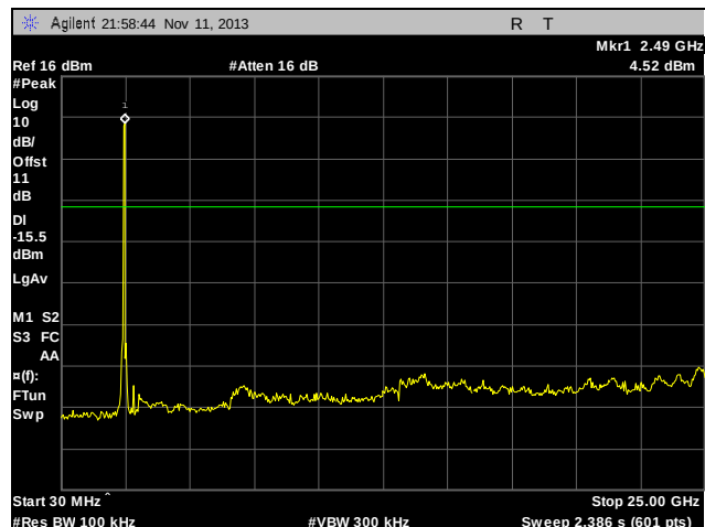
Plot 60. Conducted Spurious Emissions, High Channel, 802.11g
