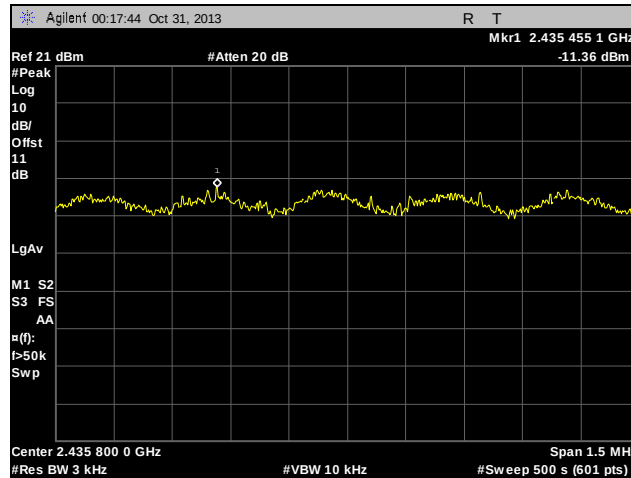
Plot 79. Peak Power Spectral Density, Mid Channel, 802.11n
