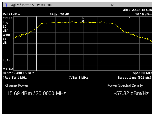
Plot 28. Peak Power Output, Mid Channel, 802.11n
