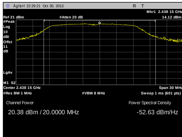
Plot 25. Peak Power Output, Mid Channel, 802.11g
