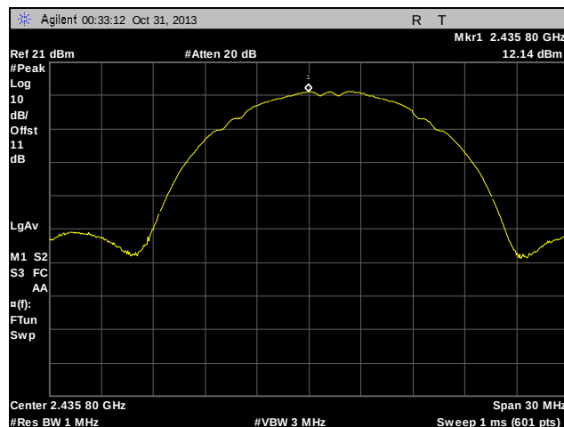
Plot 66. Peak Power Spectral Density, Determination, Mid Channel, 802.11b
