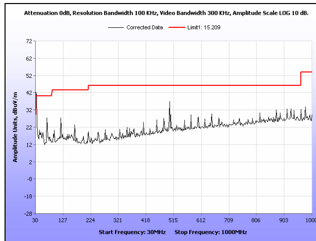
Plot 31. Radiated Spurious Emissions, Low Channel, 802.11b, 30 MHz – 1 GHz
