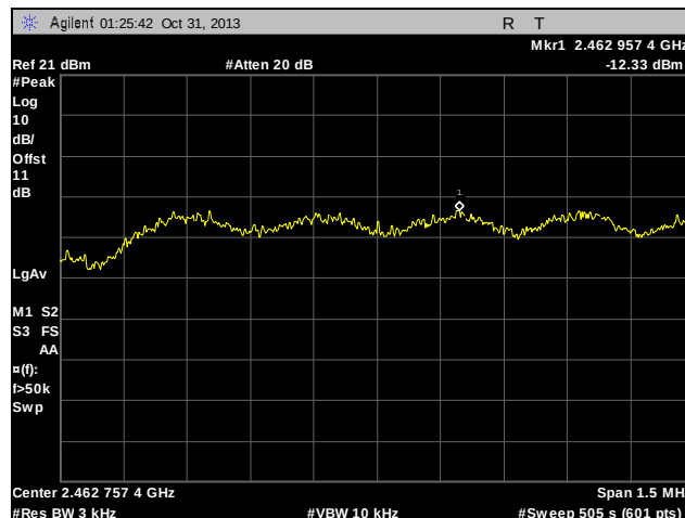
Plot 81. Peak Power Spectral Density, High Channel, 802.11n
