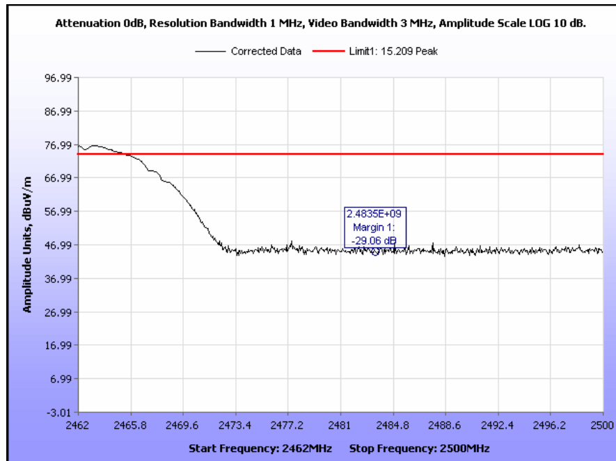
Plot 50. Radiated Restricted Band Edge, High Channel, 802.11b, Peak under Average
