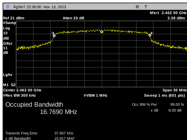
Plot 17. 99% Occupied Bandwidth, High Channel, 802.11g
