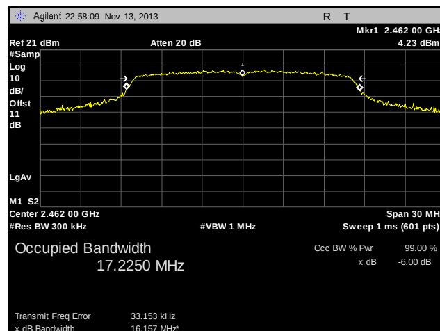
Plot 20. 99% Occupied Bandwidth, High Channel, 802.11n
