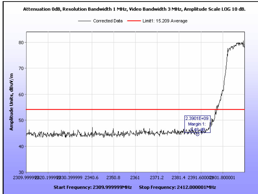
Plot 53. Radiated Restricted Band Edge, Low Channel, 802.11n, Peak under Average
