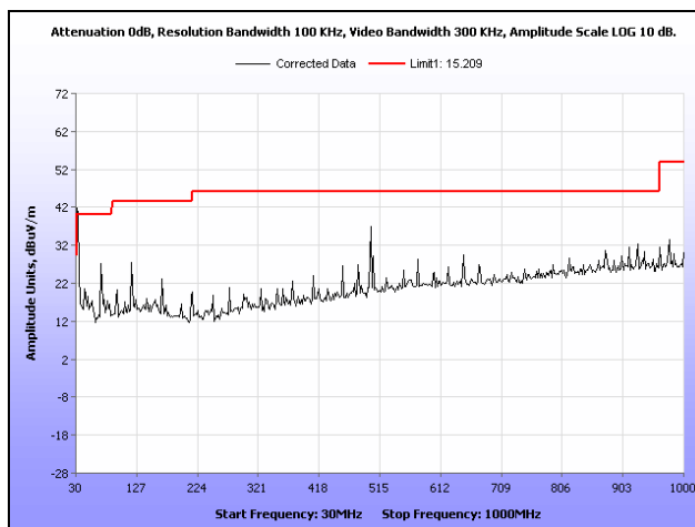
Plot 43. Radiated Spurious Emissions, Low Channel, 802.11n, 30 MHz – 1 GHz
