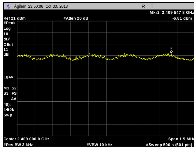
Plot 71. Peak Power Spectral Density, Low Channel, 802.11g
