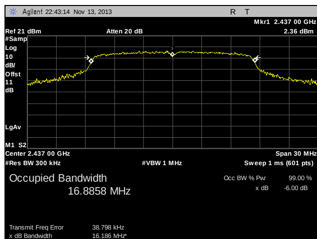
Plot 16. 99% Occupied Bandwidth, Mid Channel, 802.11g
