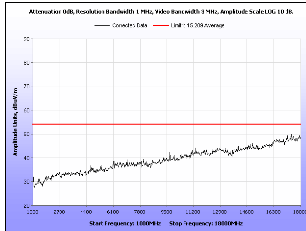
Plot 40. Radiated Spurious Emissions, Mid Channel, 802.11g, 1 GHz – 18 GHz, Peak under Average
