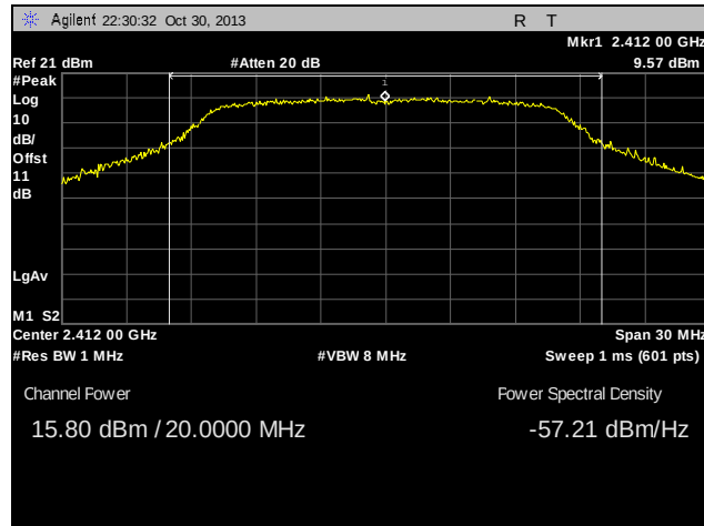
Plot 27. Peak Power Output, Low Channel, 802.11n
