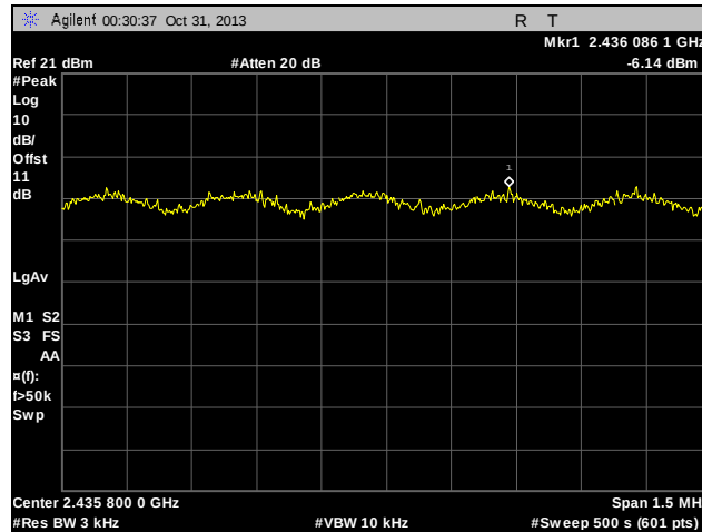
Plot 73. Peak Power Spectral Density, Mid Channel, 802.11g
