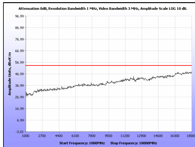
Plot 48. Radiated Spurious Emissions, High Channel, 802.11n, 1 GHz – 18 GHz, Peak under Average
