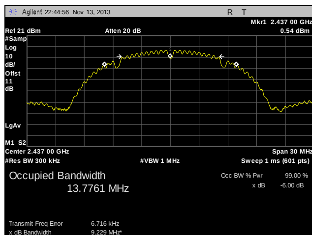
Plot 13. 99% Occupied Bandwidth, Mid Channel, 802.11b
