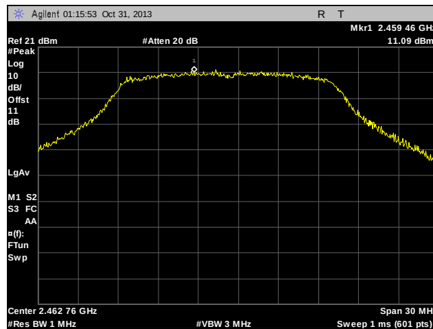
Plot 80. Peak Power Spectral Density, Determination, High Channel, 802.11n
