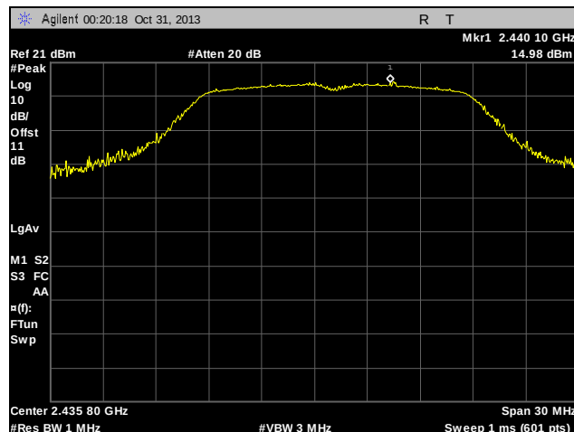
Plot 72. Peak Power Spectral Density, Determination, Mid Channel, 802.11g
