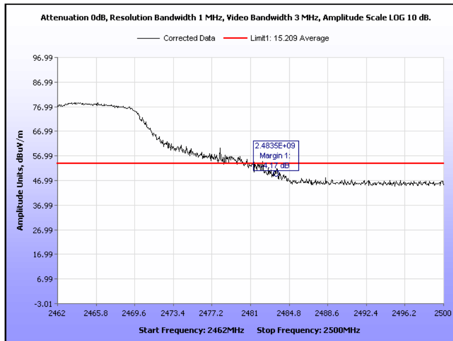
Plot 52. Radiated Restricted Band Edge, High Channel, 802.11g, Peak under Average
