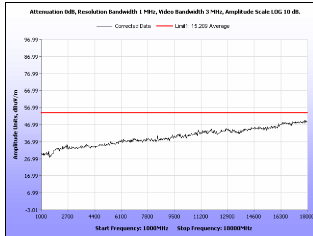
Plot 46. Radiated Spurious Emissions, Mid Channel, 802.11n, 1 GHz – 18 GHz, Peak under Average
