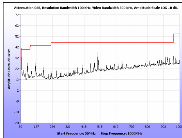
Plot 47. Radiated Spurious Emissions, High Channel, 802.11n, 30 MHz – 1 GHz
