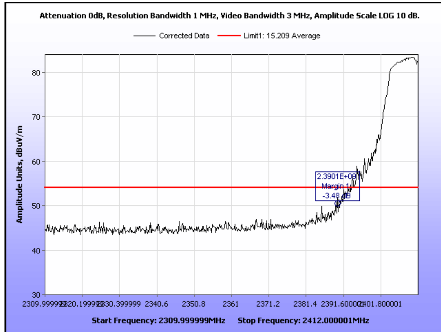
Plot 51. Radiated Restricted Band Edge, Low Channel, 802.11g, Peak under Average
