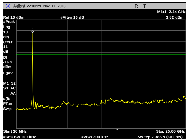
Plot 59. Conducted Spurious Emissions, Mid Channel, 802.11g
