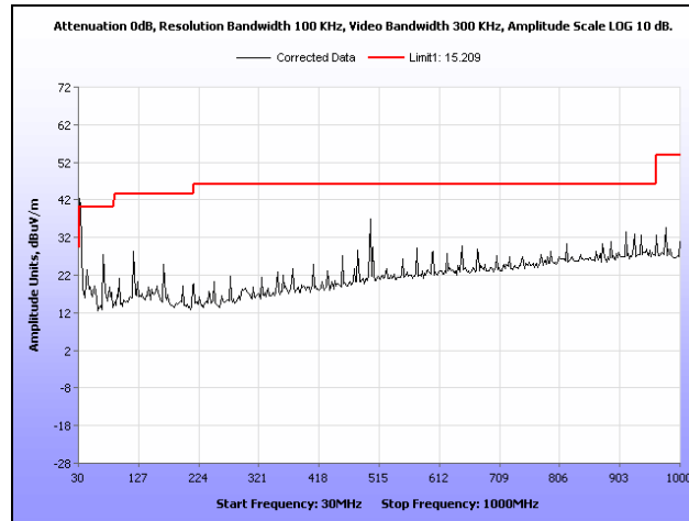
Plot 37. Radiated Spurious Emissions, Low Channel, 802.11g, 30 MHz – 1 GHz
