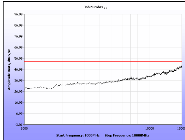
Plot 34. Radiated Spurious Emissions, Mid Channel, 802.11b, 1 GHz – 18 GHz, Peak under Average
