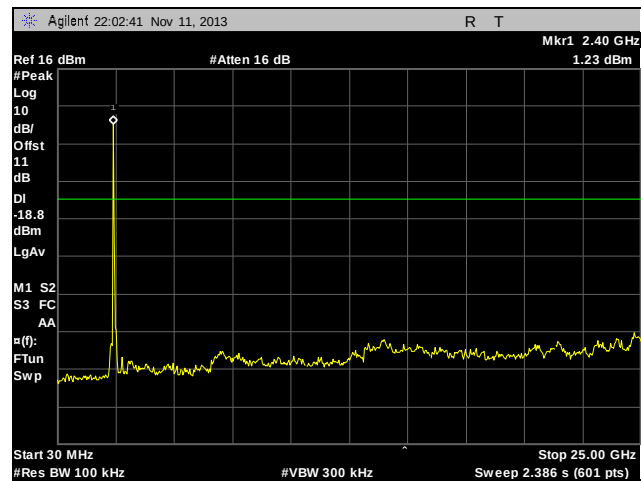
Plot 61. Conducted Spurious Emissions, Low Channel, 802.11n
