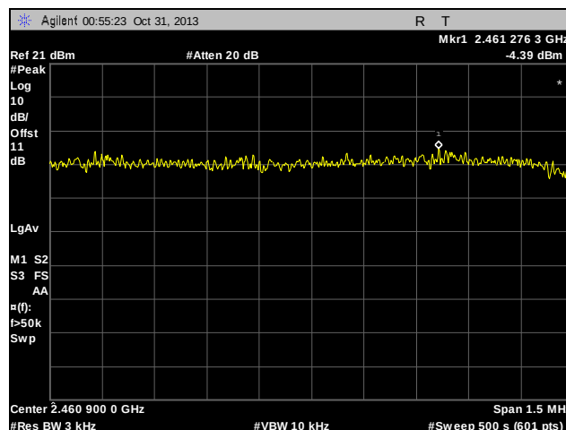
Plot 69. Peak Power Spectral Density, High Channel, 802.11b
