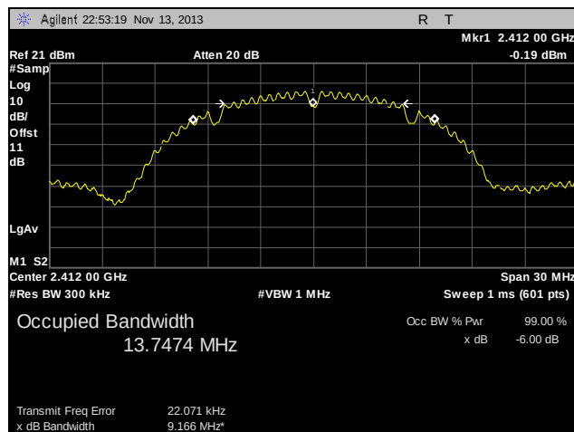
Plot 12. 99% Occupied Bandwidth, Low Channel, 802.11b
