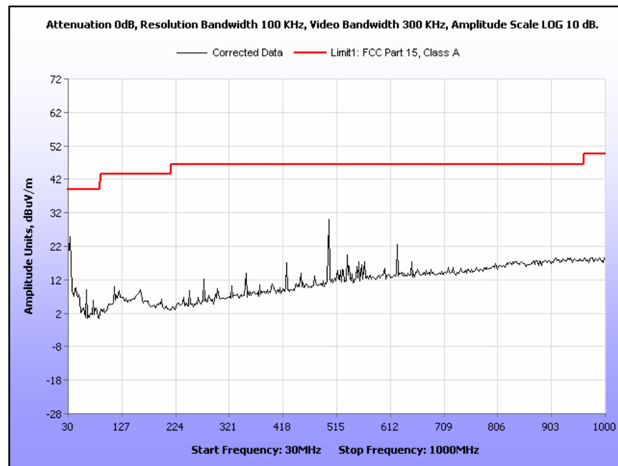
Plot 30. Radiated Emissions, 30 MHz - 1 GHz
