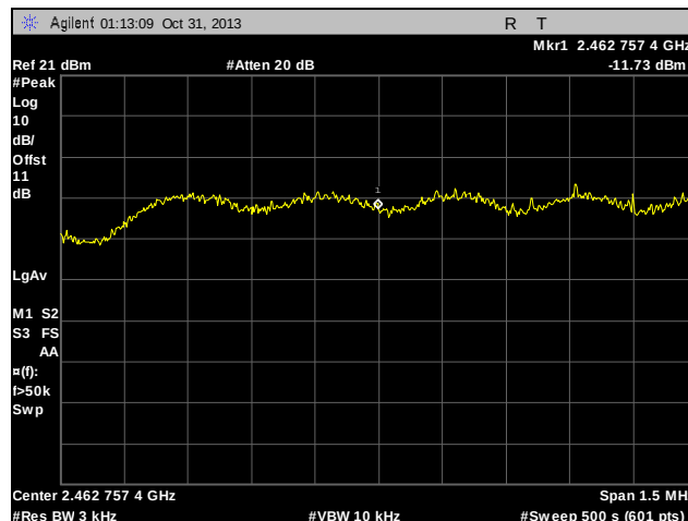
Plot 75. Peak Power Spectral Density, High Channel, 802.11g
