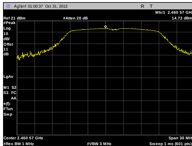
Plot 74. Peak Power Spectral Density, Determination, High Channel, 802.11g
