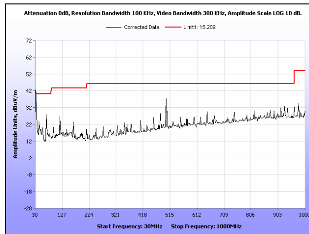
Plot 35. Radiated Spurious Emissions, High Channel, 802.11b, 30 MHz – 1 GHz
