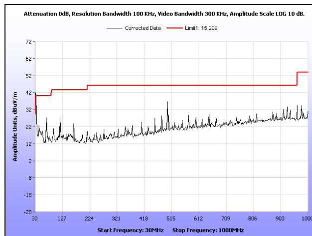
Plot 33. Radiated Spurious Emissions, Mid Channel, 802.11b, 30 MHz – 1 GHz
