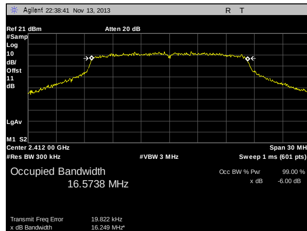
Plot 18. 99% Occupied Bandwidth, Low Channel, 802.11n
