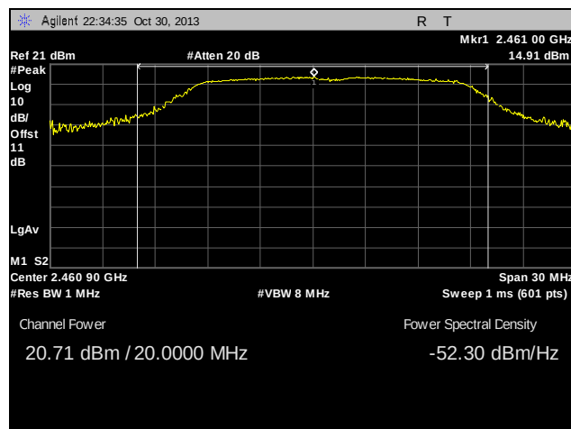
Plot 29. Peak Power Output, High Channel, 802.11n
