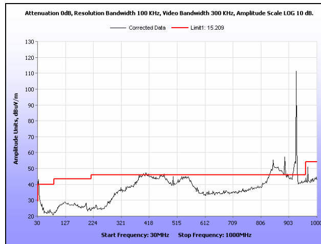
Plot 23. Radiated Spurious Emissions, High Channel, 30 MHz – 1 GHz
