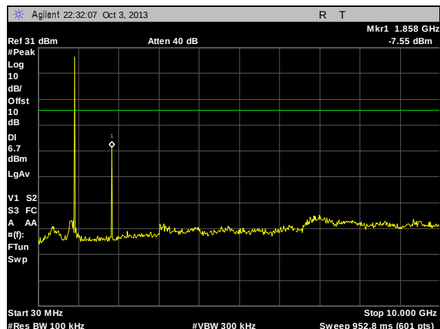
Plot 31. Conducted Spurious Emissions, High Channel
