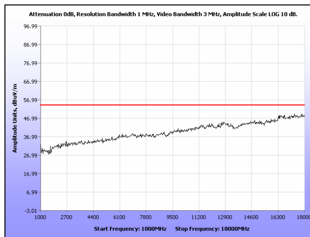
Plot 34. Radiated Spurious Emissions, Low Channel, 802.11b, 1 GHz – 18 GHz, Peak under Average
