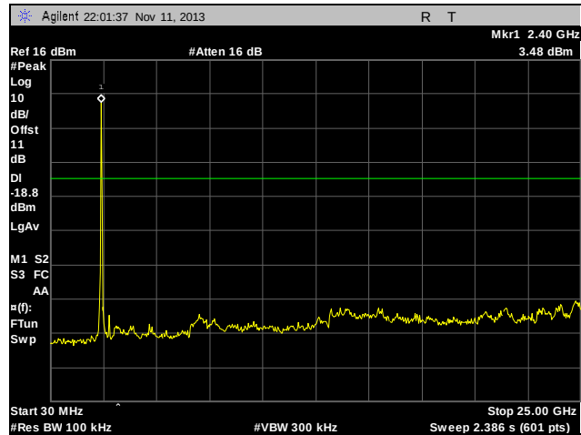
Plot 66. Conducted Spurious Emissions, Low Channel, 802.11g
