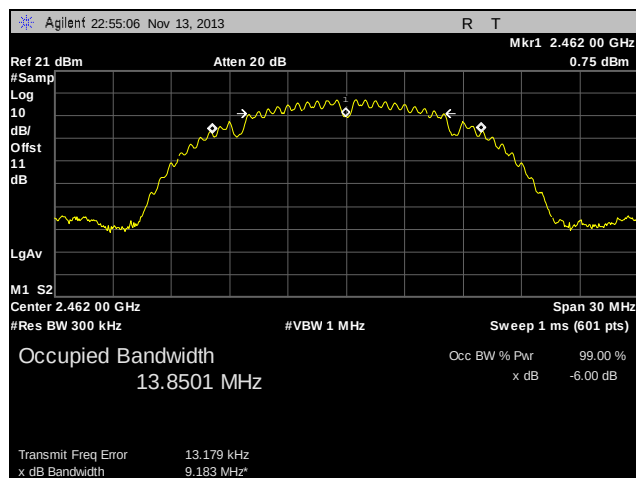
Plot 17. 99% Occupied Bandwidth, High Channel, 802.11b
