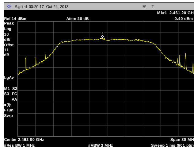
Plot 94. Peak Power Spectral Density, Determination, High Channel, 802.11n
