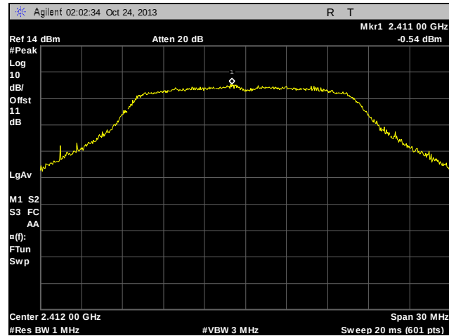
Plot 90. Peak Power Spectral Density, Determination, Low Channel, 802.11n
