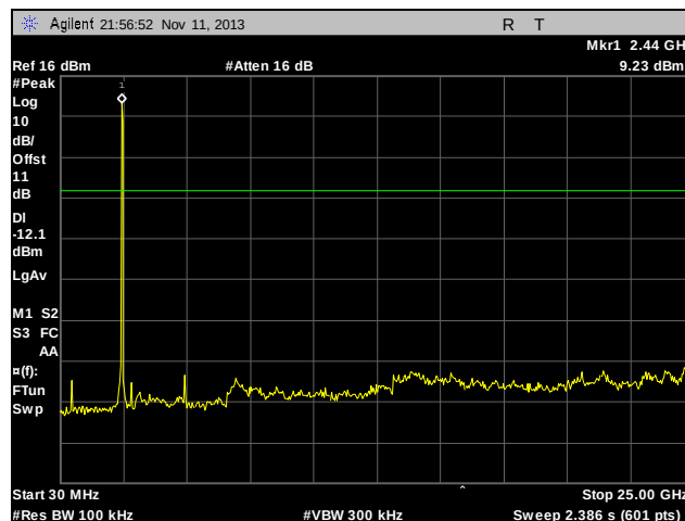
Plot 65. Conducted Spurious Emissions, High Channel, 802.11b
