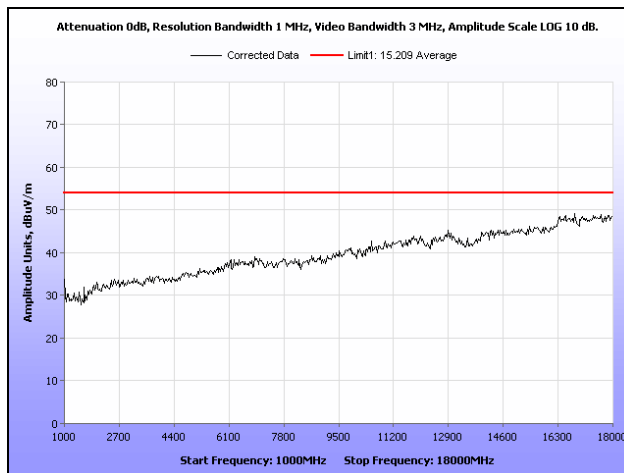
Plot 42. Radiated Spurious Emissions, Mid Channel, 802.11g, 1 GHz – 18 GHz, Peak under Average
