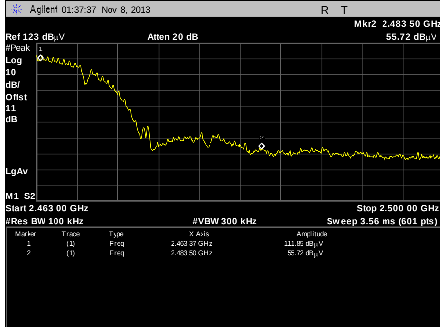
Plot 73. Band Edge, 802.11b, High Channel
