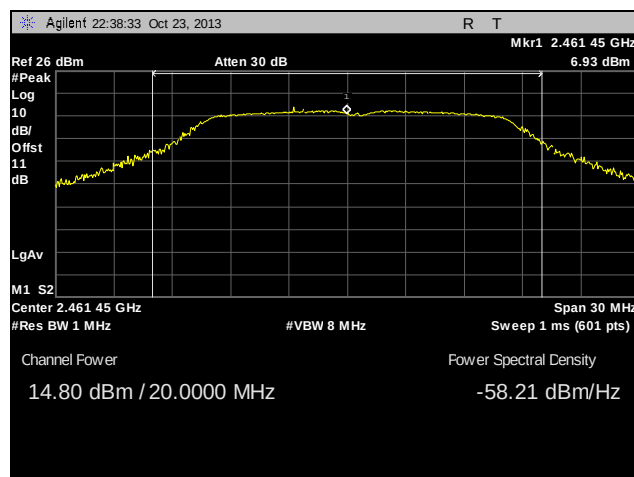
Plot 29. Peak Power Output, High Channel, 802.11g
