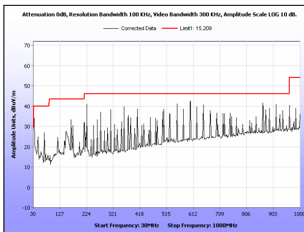
Plot 43. Radiated Spurious Emissions, High Channel, 802.11g, 30 MHz – 1 GHz
