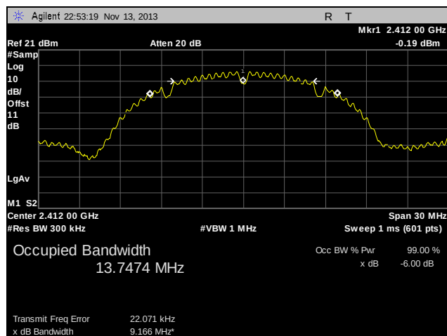
Plot 15. 99% Occupied Bandwidth, Low Channel, 802.11b
