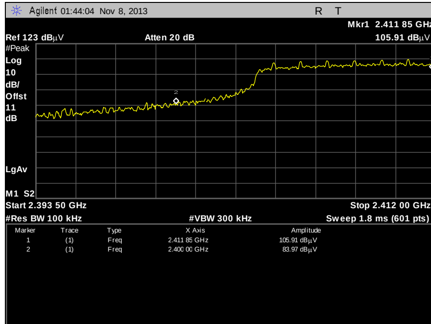
Plot 74. Band Edge, 802.11g, Low Channel
