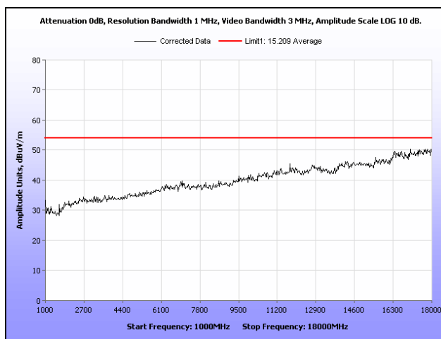
Plot 40. Radiated Spurious Emissions, Low Channel, 802.11g, 1 GHz – 18 GHz, Peak under Average
