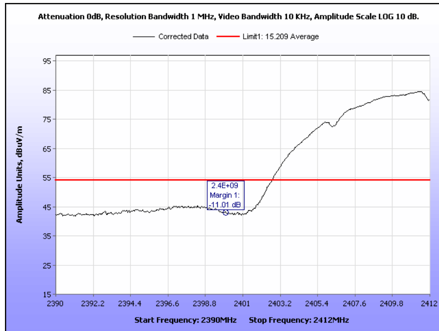
Plot 51. Radiated Restricted Band Edge, Low Channel, 802.11b, Average
