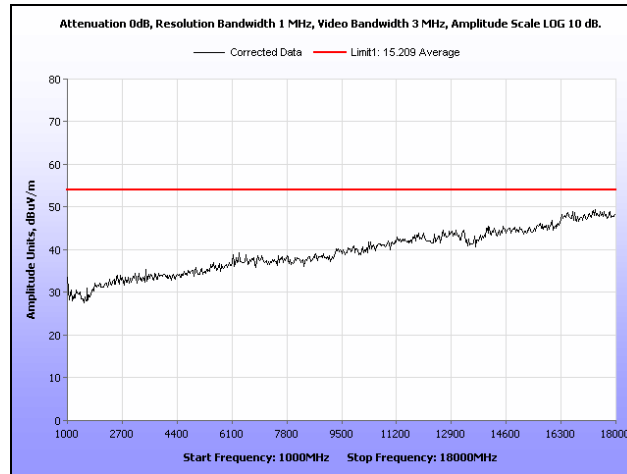
Plot 36. Radiated Spurious Emissions, Mid Channel, 802.11b, 1 GHz – 18 GHz, Peak under Average
