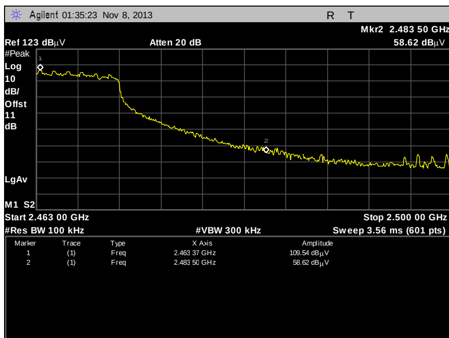
Plot 77. Band Edge, 802.11n, High Channel
