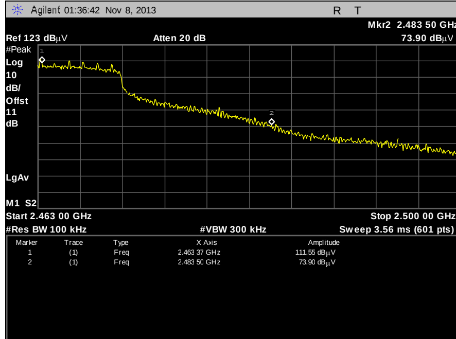
Plot 75. Band Edge, 802.11g, High Channel
