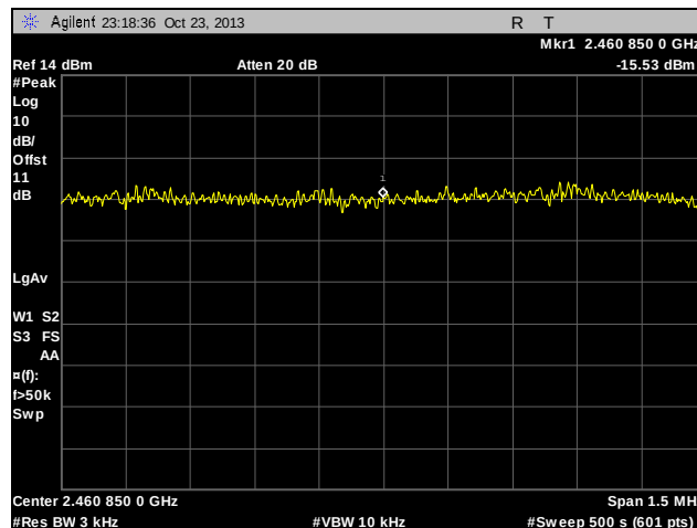
Plot 83. Peak Power Spectral Density, High Channel, 802.11b
