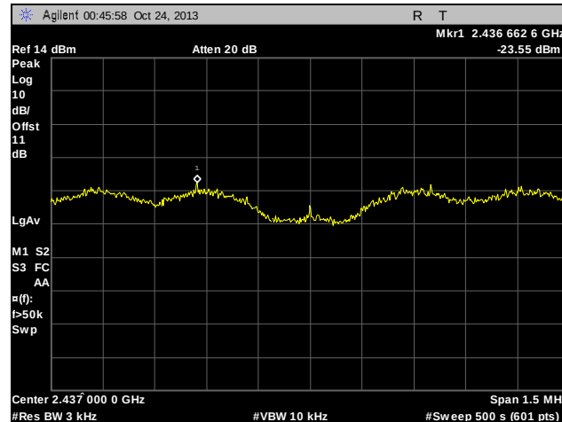
Plot 93. Peak Power Spectral Density, Mid Channel, 802.11n
