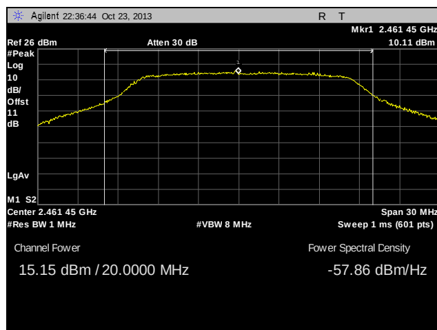
Plot 32. Peak Power Output, High Channel, 802.11n
