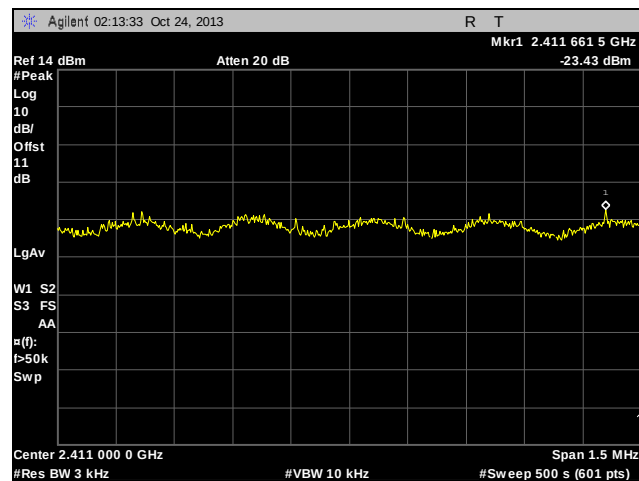
Plot 91. Peak Power Spectral Density, Low Channel, 802.11n
