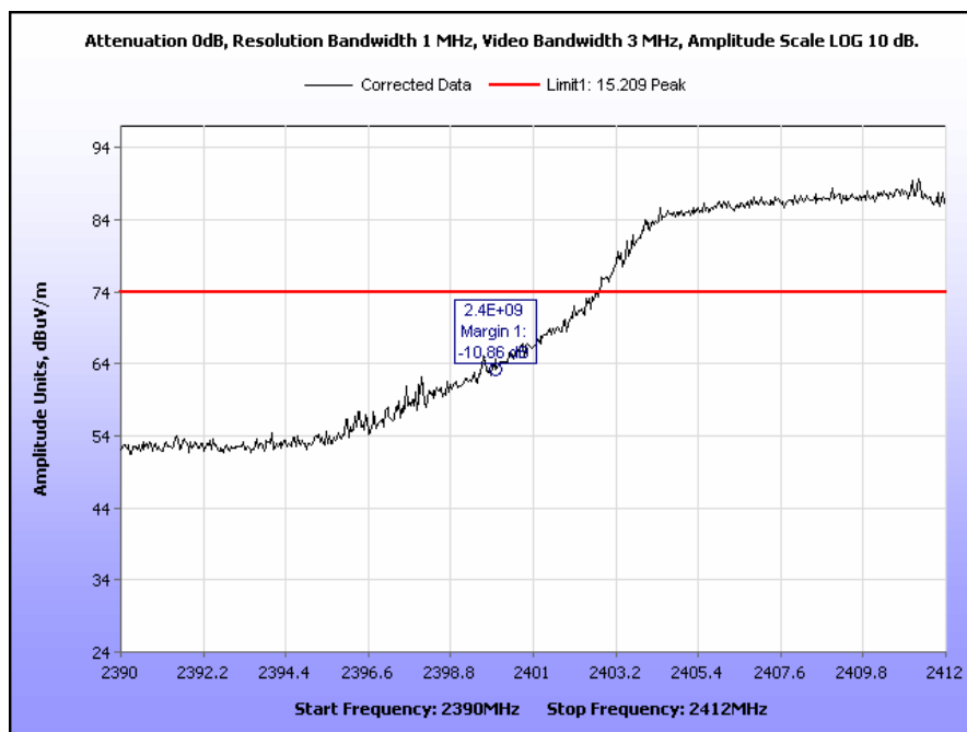
Plot 60. Radiated Restricted Band Edge, Low Channel, 802.11n, Peak
