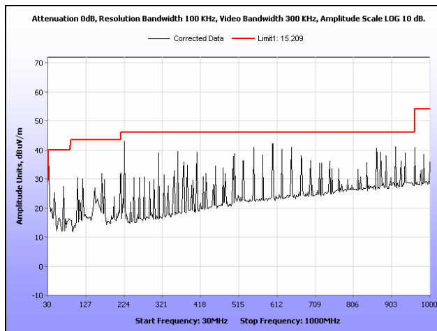
Plot 39. Radiated Spurious Emissions, Low Channel, 802.11g, 30 MHz – 1 GHz
