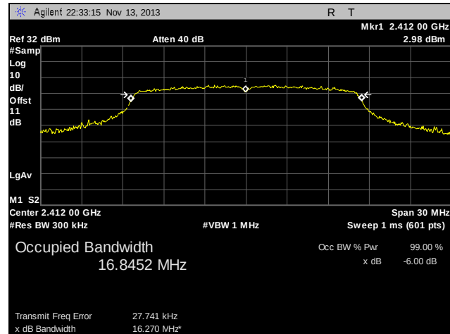
Plot 18. 99% Occupied Bandwidth, Low Channel, 802.11g
