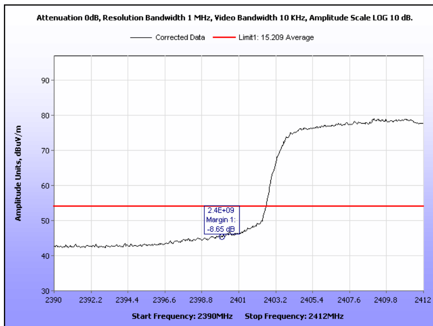
Plot 59. Radiated Restricted Band Edge, Low Channel, 802.11n, Average
