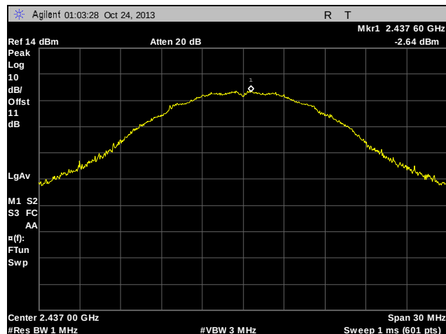
Plot 80. Peak Power Spectral Density, Determination, Mid Channel, 802.11b
