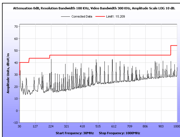
Plot 47. Radiated Spurious Emissions, Mid Channel, 802.11n, 30 MHz – 1 GHz
