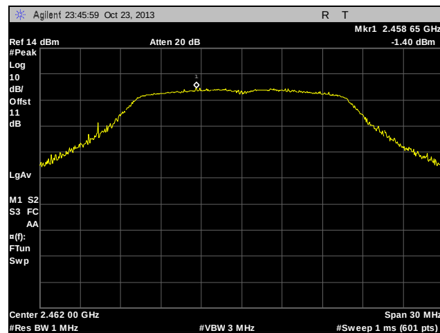
Plot 88. Peak Power Spectral Density, Determination, High Channel, 802.11g
