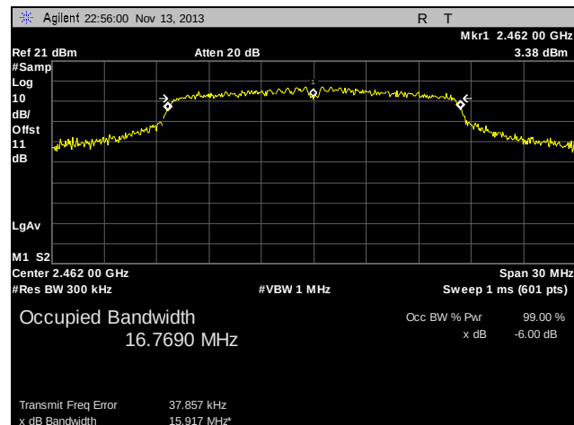
Plot 20. 99% Occupied Bandwidth, High Channel, 802.11g
