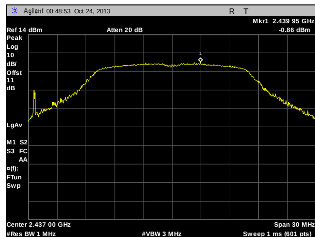
Plot 86. Peak Power Spectral Density, Determination, Mid Channel, 802.11g
