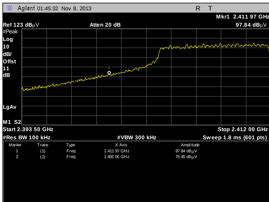
Plot 76. Band Edge, 802.11n, Low Channel
