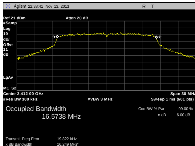
Plot 21. 99% Occupied Bandwidth, Low Channel, 802.11n
