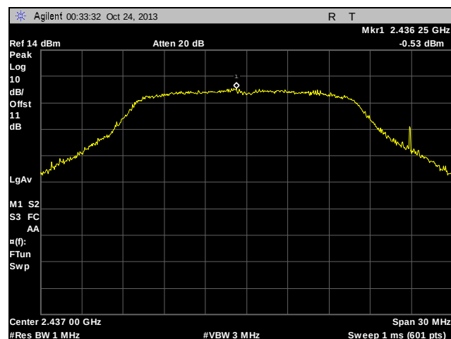
Plot 92. Peak Power Spectral Density, Determination, Mid Channel, 802.11n
