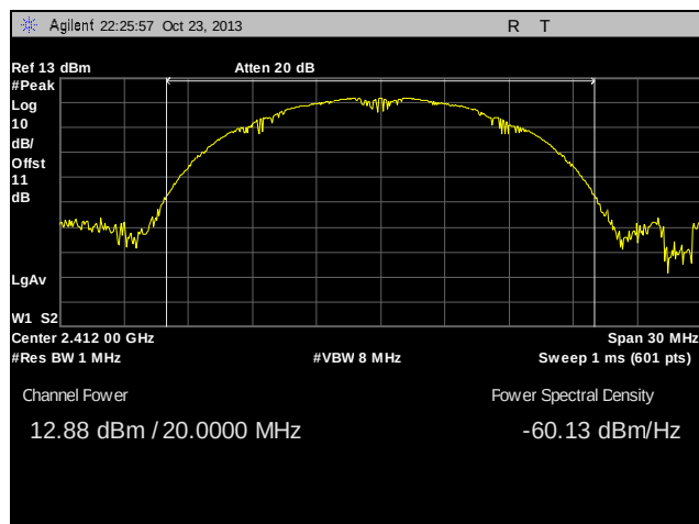
Plot 24. Peak Power Output, Low Channel, 802.11b
