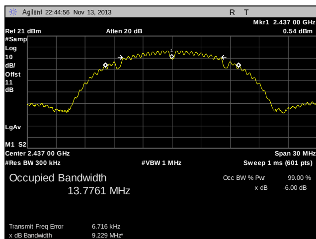
Plot 16. 99% Occupied Bandwidth, Mid Channel, 802.11b
