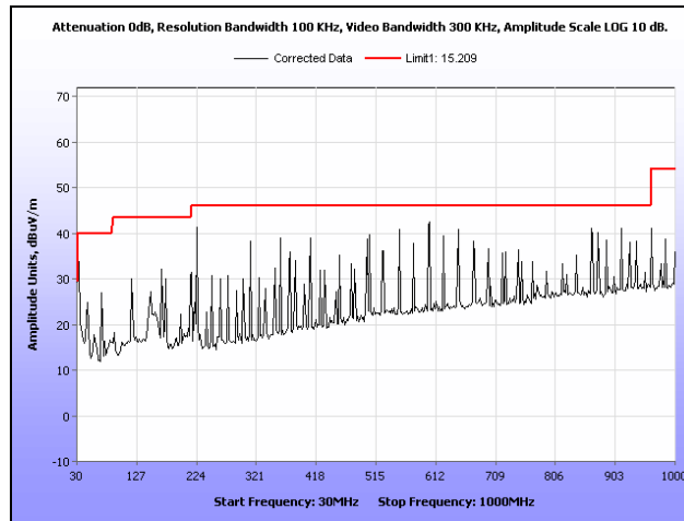
Plot 33. Radiated Spurious Emissions, Low Channel, 802.11b, 30 MHz – 1 GHz
