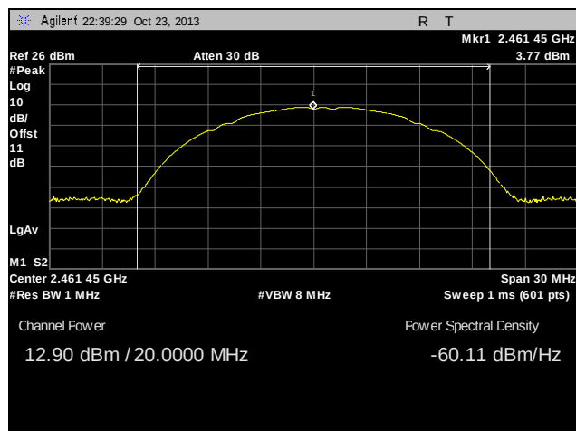
Plot 26. Peak Power Output, High Channel, 802.11b
