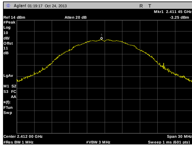
Plot 78. Peak Power Spectral Density, Determination, Low Channel, 802.11b
