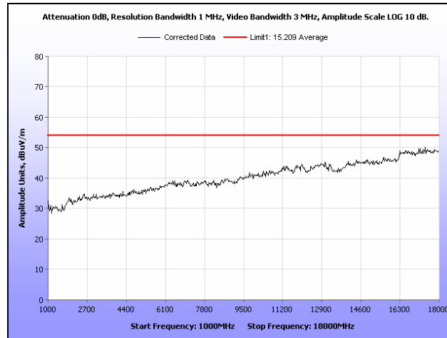
Plot 48. Radiated Spurious Emissions, Mid Channel, 802.11n, 1 GHz – 18 GHz, Peak under Average
