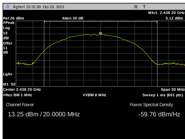
Plot 25. Peak Power Output, Mid Channel, 802.11b
