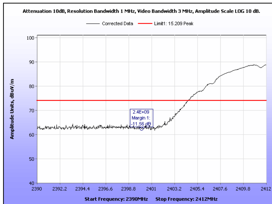
Plot 52. Radiated Restricted Band Edge, Low Channel, 802.11b, Peak
