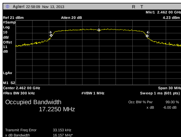
Plot 23. 99% Occupied Bandwidth, High Channel, 802.11n
