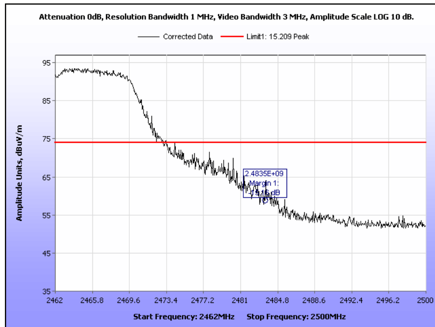
Plot 58. Radiated Restricted Band Edge, High Channel, 802.11g, Peak
