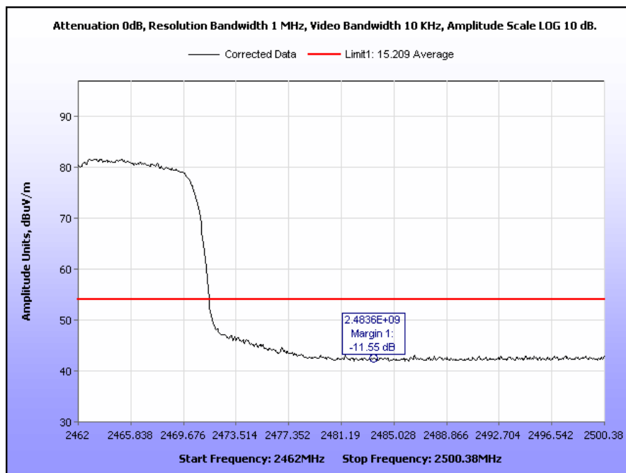
Plot 61. Radiated Restricted Band Edge, High Channel, 802.11n, Average
