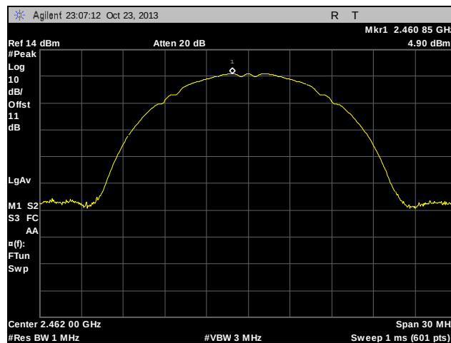
Plot 82. Peak Power Spectral Density, Determination, High Channel, 802.11b
