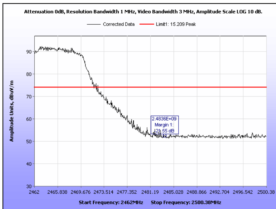
Plot 62. Radiated Restricted Band Edge, High Channel, 802.11n, Peak
