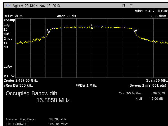
Plot 19. 99% Occupied Bandwidth, Mid Channel, 802.11g
