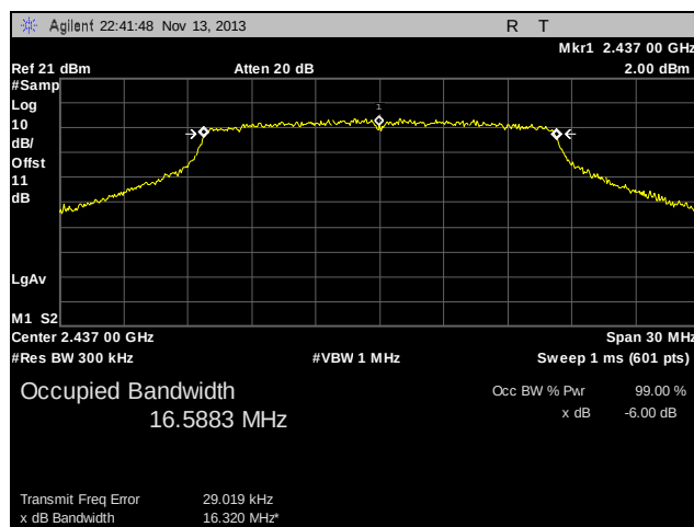
Plot 22. 99% Occupied Bandwidth, Mid Channel, 802.11n
