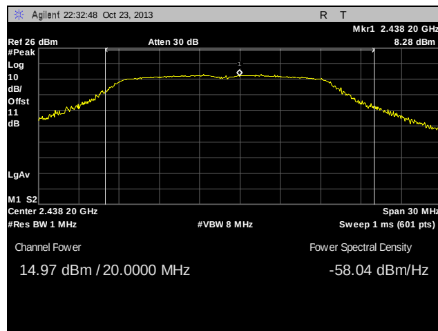
Plot 28. Peak Power Output, Mid Channel, 802.11g
