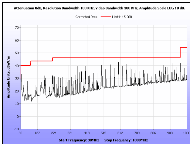
Plot 45. Radiated Spurious Emissions, Low Channel, 802.11n, 30 MHz – 1 GHz
