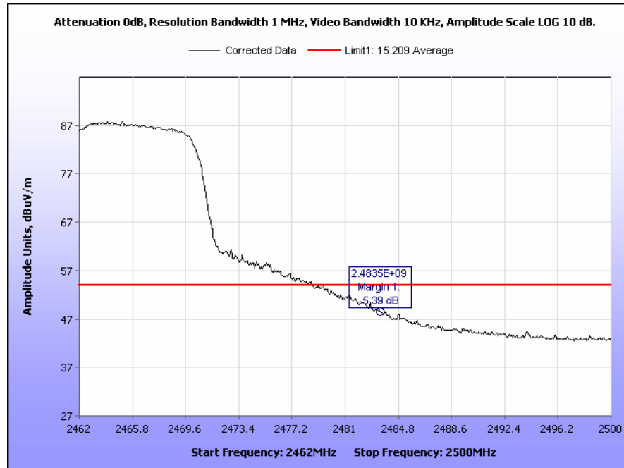
Plot 57. Radiated Restricted Band Edge, High Channel, 802.11g, Average
