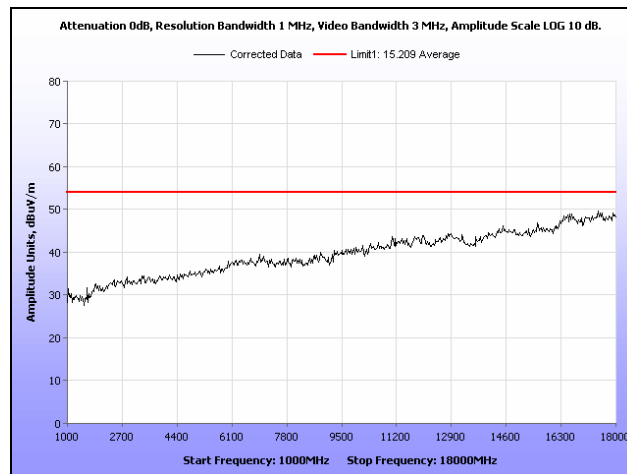
Plot 50. Radiated Spurious Emissions, High Channel, 802.11n, 1 GHz – 18 GHz, Peak under Average
