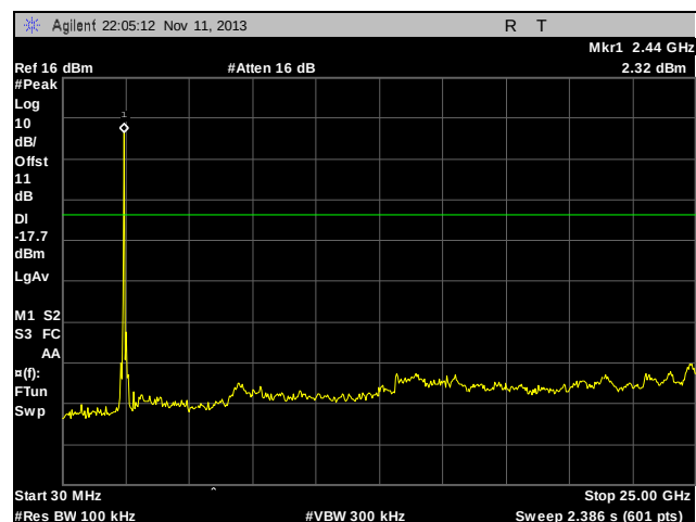
Plot 70. Conducted Spurious Emissions, Mid Channel, 802.11n
