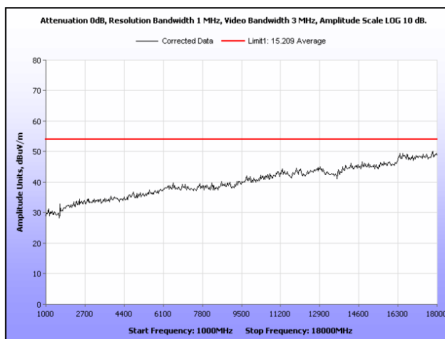
Plot 44. Radiated Spurious Emissions, High Channel, 802.11g, 1 GHz – 18 GHz, Peak under Average
