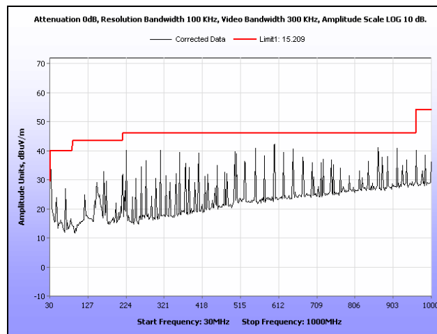
Plot 37. Radiated Spurious Emissions, High Channel, 802.11b, 30 MHz – 1 GHz
