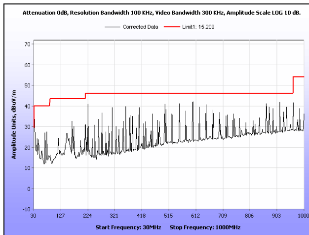
Plot 41. Radiated Spurious Emissions, Mid Channel, 802.11g, 30 MHz – 1 GHz
