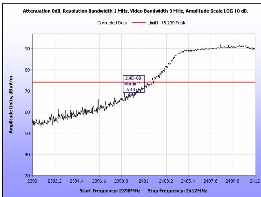
Plot 56. Radiated Restricted Band Edge, Low Channel, 802.11g, Peak
