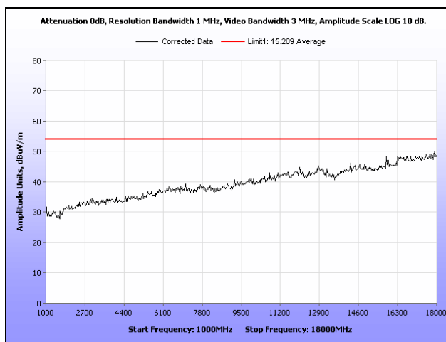
Plot 46. Radiated Spurious Emissions, Low Channel, 802.11n, 1 GHz – 18 GHz, Peak under Average
