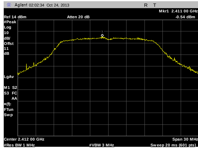
Plot 84. Peak Power Spectral Density, Determination, Low Channel, 802.11g
