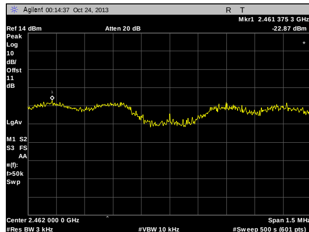
Plot 89. Peak Power Spectral Density, High Channel, 802.11g
