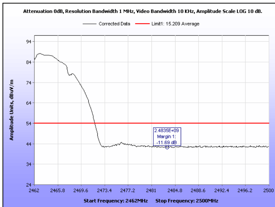
Plot 53. Radiated Restricted Band Edge, High Channel, 802.11b, Average
