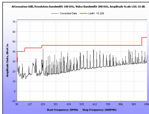
Plot 49. Radiated Spurious Emissions, High Channel, 802.11n, 30 MHz – 1 GHz
