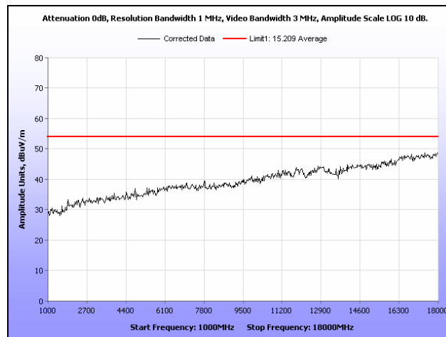
Plot 38. Radiated Spurious Emissions, High Channel, 802.11b, 1 GHz – 18 GHz, Peak under Average
