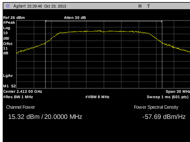
Plot 30. Peak Power Output, Low Channel, 802.11n
