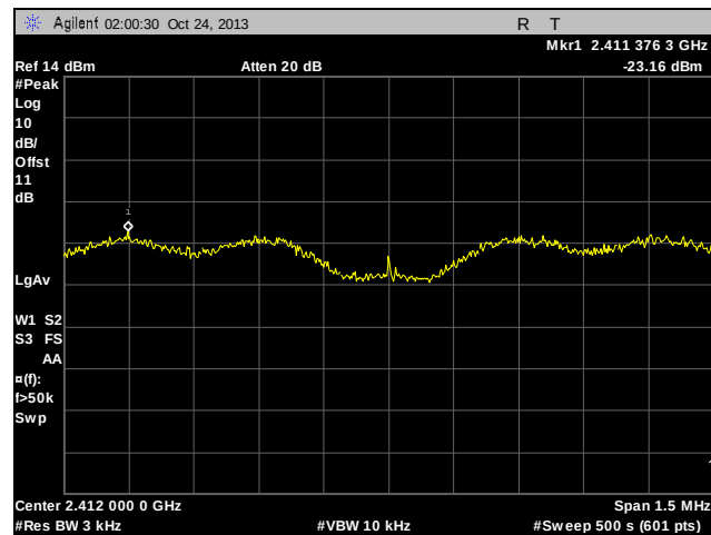
Plot 85. Peak Power Spectral Density, Low Channel, 802.11g
