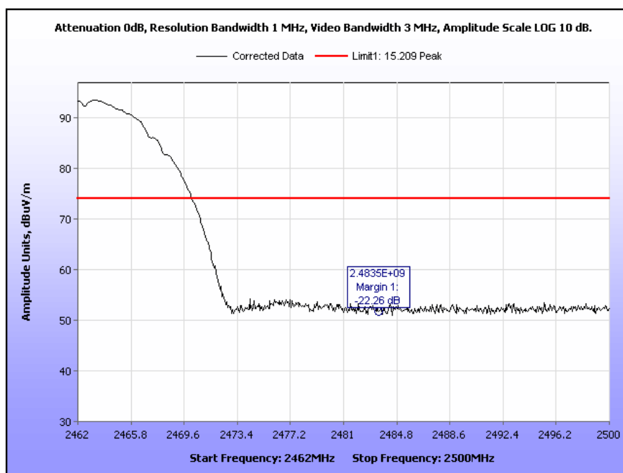
Plot 54. Radiated Restricted Band Edge, High Channel, 802.11b, Peak
