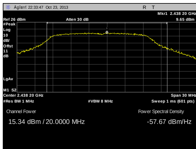
Plot 31. Peak Power Output, Mid Channel, 802.11n
