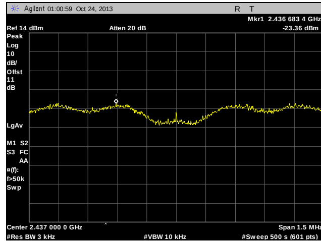
Plot 87. Peak Power Spectral Density, Mid Channel, 802.11g
