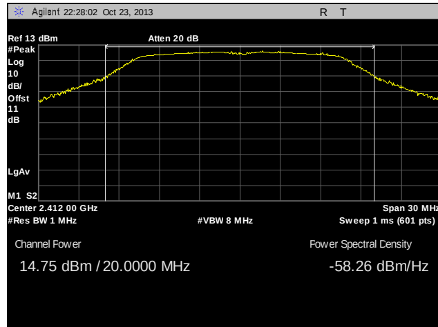
Plot 27. Peak Power Output, Low Channel, 802.11g
