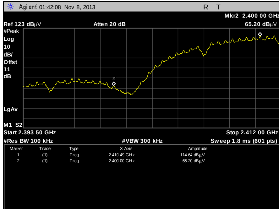
Plot 72. Band Edge, 802.11b, Low Channel
