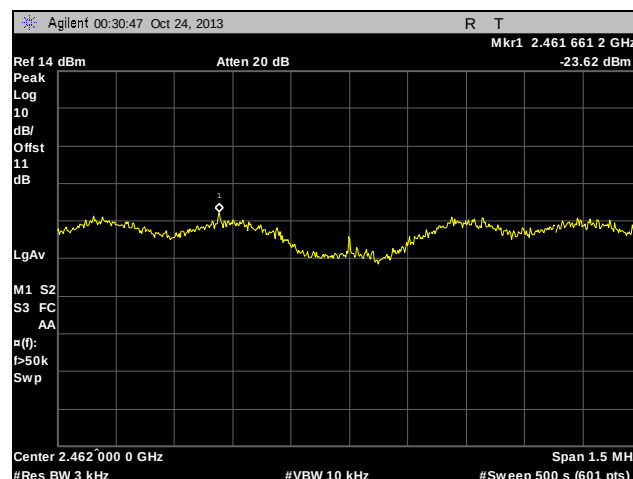
Plot 95. Peak Power Spectral Density, High Channel, 802.11n
