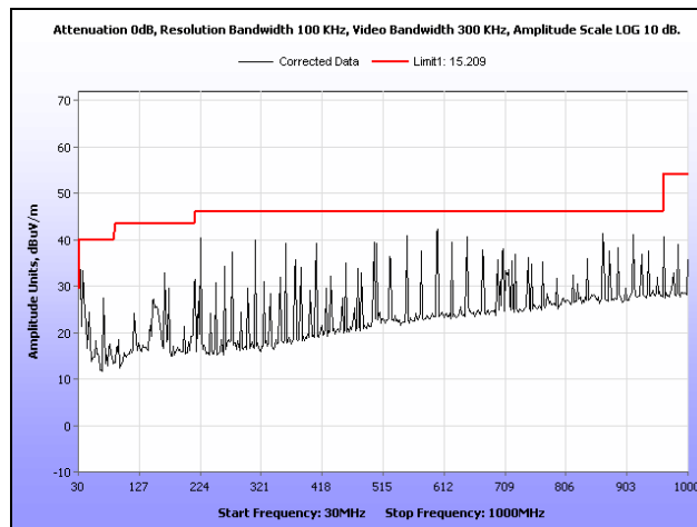
Plot 35. Radiated Spurious Emissions, Mid Channel, 802.11b, 30 MHz – 1 GHz
