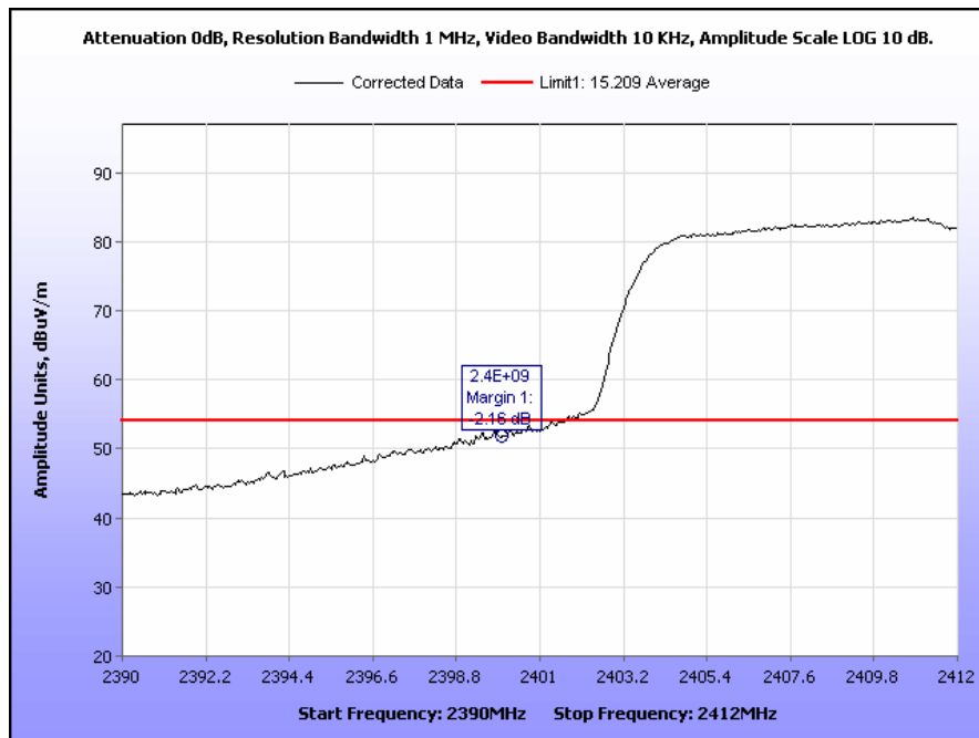
Plot 55. Radiated Restricted Band Edge, Low Channel, 802.11g, Average
