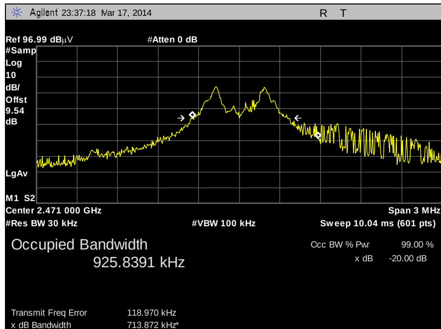
Plot 11. 99% Occupied Bandwidth, 2471 MHz
