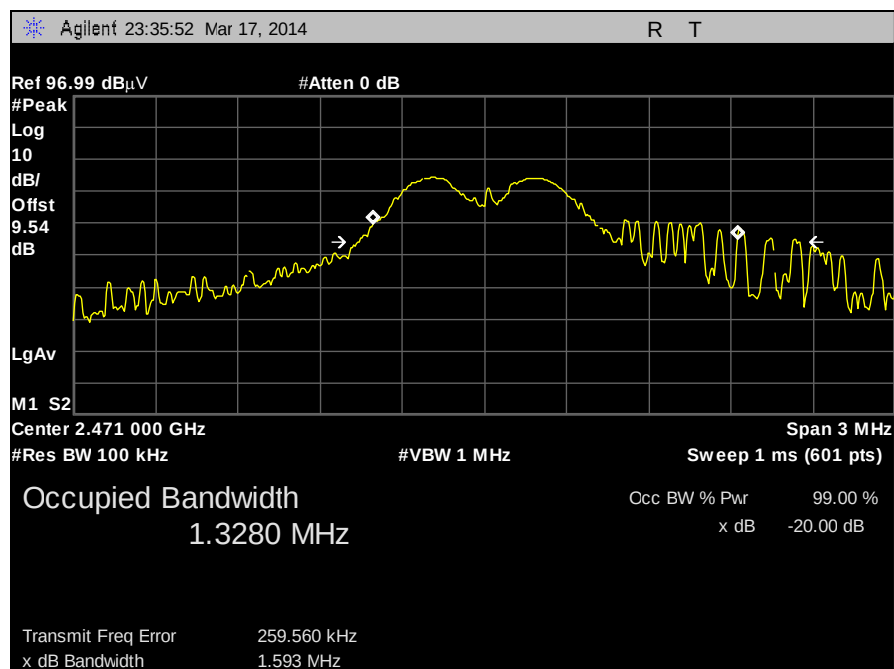
Plot 7. 20 dB Occupied Bandwidth, 2471 MHz
