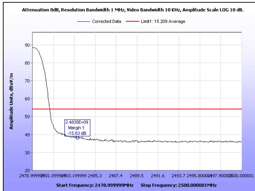
Plot 27. Restricted Band, 2479 MHz, Average
