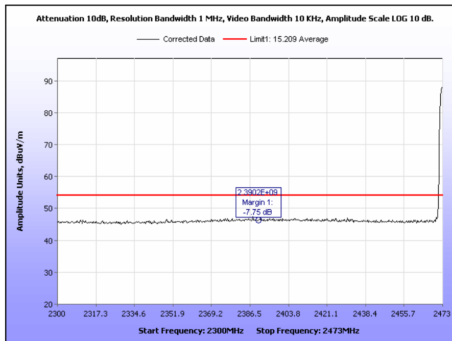
Plot 25. Restricted Band, 2473 MHz, Average
