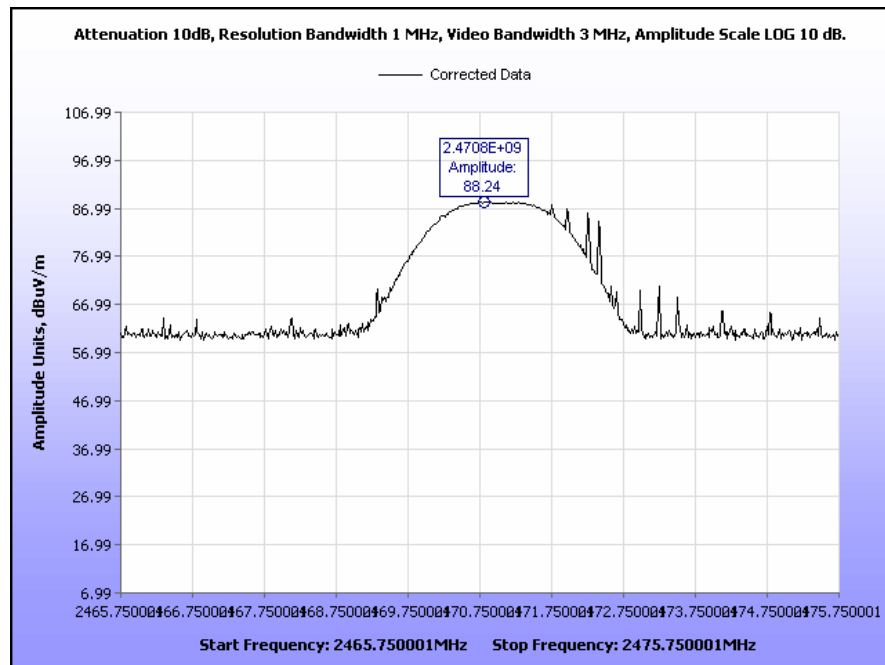
Plot 3. Radiated Field Strength of Fundamental, 2471 MHz
