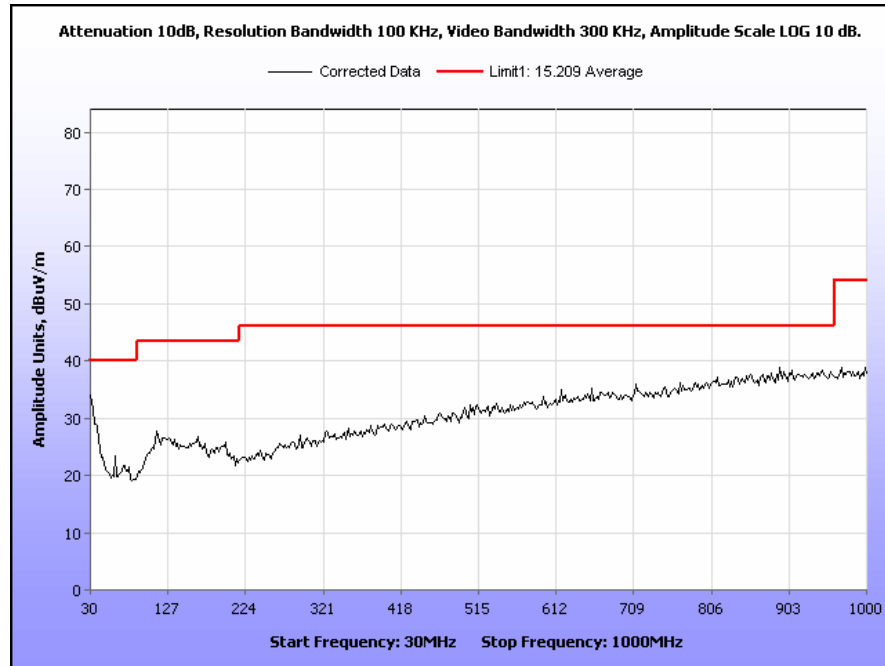
Plot 16. Radiated Spurious Emissions, 2471 MHz, 30 MHz – 1 GHz
