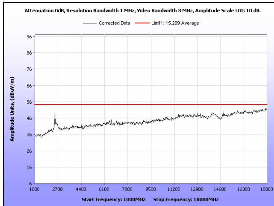
Plot 17. Radiated Spurious Emissions, 2471 MHz, Peak under Average, 1 GHz – 18 GHz
