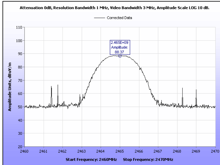
Plot 2. Radiated Field Strength of Fundamental, 2465 MHz
