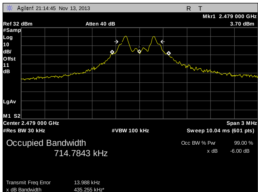
Plot 13. 99% Occupied Bandwidth, 2479 MHz
