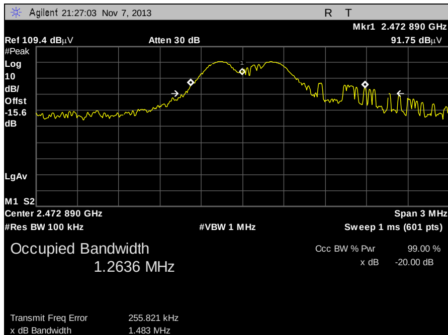
Plot 8. 20 dB Occupied Bandwidth, 2473 MHz
