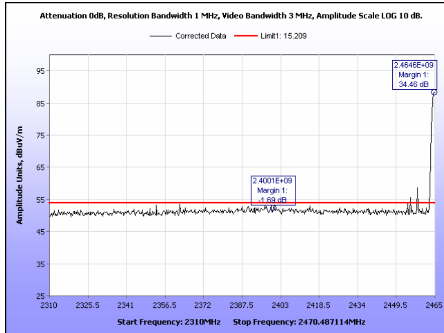
Plot 22. Restricted Band, 2465 MHz, Peak under Average
