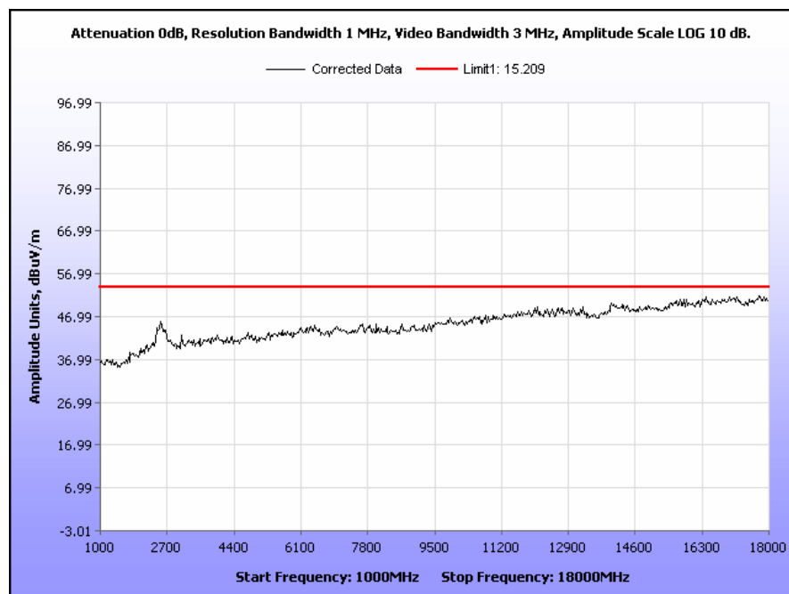
Plot 15. Radiated Spurious Emissions, 2465 MHz, Peak under Average, 1 GHz – 18 GHz
