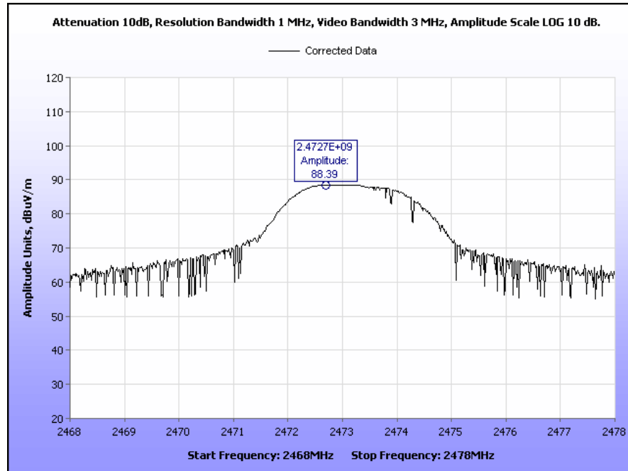
Plot 4. Radiated Field Strength of Fundamental, 2473 MHz
