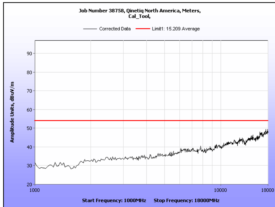
Plot 19. Radiated Spurious Emissions, 2473 MHz, Peak under Average, 1 GHz – 18 GHz
