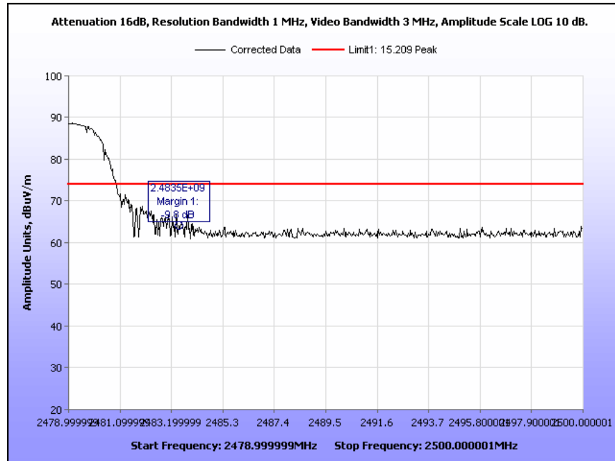
Plot 26. Restricted Band, 2479 MHz, Peak
