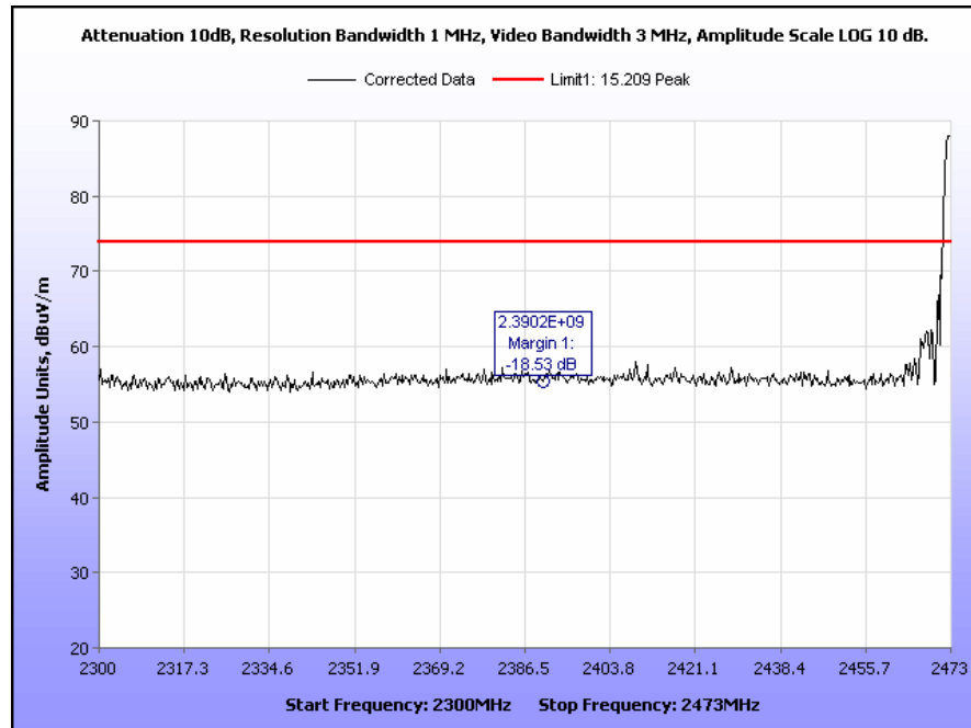
Plot 24. Restricted Band, 2473 MHz, Peak
