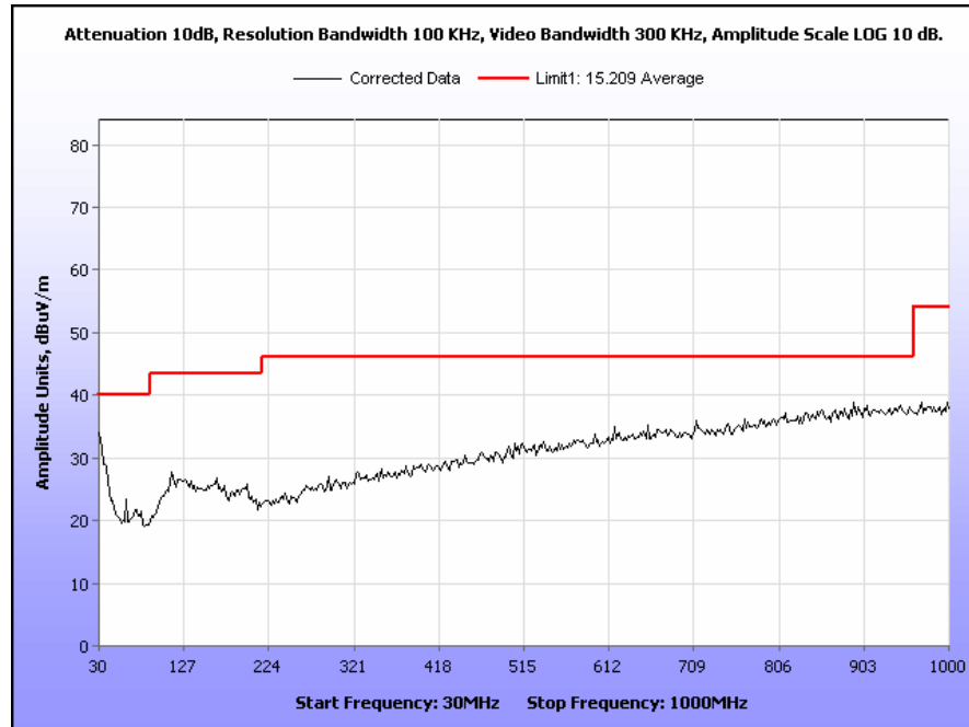
Plot 20. Radiated Spurious Emissions, 2479 MHz, 30 MHz – 1 GHz
