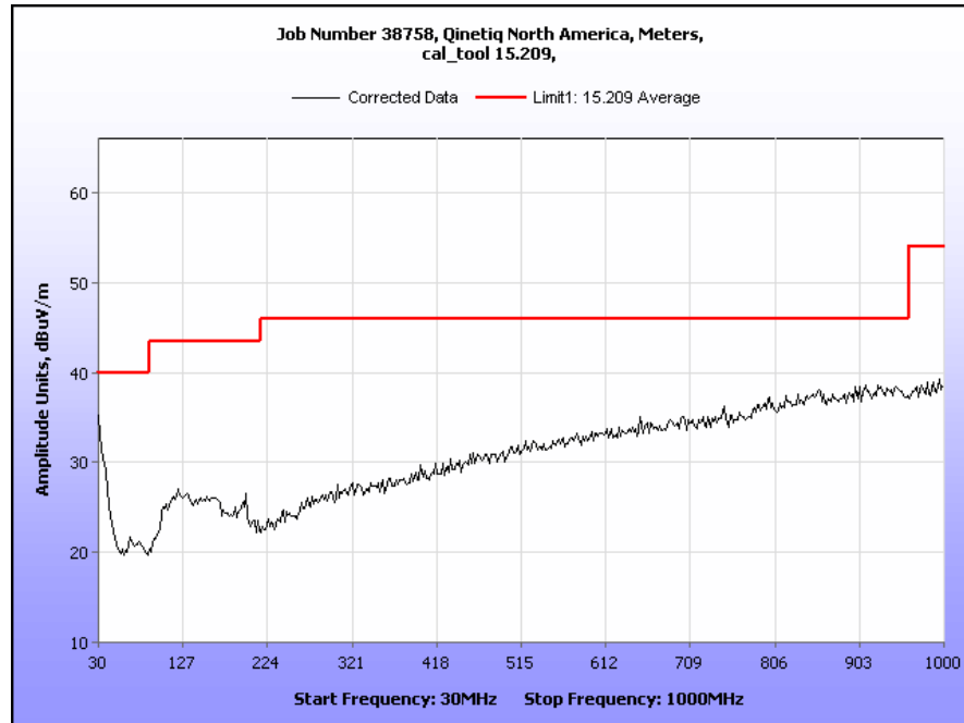
Plot 14. Radiated Spurious Emissions, 2465 MHz, 30 MHz – 1 GHz
