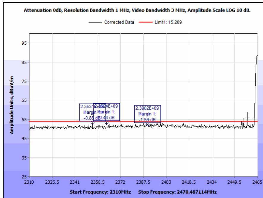
Plot 23. Restricted Band, 2471 MHz, Peak under Average
