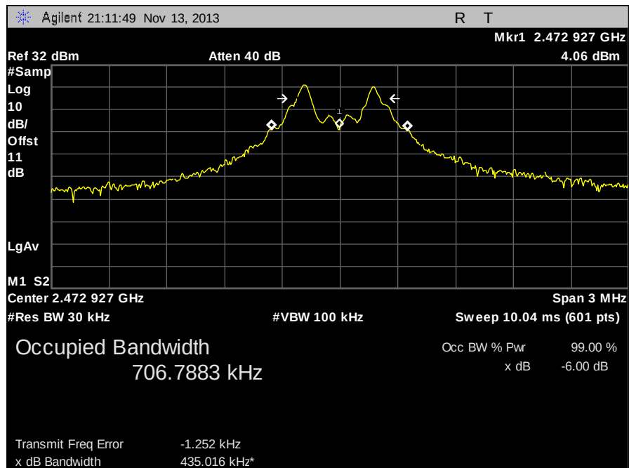
Plot 12. 99% Occupied Bandwidth, 2473 MHz
