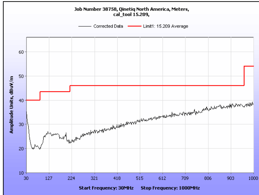
Plot 18. Radiated Spurious Emissions, 2473 MHz, 30 MHz – 1 GHz
