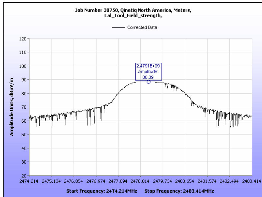
Plot 5. Radiated Field Strength of Fundamental, 2479 MHz
