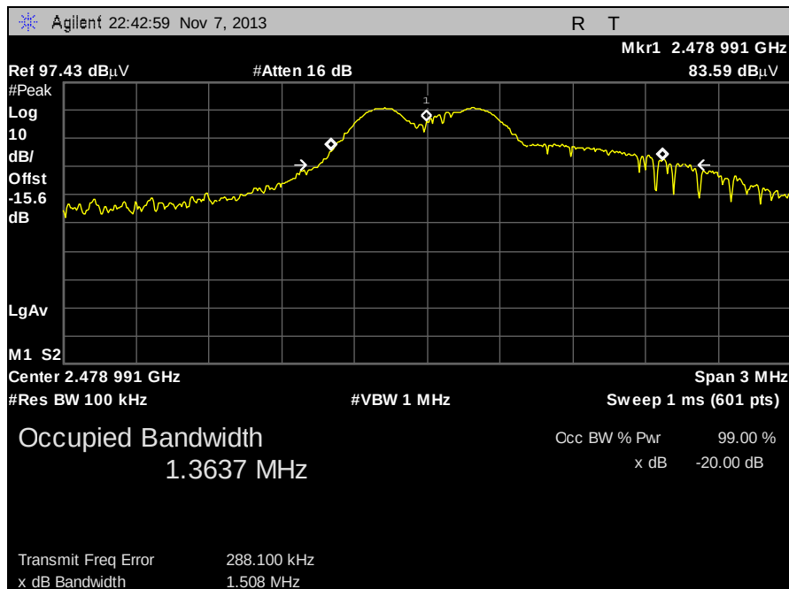
Plot 9. 20 dB Occupied Bandwidth, 2479 MHz
