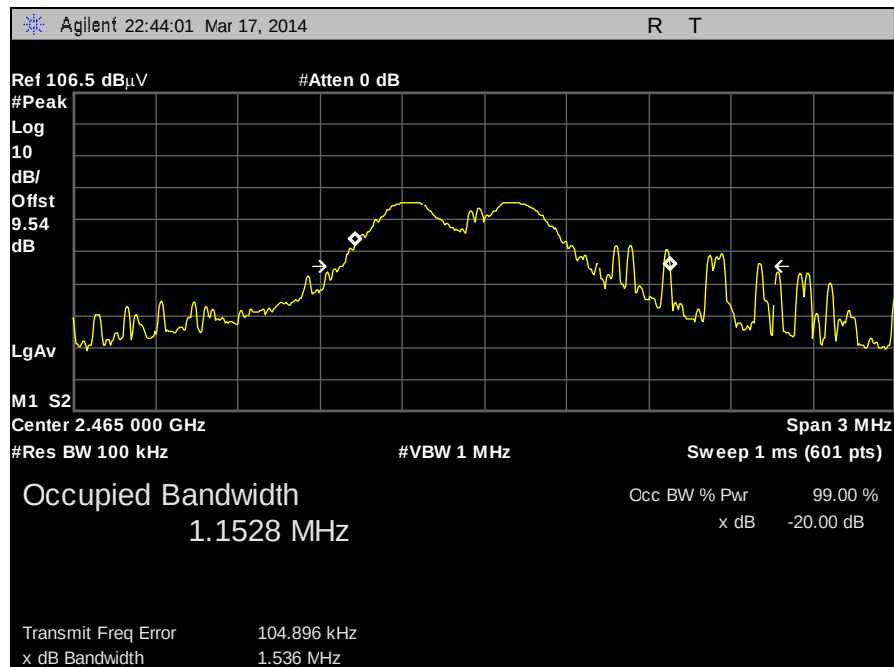
Plot 6. 20 dB Occupied Bandwidth, 2465 MHz
