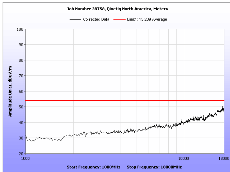
Plot 21. Radiated Spurious Emissions, 2479 MHz, Peak under Average, 1 GHz – 18 GHz
