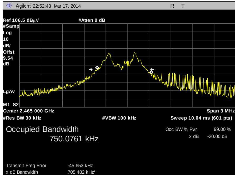
Plot 10. 99% Occupied Bandwidth, 2465 MHz
