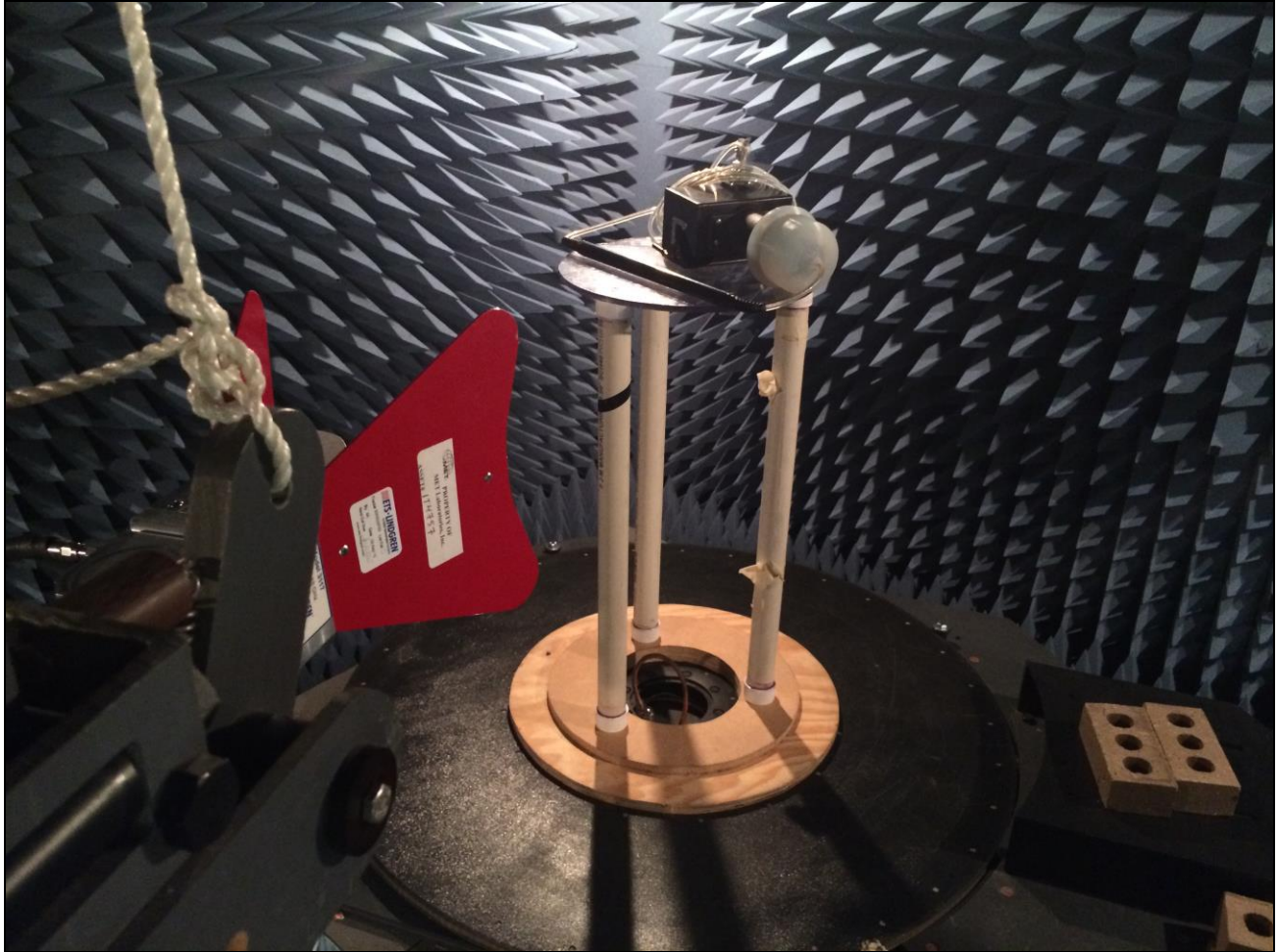
Photograph 2. Radiated Field Strength, Test Setup
