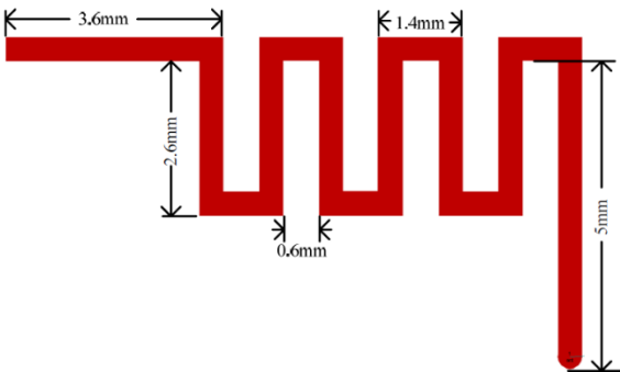
Antenna Photo & Length (mm)
