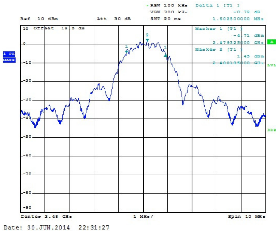
Figure 7.2.2-3: 6dB BW - High Channel
